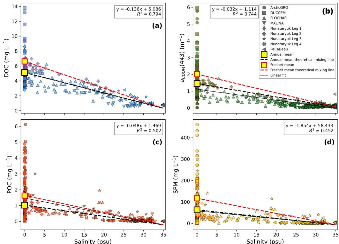
Figure 4. Linear regressions between salinity (psu) and (a) DOC, (b) a_{CDOM(443)} , (c) POC and (d) SPM across the fluvial marine salinity gradient from all campaign data from 2009-2024. The solid black lines represent the linear fit. The linear regression analysis filtered observations for salinity >0.2 psu for all four parameters to exclude the large seasonal variation of the river water. The yellow box outlined in black represents the annual mean for observations \leq 0.2 psu and the black dashed line represents the annual mean theoretical mixing line. The yellow box outlined in red represents the freshet mean for observations \leq 0.2 psu while the red dashed line represents the spring freshet theoretical mixing line (for months May-June, as described in Holmes et al., 2012). Observations outlined in red represent samples from May and June. Equations and coefficients of determination ( r^2 ) are shown for each plot.
