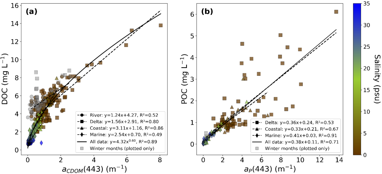
Figure 6. Bio-optical relationships for measured in-situ (a) DOC and a_{CDOM}(443) and (b) POC and a_P(443) along the freshwater-marine salinity gradient during 2009-2024. The black solid line shows the regression of all samples (Massicotte et al., 2021; Lizotte et al., 2023; Bröder et al., 2022; this study; mackenzie-monitoring.awi.de) across all compartments. The dashed black lines show the relationship per compartment. Observations in grey are plotted but are not included in the statistical analysis.
