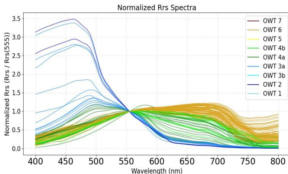
Fig. A4. In-situ remote sensing reflectance ( R_{rs} ) observations normalized to R_{rs}(555) nm from MALINA, Nunataryuk, PeCaBeau, and FLOCHAR sampling campaigns. This figure shows that the OWT classification applied in this study can distinguish R_{rs} spectra very well.
