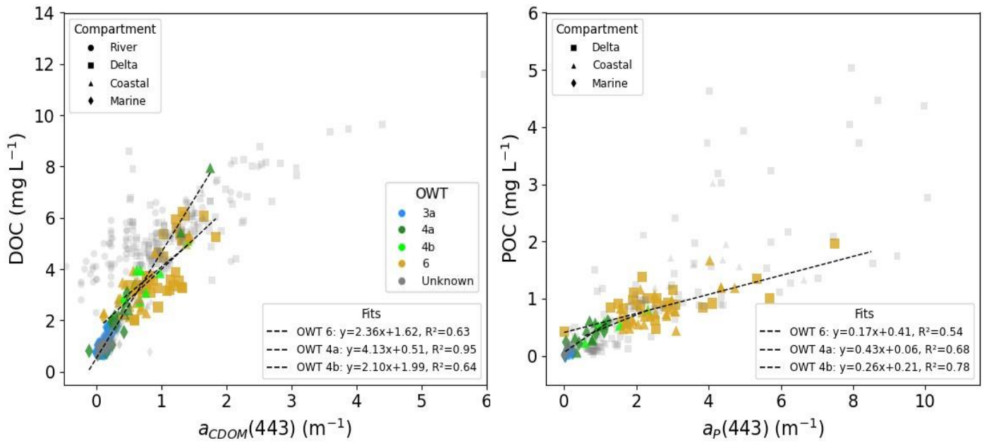
Fig. A3. Bio-optical relationships for measured in-situ DOC and a_{CDOM}(443) and POC and a_P(443) by OWT. The dashed black lines show the relationship for samples with dominant OWT maximum memberships (OWT 4a, 4b, 6). (OWT 6: DOC- a_{CDOM} : n=72 ; POC- a_P : n=57 ) (Massicotte et al., 2021, Lizotte et al., 2023, Bröder et al., 2022, this study, mackenziemonitoring.awi.de).
