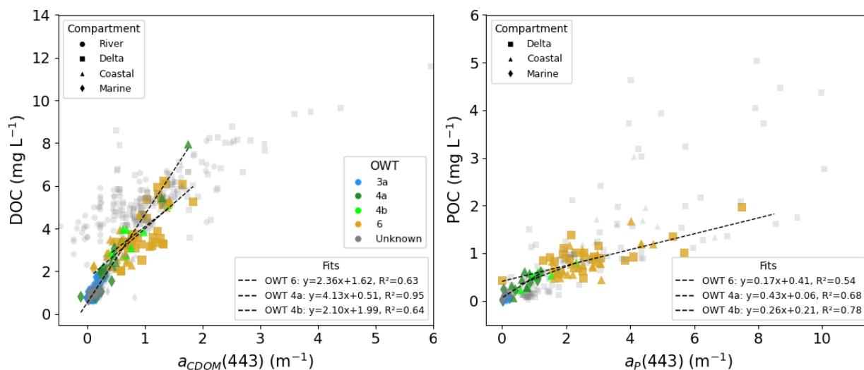
Fig. A3. Bio-optical relationships for measured in-situ DOC and a_{CDOM}(443) and POC and a_P(443) by OWT. The dashed black lines show the relationship for samples with dominant OWT maximum memberships (OWT 4a, 4b, 6). (OWT 6: DOC- a_{CDOM} : n=72; POC- a_P : n=57) (Massicotte et al., 2021, Lizotte et al., 2023, Bröder et al., 2022, this study, mackenzie-monitoring.awi.de).
