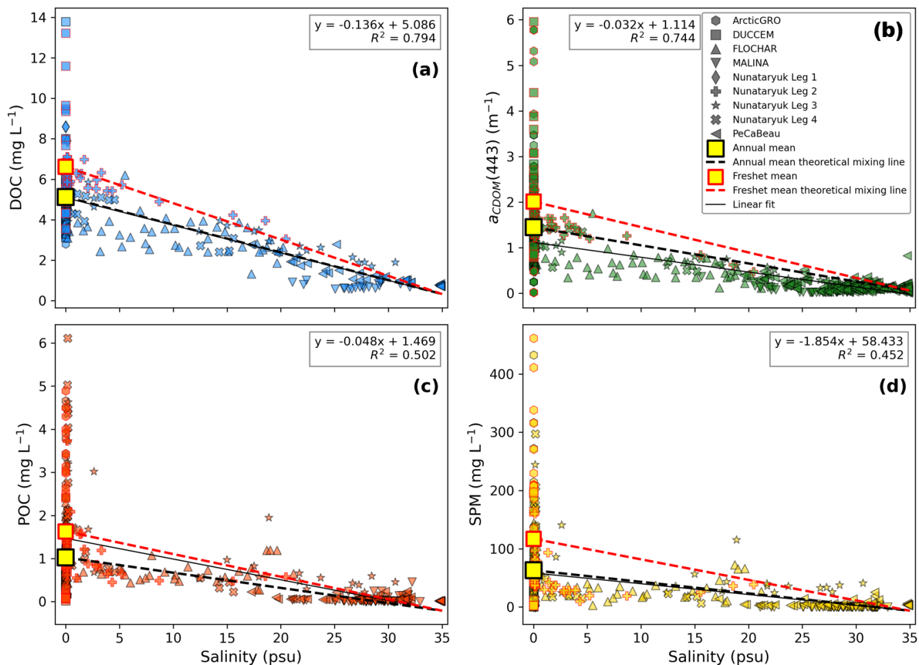
Figure 4. Linear regressions between salinity (psu) and (a) DOC, (b) a_{CDOM}(443) , (c) POC and (d) SPM across the fluvial-marine salinity gradient from all campaign data from 2009-2024. The solid black lines represent the linear fit. The linear regression analysis filtered observations for salinity >0.2 psu for all four parameters to exclude the large seasonal variation of the river water. The yellow box outlined in black represents the annual mean for observations \leq 0.2 psu and the black dashed line represents the annual mean theoretical mixing line. The yellow box outlined in red represents the freshet mean for observations \leq 0.2 psu while the red dashed line represents the spring freshet theoretical mixing line (for months May-June, as described in Holmes et al., 2012). Observations outlined in red represent samples from May and June. Equations and coefficients of determination ( r^2 ) are shown for each plot.
