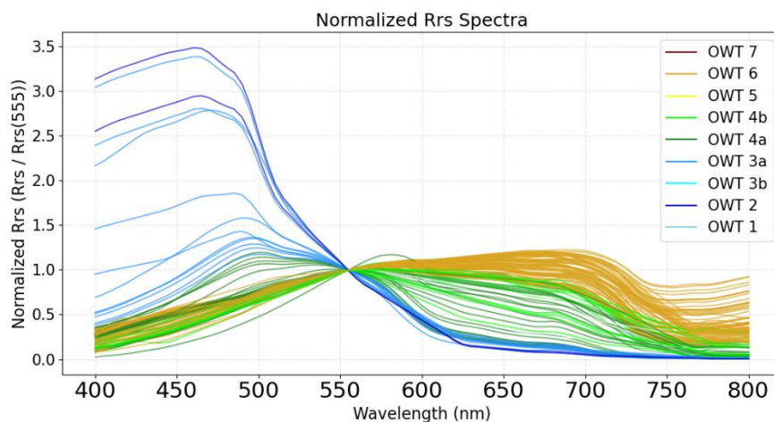
Fig. A4. In situ remote sensing reflectance ( R_{rs} ) observations normalized to R_{rs}(555) nm from MALINA, Nunataryuk, PeCaBeau, and FLOCHAR sampling campaigns. This figure shows that the OWT classification applied in this study can distinguish R_{rs} spectra very well.
