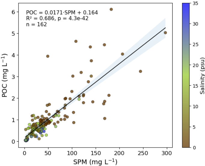
Fig. A1. Relationship between suspended particulate matter (SPM) and particulate organic carbon (POC). POC concentrations increase significantly with SPM, indicating a strong positive association between particle load and organic carbon content. Point color denotes salinity (psu). The solid line represents the linear regression, and the shaded band indicates the 95% 645 confidence interval.
