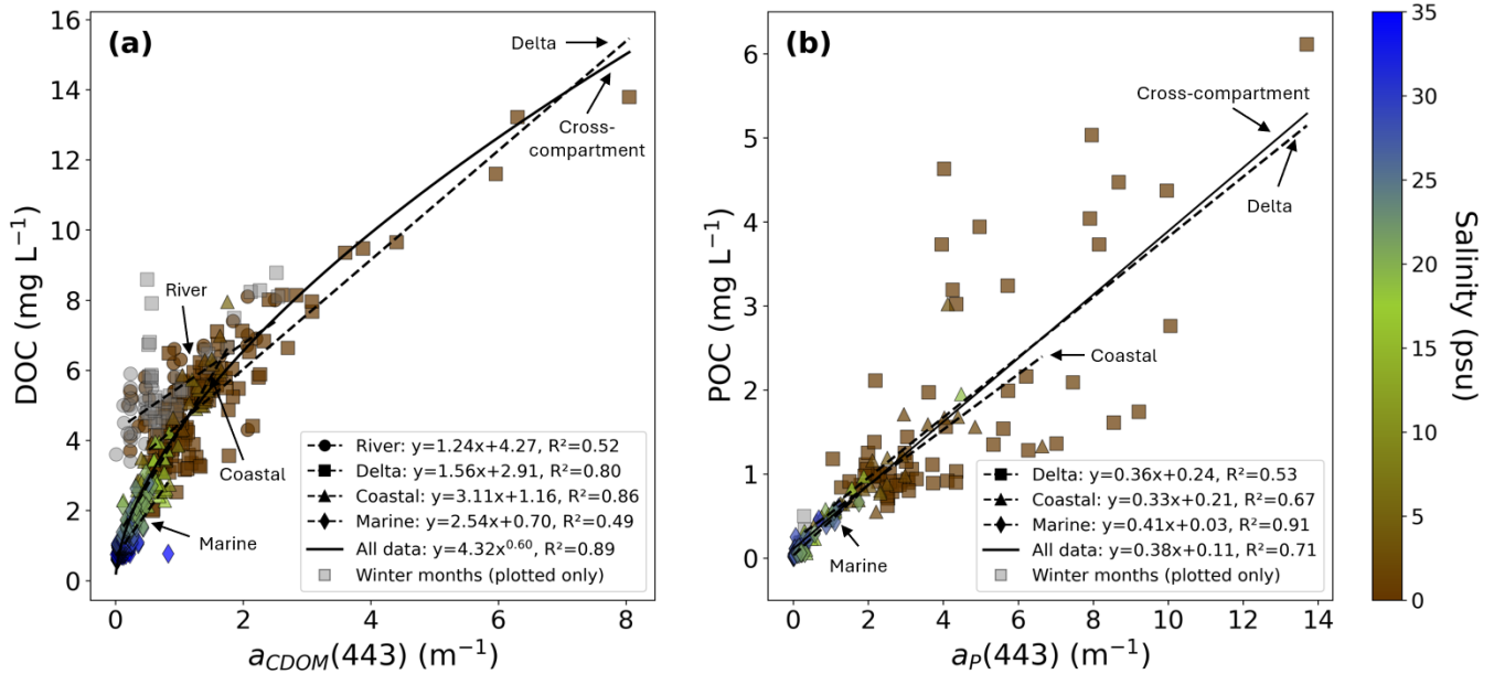
430 Figure 6. Bio-optical relationships for measured in-situ (a) DOC and a_{CDOM}(443) and (b) POC and a_P(443) along the freshwater-marine salinity gradient during 2009-2024. The black solid line shows the regression of all samples (Massicotte et al., 2021; Lizotte et al., 2023; Bröder et al., 2022; this study; mackenzie-monitoring.awi.de) across all compartments. The dashed black lines show the relationship per compartment. Observations in grey are plotted but are not included in the statistical analysis.
