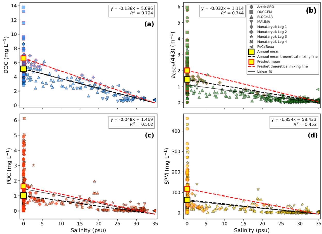
Figure 4. Linear regressions between salinity and (a) DOC, (b) a_{CDOM}(443) , (c) POC and (d) SPM across the fluvial-marine salinity gradient from all campaign data from 2009-2024. The solid black lines represent the linear fit. The linear regression analysis filtered observations for salinity >0.2 psu for all four parameters to exclude the large seasonal variation of the river water. The yellow box outlined in black represents the annual mean for observations \leq 0.2 psu and the black dashed line represents the annual mean theoretical mixing line. The yellow box outlined in red represents the freshet mean for observations \leq 0.2 psu while the red dashed line represents the spring freshet theoretical mixing line (for months May-June, as described in Holmes et al., 2012). Observations outlined in red represent samples from May and June. Equations and coefficients of determination ( r^2 ) are shown for each plot.
