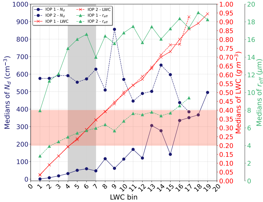
Figure 15. Medians of N_d , r_{eff} and LWC according to LWC bins for both IOP.
