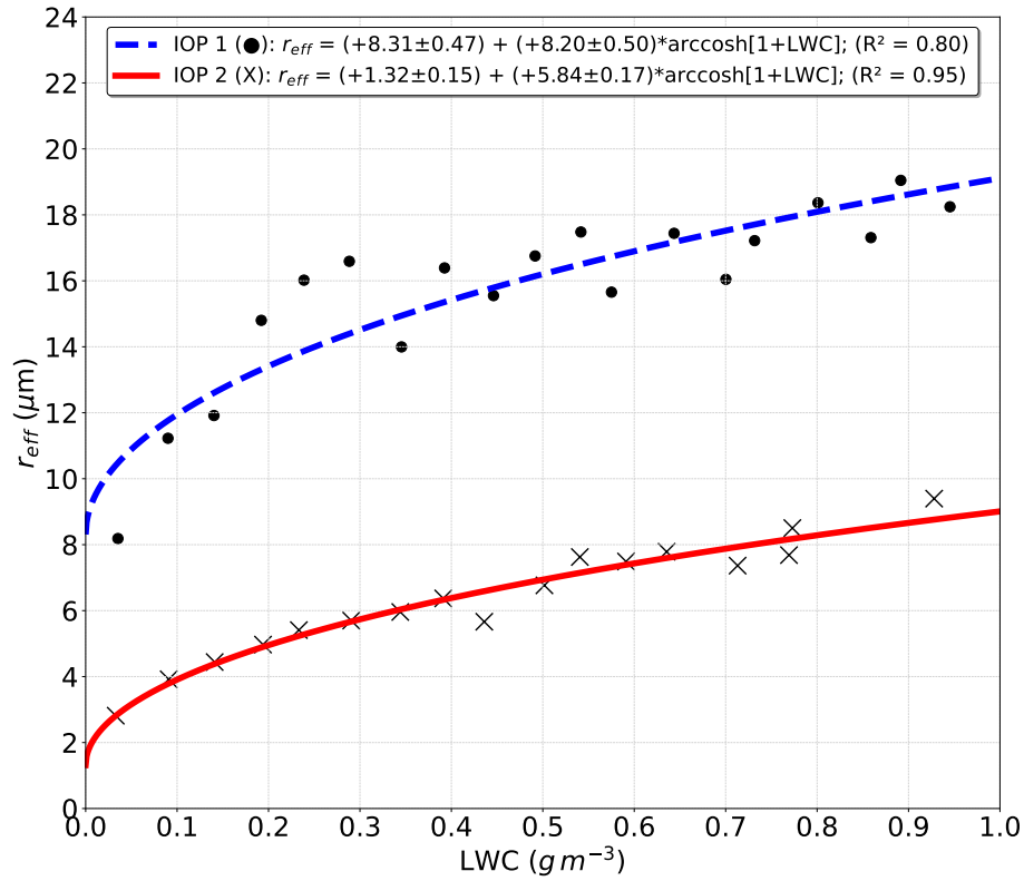
Figure 3. Dispersion of medians of r_{eff} . and LWC calculated in the 20 bins for IOP 1 and 2. The medians included experimental points from all altitudes where clouds with liquid water were identified and for which N_d \geq 0.3 particles cm^{-3} and LWC \geq 0.02 g m^{-3} . Although no filter was applied to distinguish between cumuliform and stratiform clouds, these clouds were selected using these same filters in both IOP. The adjustments (hyperbolic arc cosine function) originated the equations shown in the graph's legend.
