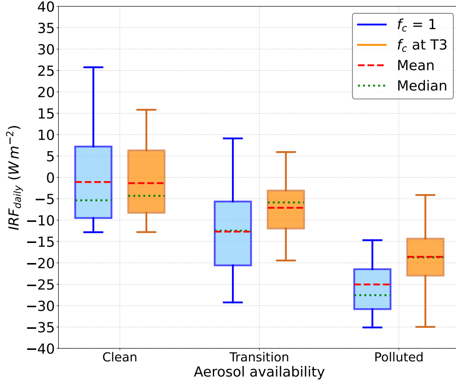
Figure 7. Boxplots, means and medians of IRF_{daily} calculated according to the first clean atmosphere reference for 2015 and separated according to the aerosol availability at T3.
