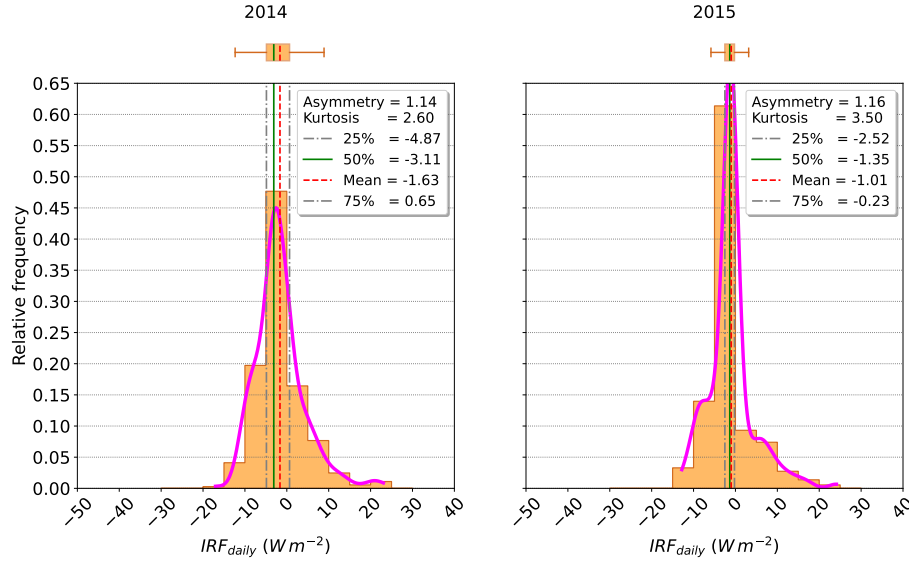
Figure 14. Boxplots and histograms of IRF_{daily} for 2014 and 2015 for f_c = \pm 100\% measured at T3, according to the second reference for a clean atmosphere.
