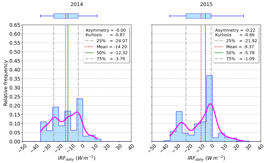
Figure 8. Boxplots and histograms of IRF_{daily} for 2014 (left) and 2015 (right) for f_c = \pm 100\% .
