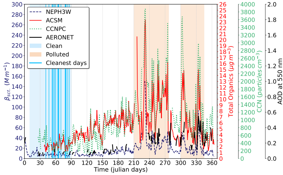
Figure 1. Daily averages of \beta_{sct.} , Org. and CCN for 2014. The legend indicates the instruments responsible for data acquisition and the days that demilit the clean and polluted scenarios. The identification of cleanest days within the clean scenario was carried out using a clustering technique described in Sect. 2.4.
