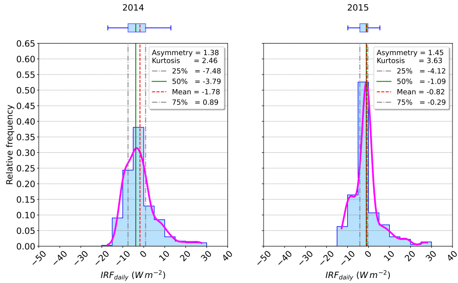
Figure 13. Boxplots and histograms of IRF_{daily} for 2014 and 2015 for f_c = \pm 100\% according to the second reference for a clean atmosphere.
