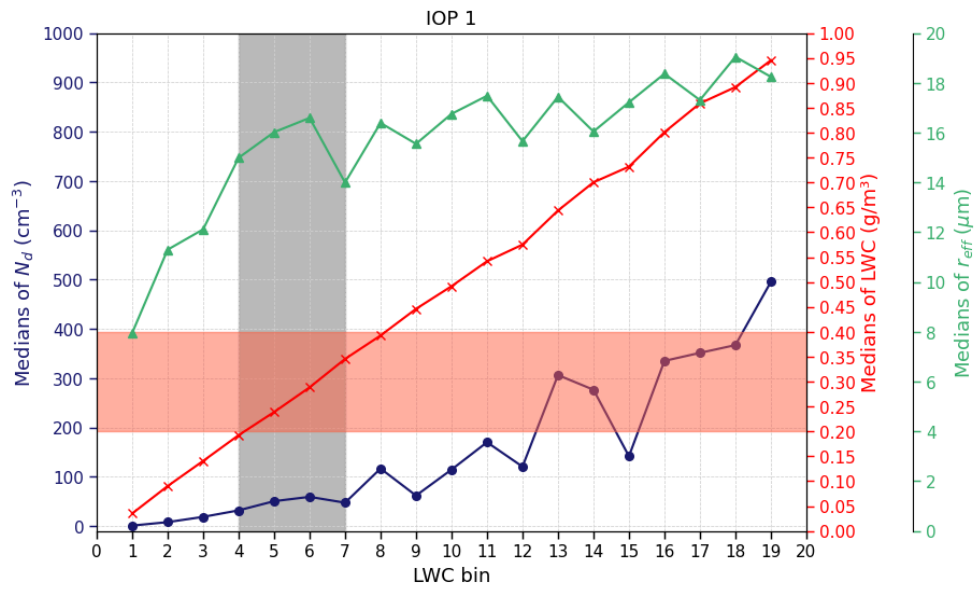
Figure 1: Median's variations ( N_d , LWC e r_{eff} ) along LWC bins for IOP1. Bins 4 to 7 correspond to the LWC range ( 0.2 to 0.4 \text{ g/m}^3 ) considered for filtering the clouds analyzed in the study.
