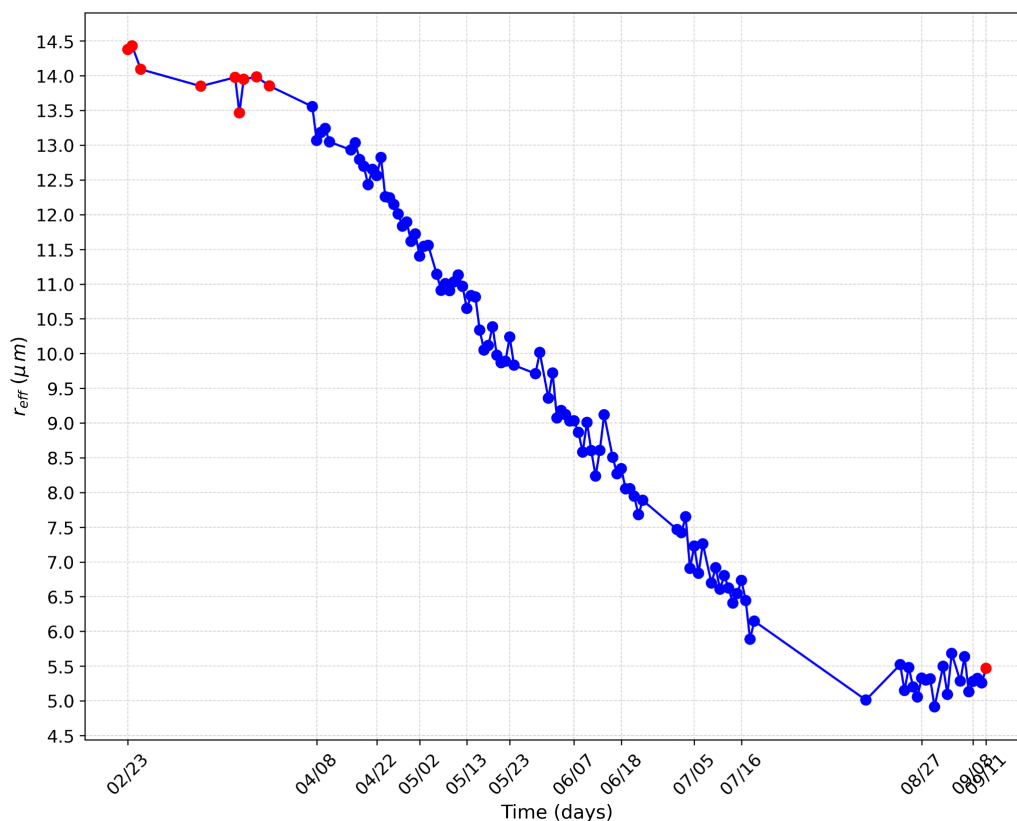
Figure 7: Diurnal medians of r_{eff} during 2014. The cleanest days within the clean and polluted seasons are represented by the red dots, while the bluish dots correspond to the transition days.
