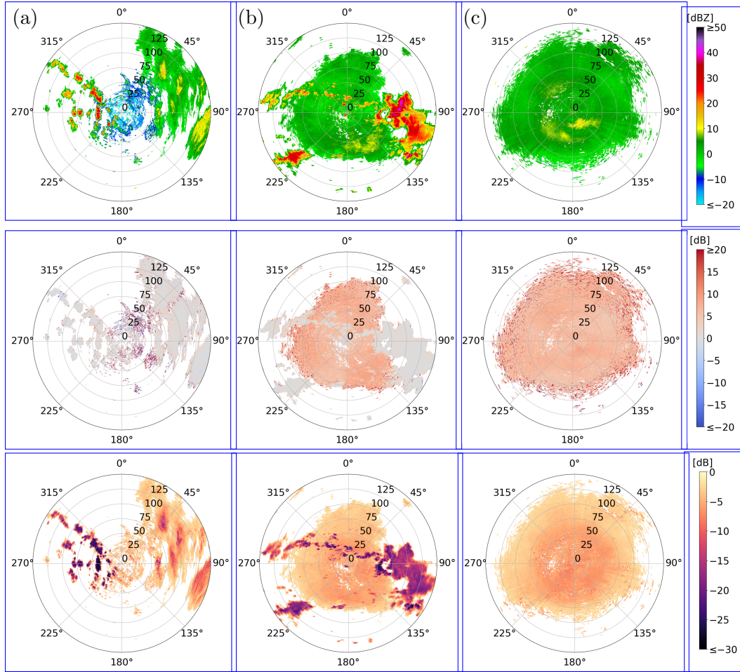
Figure 1: Horizontal reflectivity (first row), differential reflectivity (second row), and depolarization ratio (third row) for examples of (a) a winter sweep, (b) a mixed summer sweep, and (c) a cluttered summer sweep. White pixels are filtered by the initial preprocessing done by DWD. The sweeps shown were measured (a) on January 9, 2025, at 17:55 UTC in Flechtdorf, (b) on June 16, 2022, at 09:00 UTC in Dresden and (c) on June 18, 2022, at 10:00 UTC in Isen.
