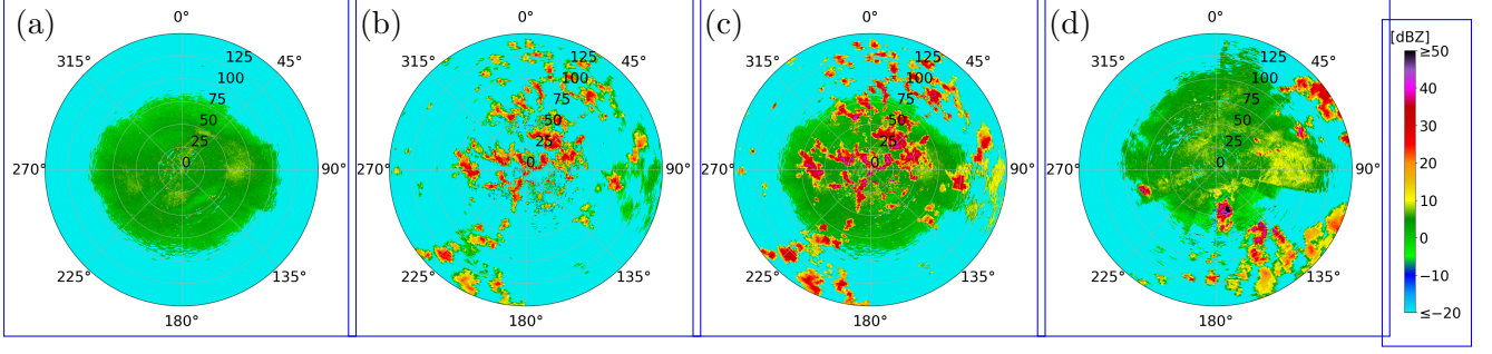
Figure 5: Comparison of Cartesian representations of different DBZH images: (a) cluttered summer radar image, (b) winter radar image, (c) their corresponding synthetic radar image with weighting factors \lambda_w = 6.5 , and \lambda_s = 1 and (d) mixed summer radar image. The radar images shown were measured (a) on June 18, 2022, at 10:00 UTC in Neuheilenbach, (b) on January 9, 2025, at 17:00 UTC in Borkum and (d) on June 16, 2022, at 09:55 UTC in Memmingen.
