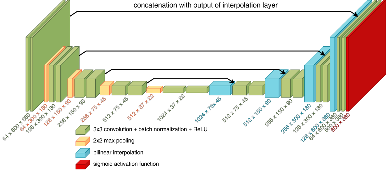
Figure 4: Schematic representation of the network architecture with n_f = 64 feature channels in the first downsampling step . Below each layer, the respective output dimensions are given.
