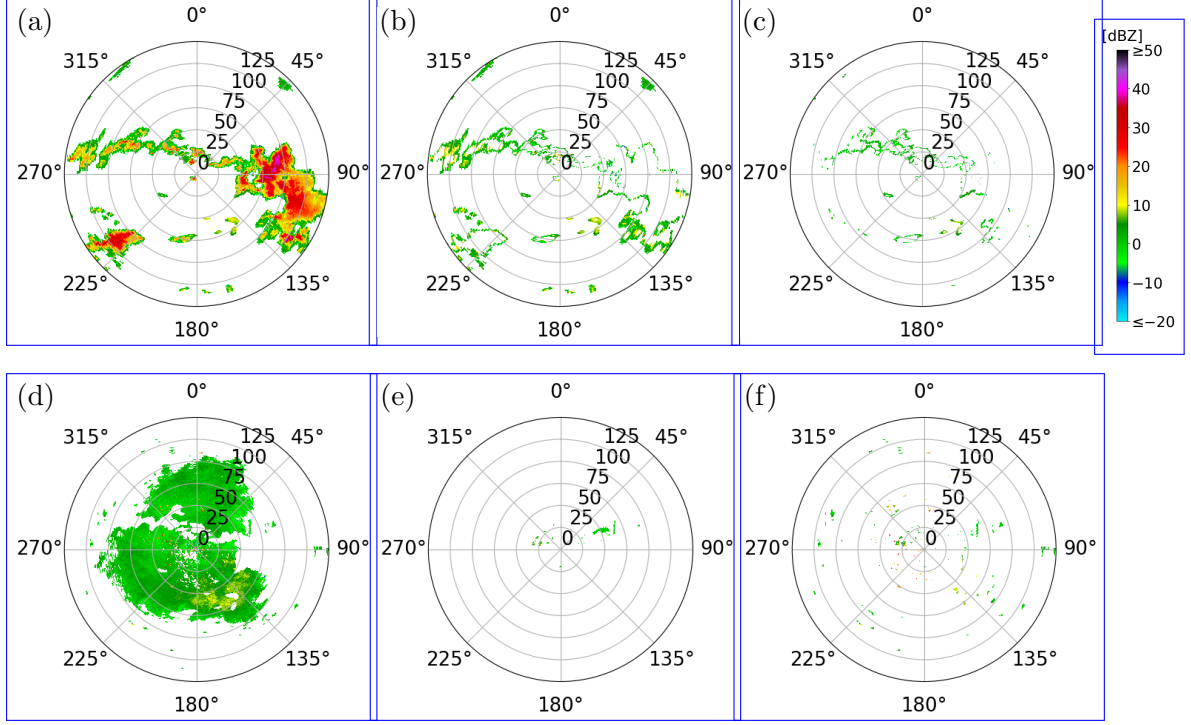
Figure 11: Evaluation of the SotA method and the trained network on the experimentally measured radar image shown in Fig. 1b: The first row shows (a) the ground truth for the meteorological echoes and the meteorological echoes misclassified as non-meteorological echoes by (b) the SotA method and (c) the trained network. Analogously, the second row shows (d) the hand-labeled ground truth for the non-meteorological echoes and the non-meteorological echoes misclassified as meteorological echoes by (e) the SotA method and (f) the trained network.
