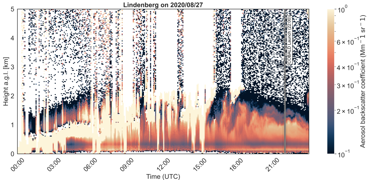
Figure 3. Temporal evolution of forward retrieval aerosol backscatter coefficient ( Mm^{-1}sr^{-1} ) from the ceilometer at Lindenberg for 27 August 2020. COBALD launch time is shown as a black line.
