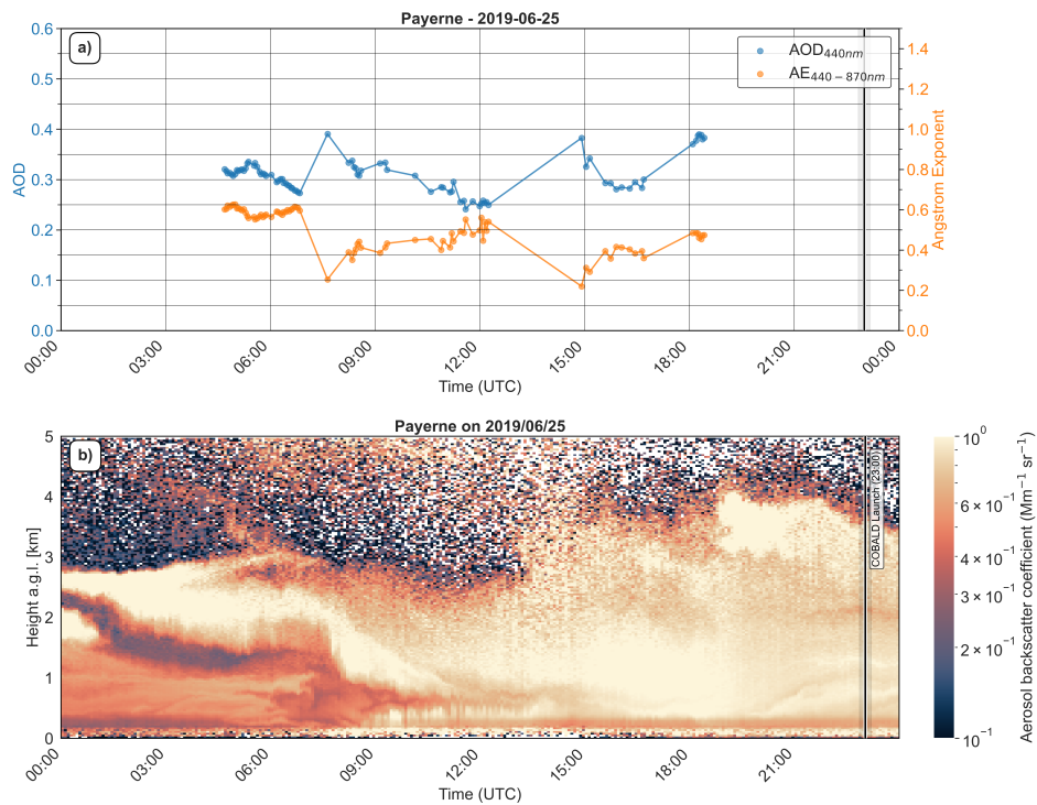
Figure 1. Characterization of the dust outbreak event over Payerne. a) AOD (440 nm) and Ångström exponent (440-870 nm); b) ceilometer aerosol backscatter coefficient with forward retrieval, COBALD launch time is marked as a shaded black band
