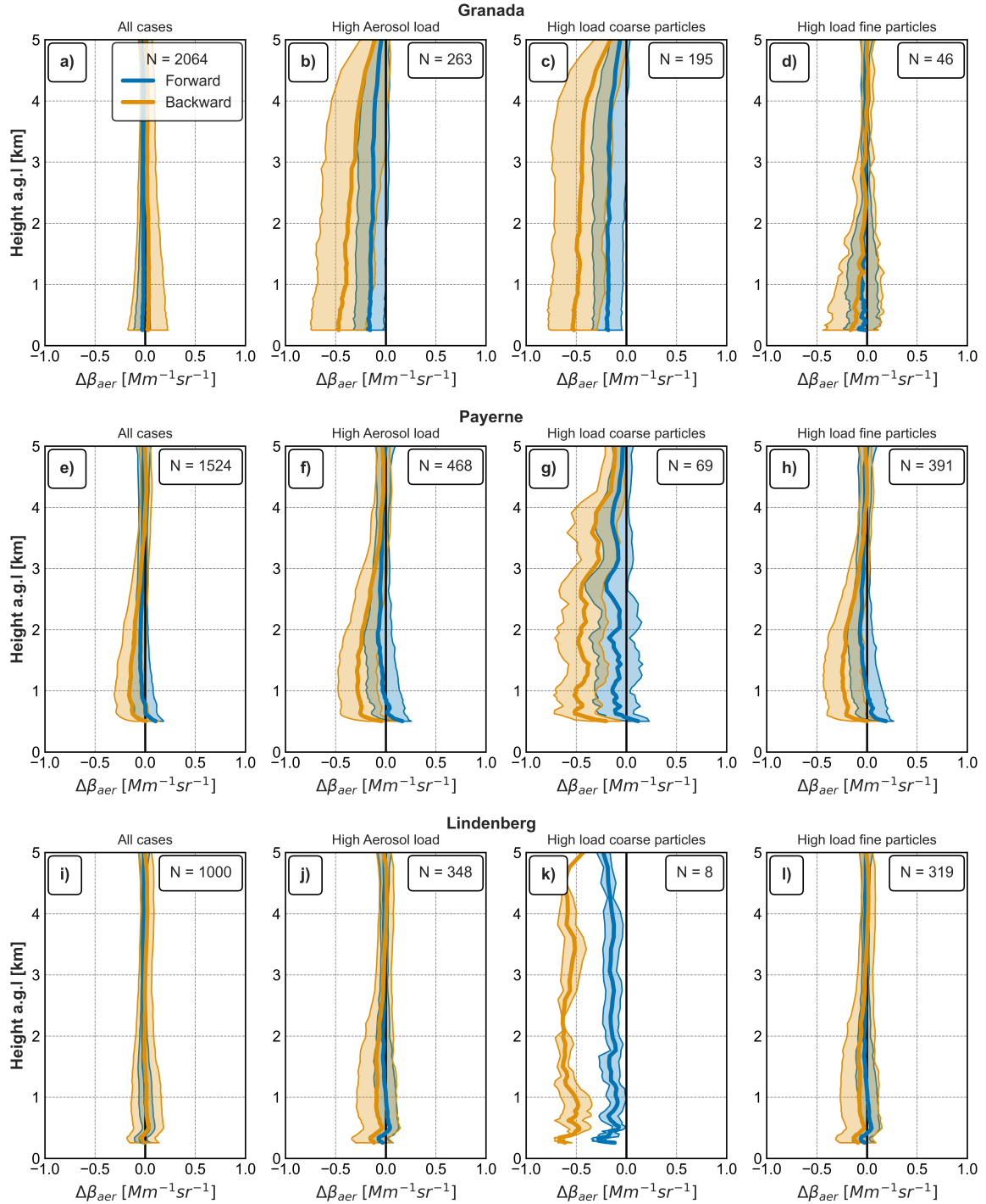
Figure 5. Tropospheric backscatter coefficient profiles comparison: Klett-Fernald backward retrievals versus GRASP pac for Granada (top), Payerne (middle) and Lindenberg (bottom) with the full dataset (a, e, i), high aerosol load (b, f, j), coarse dominated particles (c, g, k), fine dominated particles (d, h, l) aerosol conditions and N shows number of profiles in each panel
