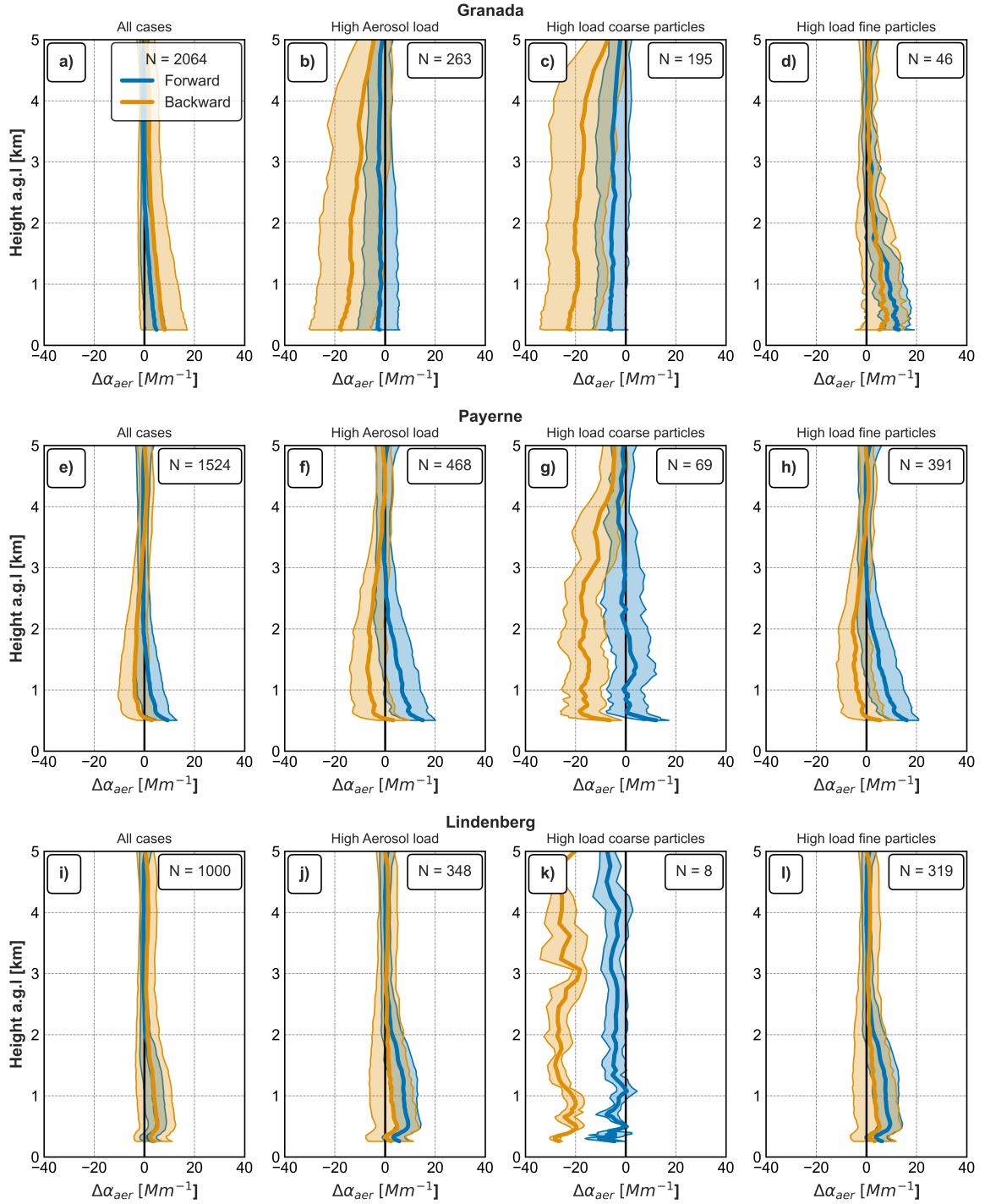
Figure 6. Tropospheric extinction profiles comparison: differences between Klett-Fernald backward retrieval - GRASP pac for Granada (top), Payerne (middle) and Lindenberg (bottom) with the full dataset (a, e, i), high aerosol load (b, f, j), coarse dominated particles (c, g, k), fine dominated particles (d, h, l) aerosol conditions and N shows the number of profiles in each panel.
