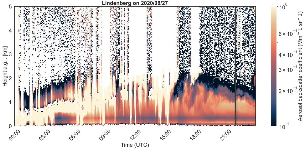
Figure 3. Temporal evolution of forward retrieval aerosol backscatter coefficient from the ceilometer for the day 27 August 2020. COBALD launch time is marked as a shaded black band
