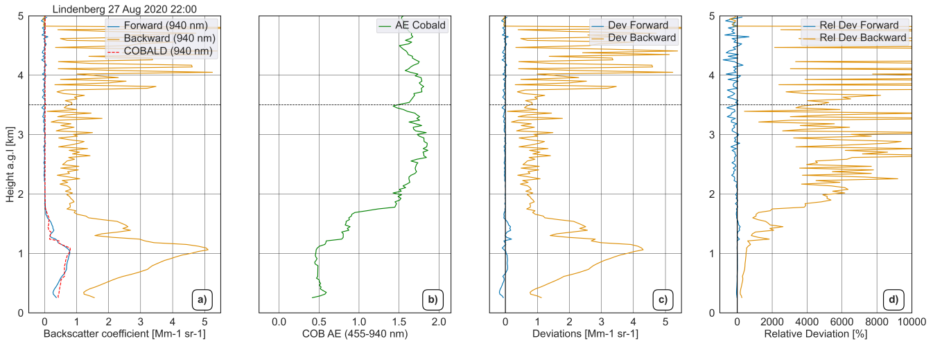
Figure 4. 30 min averaged profile comparison between forward/backward retrievals versus COBALD sonde for 27 August 2020. Panel a show the backward (yellow) forward (blue) and COBALD (red) profile, next panel (b) show the Ångström exponent profile of COBALD and the following panels (c and d) show the deviation and relative deviation of Backward-COBALD (yellow) and Forward-COBALD (blue)
