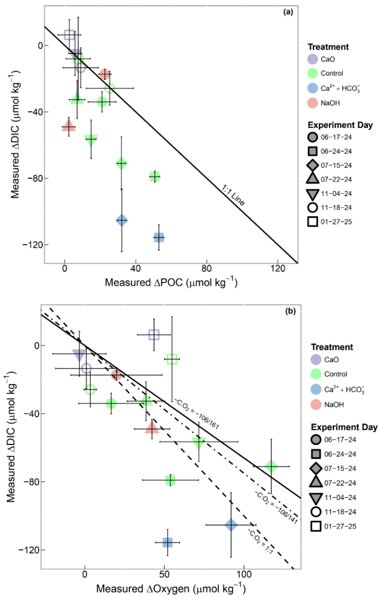
Figure 8. Comparison of stoichiometric changes in DIC, Dissolved O 2 , and POC in terms of the Redfield Ratio. (a) Cross plot of measured decrease of DIC versus the measured increase of POC; solid
