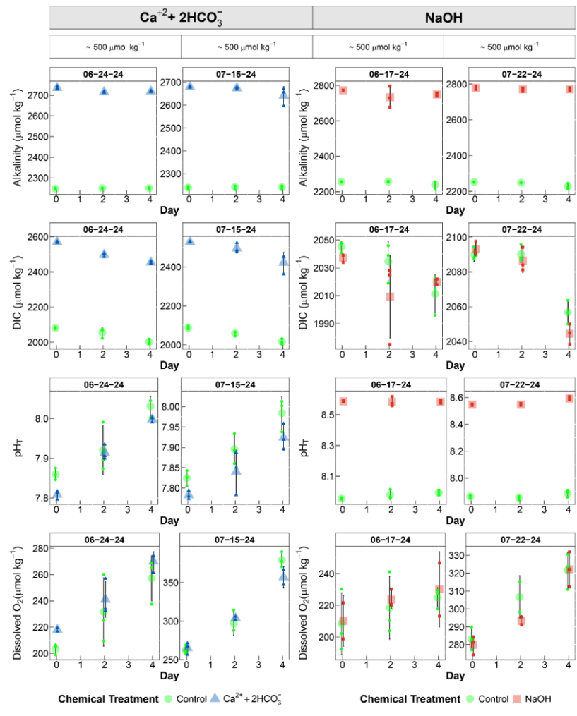
Figure 2. Water Chemistry from (NaOH and [\text{Ca}^{2+}] + [\text{HCO}_3^-] -addition) aAmendment eExperiments. Panels are grouped by the alkalinity treatment they received: Controls (green), NaOH (red) and \text{CaCl}_2 + \text{NaHCO}_3 (blue). The start date of the experiment is listed for reference to differentiate between duplicate experiments. The four variables displayed here are measured Alkalinity ( \mu\text{mol kg}^{-1} ), measured Dissolved Inorganic Carbon (DIC, \mu\text{mol kg}^{-1} ), \text{pH}_T (Total Scale) calculated from CO2Sys.v3, and Dissolved Oxygen ( \text{O}_2 , \mu\text{mol kg}^{-1} ). Each plot shows the average of the treatment per timepoint (n =
