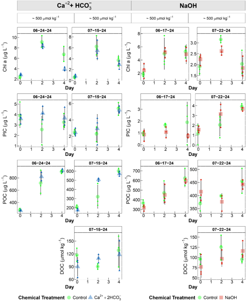
412 413 Figure 3. Four dDay tTimeseries of bBiogeochemical rResponse to dDifferent aAlkalinity 414 eEnhancements. Smaller symbols show individual bottles; larger symbols show the mean. Error bars are 415 the standard deviation between replicates ( n = 3 ). The start date of the experiment and the amount of 416 alkalinity added are included as headers for reference. The variables displayed are Chlorophyll a (Chl
