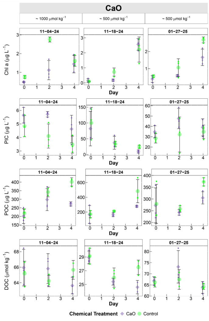
476 477 Figure 5. Four dDay tTimeseries of bBiogeochemical rResponse to dDifferent aAlkalinity 478 eEnhancements. Smaller symbols show individual bottles, large symbol shows mean. Error bars are the 479 standard deviation between replicates (n = 3). The start date of the experiment and the amount of 480 alkalinity added are included as headers for reference. The variables displayed are Chlorophyll a (Chl a, 481 \mu\text{g L}^{-1} ), Particulate Inorganic Carbon (PIC, \mu\text{g L}^{-1} ), Particulate Organic Carbon (POC, \mu\text{g L}^{-1} ), and 482 Dissolved Organic Carbon (DOC, \mu\text{mol kg}^{-1} ).
