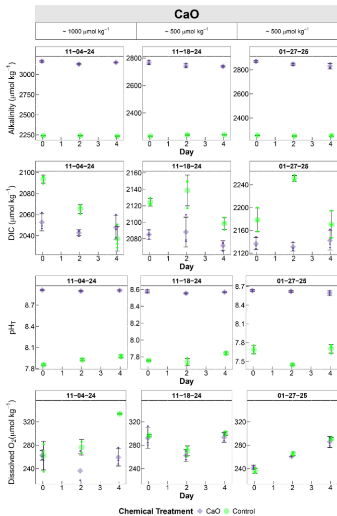
Figure 4. Water Chemistry from (CaO) aAmendment cExperiments. Panels are grouped by the alkalinity treatment they received: Controls (green) and CaO (purple). The start date of the experiment is listed for reference to differentiate between duplicate experiments. The four variables displayed here are measured Alkalinity ( \mu\text{mol kg}^{-1} ), measured Dissolved Inorganic Carbon (DIC, \mu\text{mol kg}^{-1} ), \text{pH}_T (Total Scale) calculated from CO2Sys.v3, and Dissolved Oxygen ( \text{O}_2 , \mu\text{mol kg}^{-1} ). Each plot shows the average of the treatment per timepoint ( n = 3 ), and the error bars are the standard deviation between the triplicate bottles. Smaller symbols show individual bottles.
