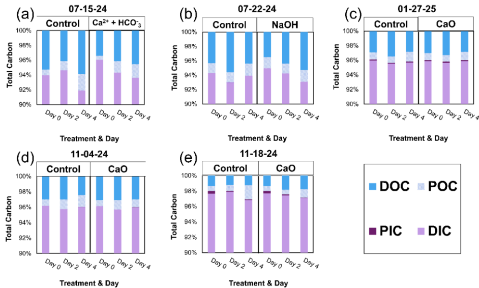
Figure 7. Total Carbon Budget for All Experiments. Panel (a) + 500 \mu\text{mol kg}^{-1} \text{CaCl}_2 + \text{NaHCO}_3 , (b) + 500 \mu\text{mol kg}^{-1} \text{NaOH} , (c) + 500 \mu\text{mol kg}^{-1} \text{CaO} , (d) + 1000 \mu\text{mol kg}^{-1} \text{CaO} , and (e) + 500 \mu\text{mol kg}^{-1} \text{CaO} with higher (ambient) particles of inorganic carbon. Bar plots are an average of 3 bottles per timepoint. Plots show changes in distribution of carbon over the duration of the experiment between treatments and controls. The total amount of C will always = 100%.
