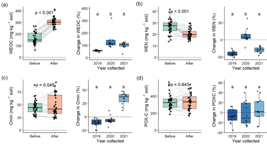
Figure 1: Soil storage increased WEOC (a) and Cmin (c), and decreased WEN (b) concentrations, while no significant change was observed for POX-C (d) concentrations, where the paired observations are shown represented by dotted lines, and p-values from paired t-tests are also shown. Percent change analysis revealed that POX-C concentrations were stable, while other indicators changed year-to-year, where years sharing the same lowercase letter are not significantly different (Tukey HSD, \alpha = 0.05 ).
