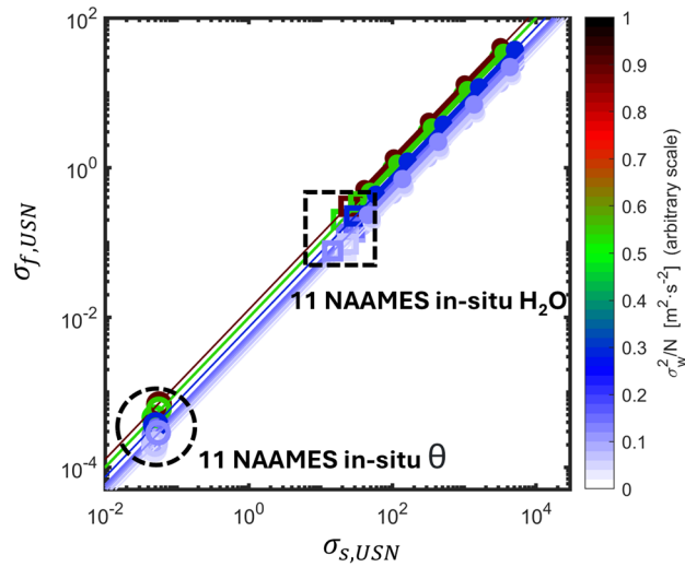
Figure 6. Impact of uncorrelated sensor noise on flux random errors. Results are shown for the noise perturbation ensemble described in-text (filled circles), for the uncontaminated NAAMES H_2O observations (squares), and for the NAAMES \theta observations (hollow circles). Each plotted value for the noise perturbation ensemble reflects the mean across all 500 members (standard deviations are smaller than the data points and thus not visible). See Fig. S4 for regression statistics.
