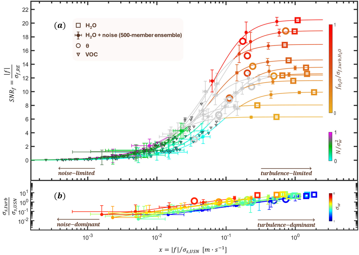
Figure 7. (a) Flux SNR ( SNR_f ) as a function of the flux:USN ratio. The curves visualize the SNR_f - x relationship based on Eq. (4) for the 11 ten analyzed flux legs, and are colored (arbitrary scale) to indicate noise-limited (bottom colorbar), transitional (grey), and turbulence-limited (top colorbar) regimes. Datapoints indicate the noise perturbation ensemble (filled circles; 500-member mean and standard deviation) along with the NAAMES H_2O (hollow squares), \theta (hollow circles), and VOC (triangles) observations. (b) Ratio of the turbulent- to USN-driven scalar concentration variability ( \frac{\sigma_{s,turb}}{\sigma_{s,USN}} ) as a function of the flux:USN ratio. Plotting conventions follow those of panel (a), with the noise perturbation ensemble represented by the 500-member median and interquartile range, and colors indicating the standard deviation of the vertical wind speed. \sigma_{s,USN} and \sigma_{s,turb} are derived from the variance partitioning analysis described in-text with negative values set to zero. Zero and negative values are omitted from the logarithmic scales. All fluxes employ traditional EC estimates with flight-specific lag times. Color bars use arbitrary scales.
