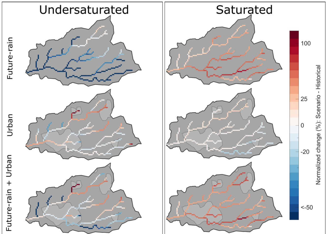
385 Figure 6 An example of the spatial intra-basin hydrological relative change of different scenarios compared to the Historical one for undersaturated event (left) and saturated event (right). Results show the relative change of peak discharges at each pixel for a single storm shift resulting in the outlet median peak discharge (bold line in Fig. 5). Light gray polygons in the lower two panels represent areas of major projected urbanization changes. Other, less significant land use variations (Fig. 1c), are not represented in this figure. Results for the future scenario are not shown as they are not significantly different from the 390 Future-rain + Urban scenario.
