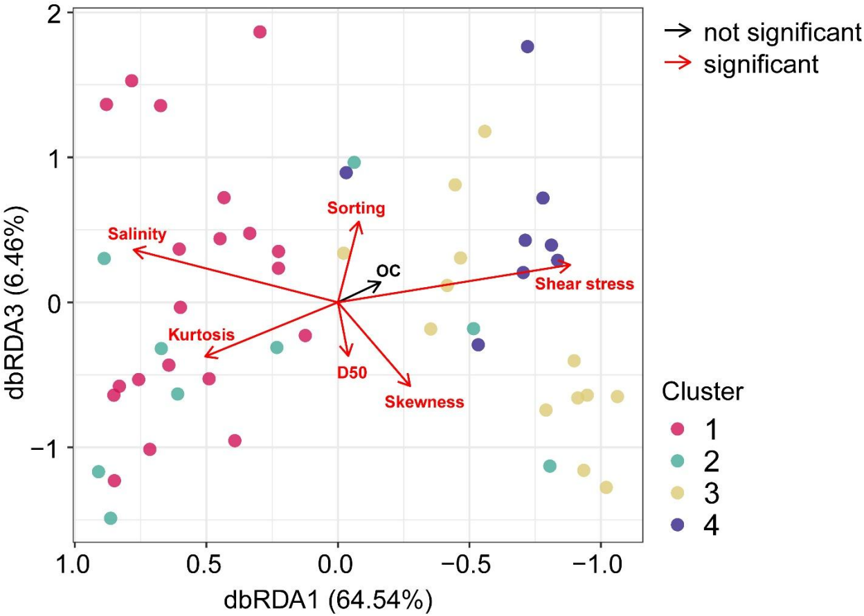
Figure 2: Distance-based redundancy analysis (dbRDA) of community ash-free dry mass. Note that axes 1 and 3 are shown with axis 1 reversed to reflect the spatial orientation of the sampling area.
