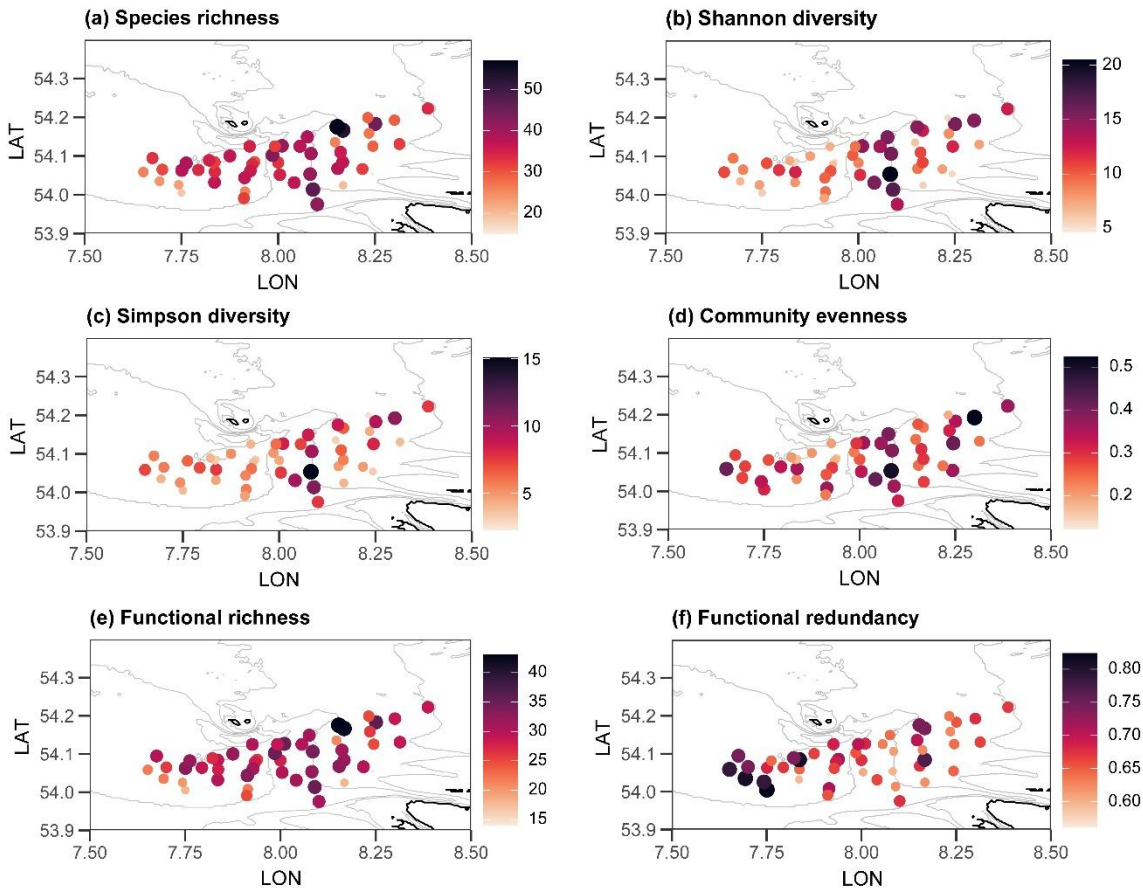
Figure 4: Calculated taxonomic and functional biodiversity indices for each station. The darker color and larger size of dot the symbols represent higher estimated values.
