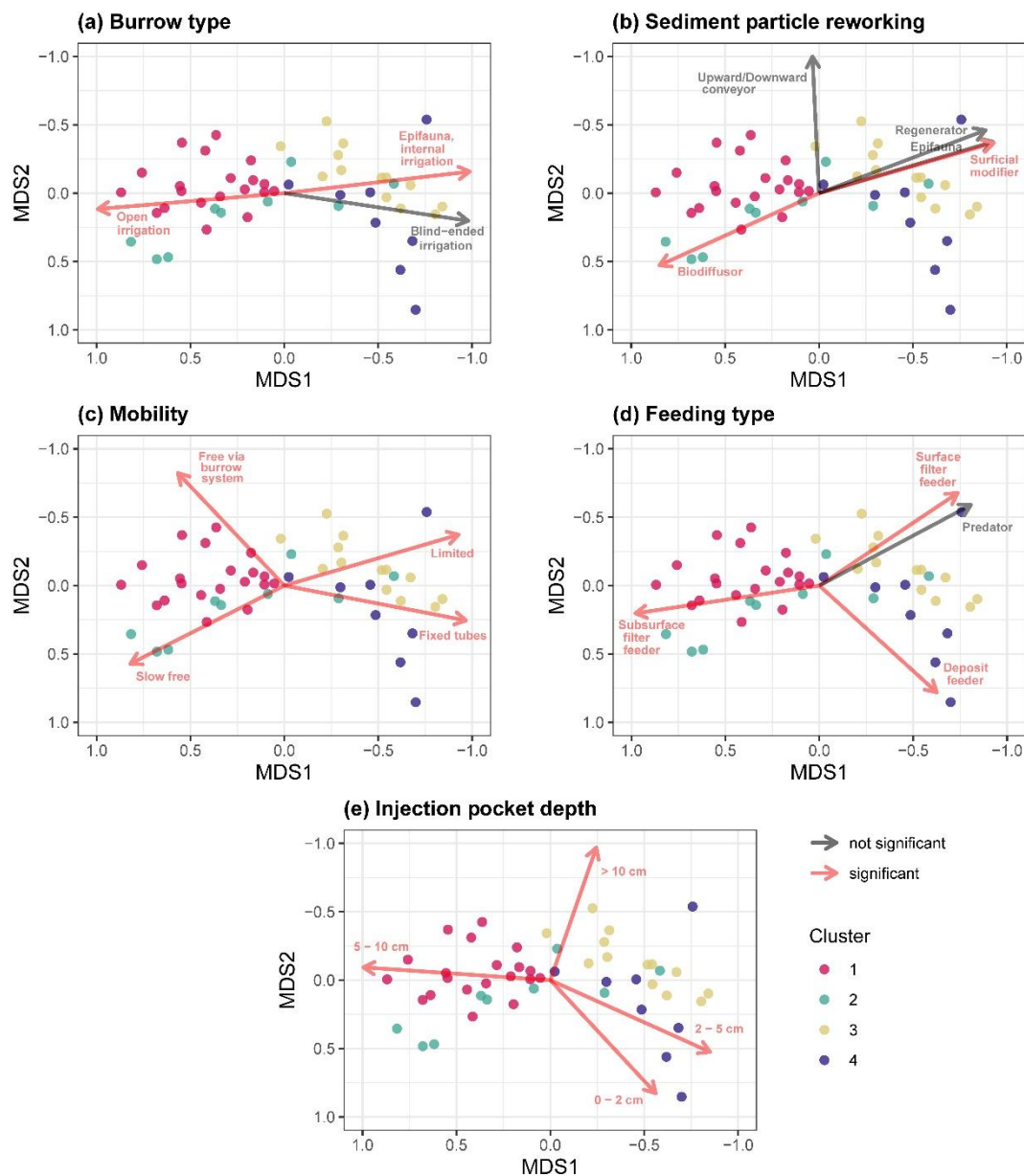
355 Figure 3: Non-metric multidimensional scaling (nMDS) ordination based on square-root transformed species ash-free dry mass. Functional traits (burrow type, sediment particle reworking mode, mobility, feeding type, and injection pocket depth) are projected as vectors according to their correlations with the ordination axes (stress = 0.14). Red arrows indicate traits with significant correlations.
