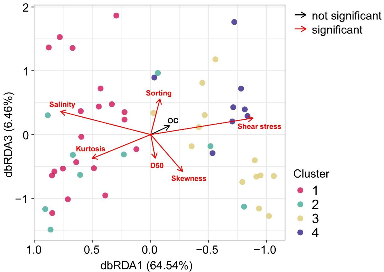
Figure 2: Distance-based redundancy analysis (dbRDA) of community ash-free dry mass. Note that axes 1 and 3 are shown (with axis 1 reversed) to better reflect the spatial pattern orientation of the sampling area.
