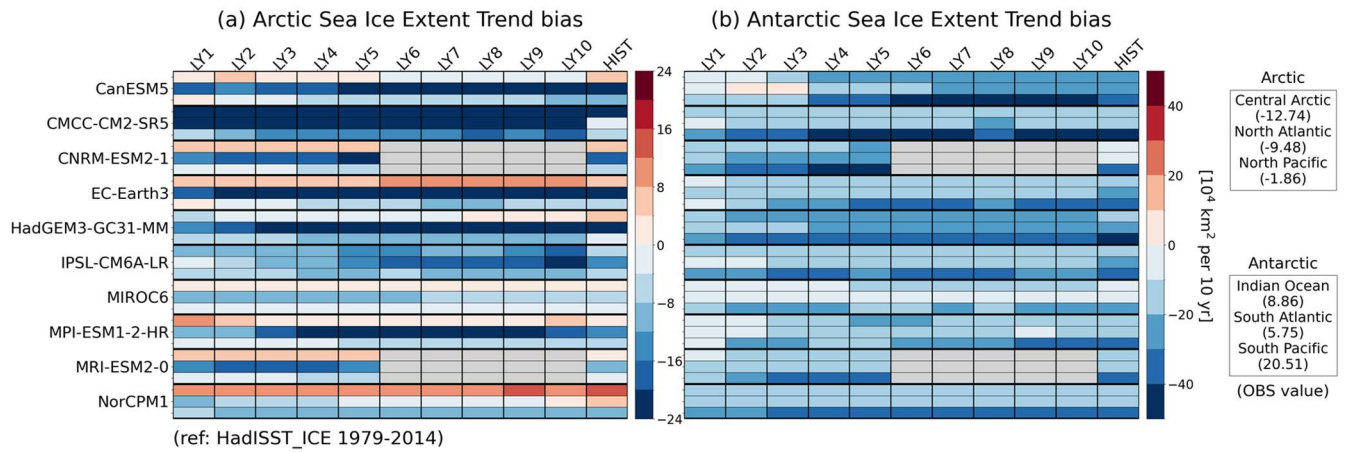
290 Figure 6. Same as Fig. 2, but for the trend bias of (a) the Arctic and (b) the Antarctic sea-ice extent. Units are [ 10^4 km 2 per 10 yr].
