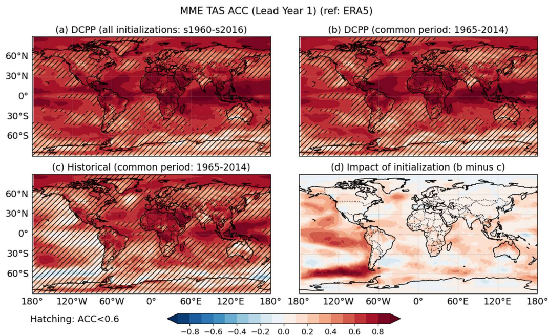
Figure 10: This example figure illustrates the spatial distribution of MME at LY1 of TAS ACC. (a) ACC calculated from all available DCP experiments initialized from 1960 to 2016. (b and c) Same as (a) but for the common evaluation period of 1965–2014 from DCP and HIST simulations, respectively. Regions with ACC below 0.6 are hatched to indicate limited practical prediction skill. (d) The difference between (b) and (c) represents the added skill due to initialization. Red regions indicate areas where initialization improves prediction skill.
