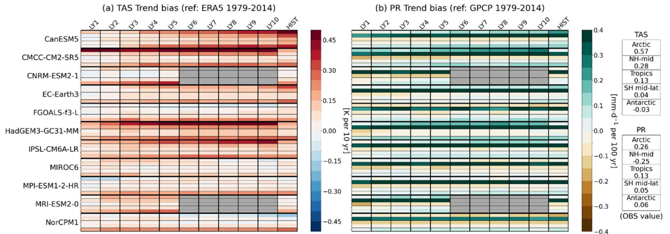
285 Figure 5. Same as Fig. 1, but for the trend bias over the period 1979–2014. The trend bias is defined as the difference in trend between the model and the observations. Units are [K per 10 yr] for (a) TAS and [mm d -1 per 100 yr] for (b) PR. Trend bias is calculated for each month and each grid cell, and then annual and area averages are taken.
