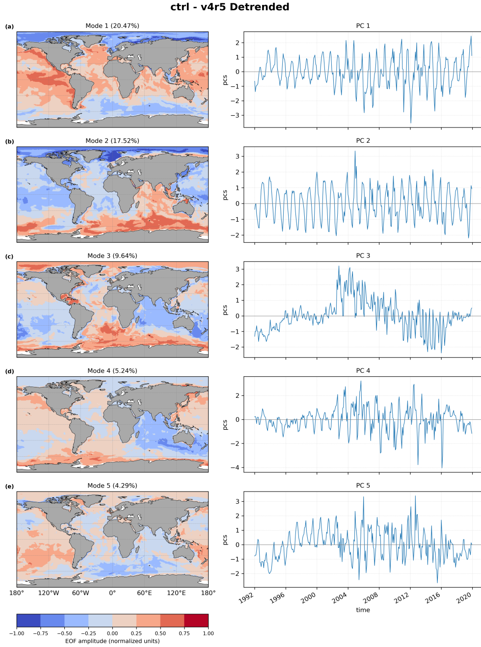
Figure 7. First five empirical orthogonal functions of the detrended ECCOctrl–ECCOv4r5 p_b fields based on the full 28-year record (1992–2019). Time series of principal components (PC) are in units of cm.
