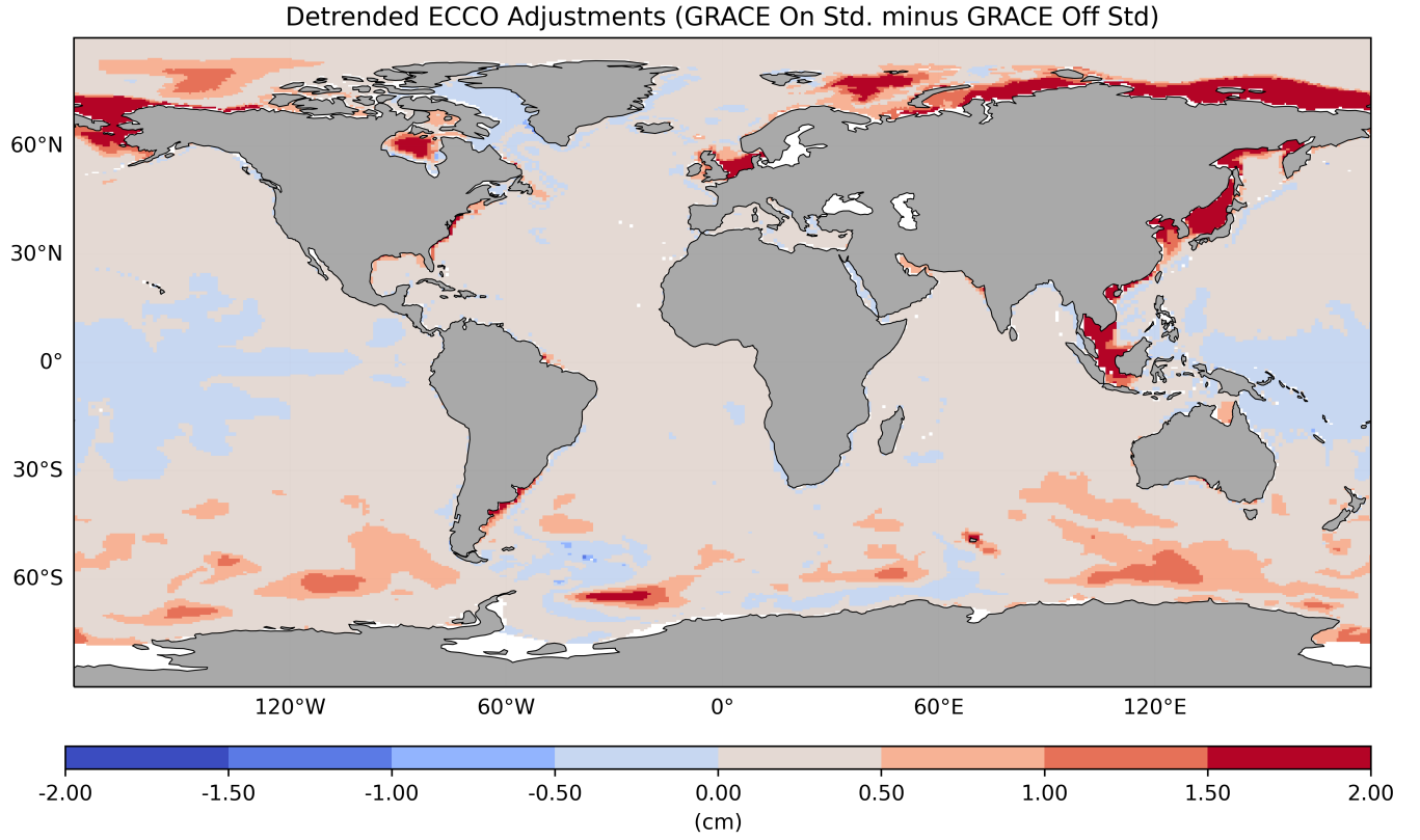
Figure 9. Difference in the temporal standard deviations of detrended ECCOctrl–ECCOv4r5 fields, calculated for periods with and without GRACE observations. Positive values indicate larger p_b adjustments for periods with GRACE data.
