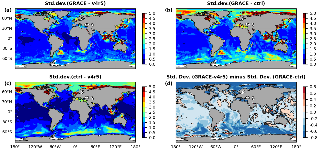
Figure 2. Standard deviation of the difference fields (a) GRACE–ECCOv4r5, (b) GRACE–ECCOctrl and (c) ECCOctrl–ECCOv4r5, based on their overlapping period. Global spatial means have been removed from all the fields. The difference (a) minus (b) is shown in (d).
