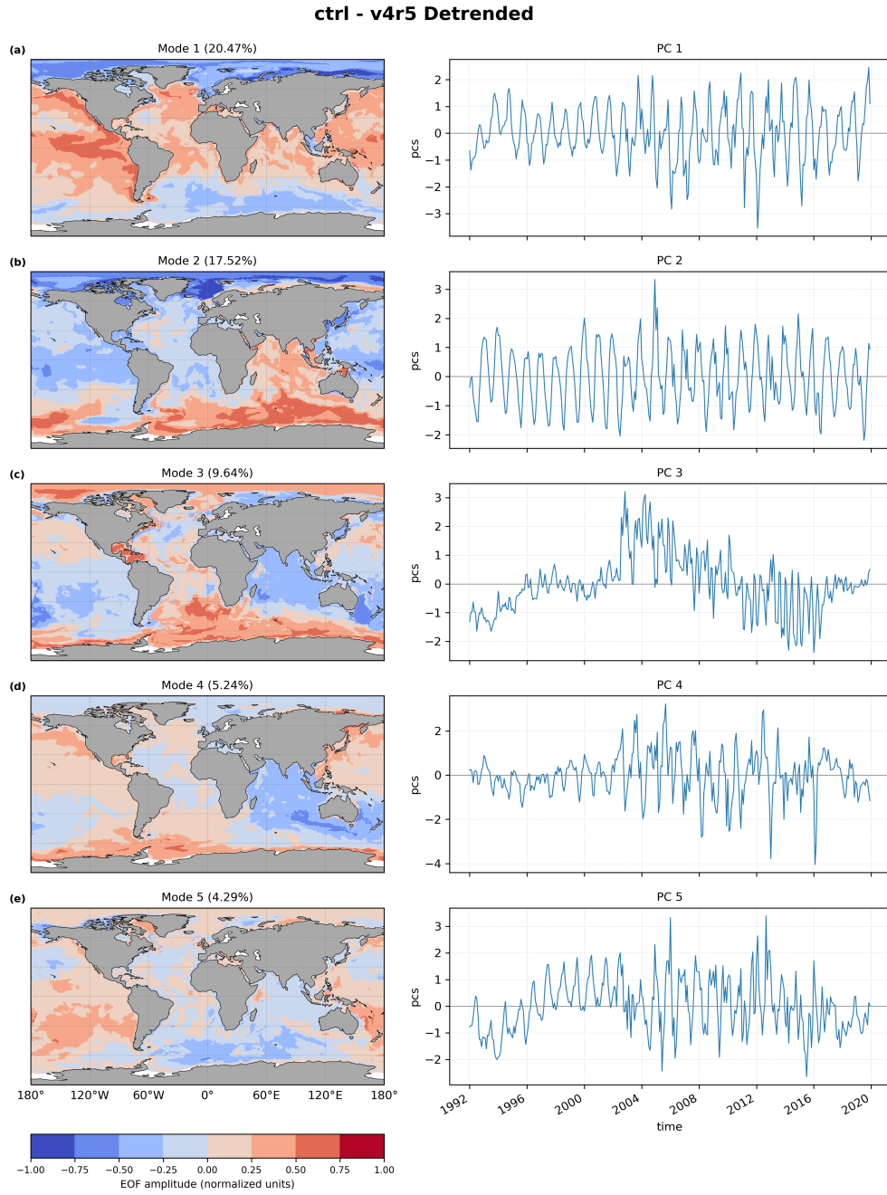
Figure 7. First five empirical orthogonal functions of the detrended ECCOctrl–ECCOv4r5 fields based on the full 28-year record (1992–2019).
