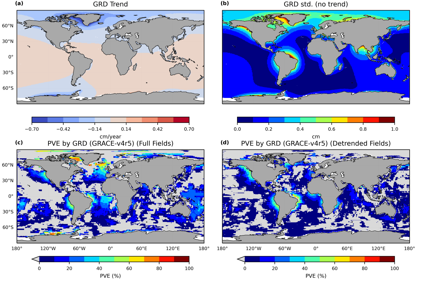
Figure 12. (a) Trends (cm/yr) and (b) standard deviations (cm) of the GRD fields, and (c,d) the percentage of variance in GRACE–ECCOv4r5 fields explained by GRD, based on full fields (c) and detrended fields (d).
