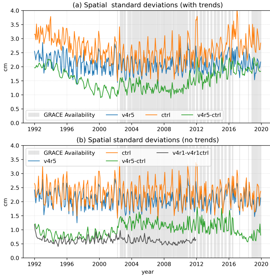
Figure 8. Time series of the spatial standard deviation of the ECCOctrl–ECCOv4r5 fields (green), calculated based on (a) full values and (b) detrended values. Shaded areas denote periods with GRACE data availability. Standard deviations of the corresponding p_b fields for ECCOctrl and ECCOv4r5 are also shown for comparison.
