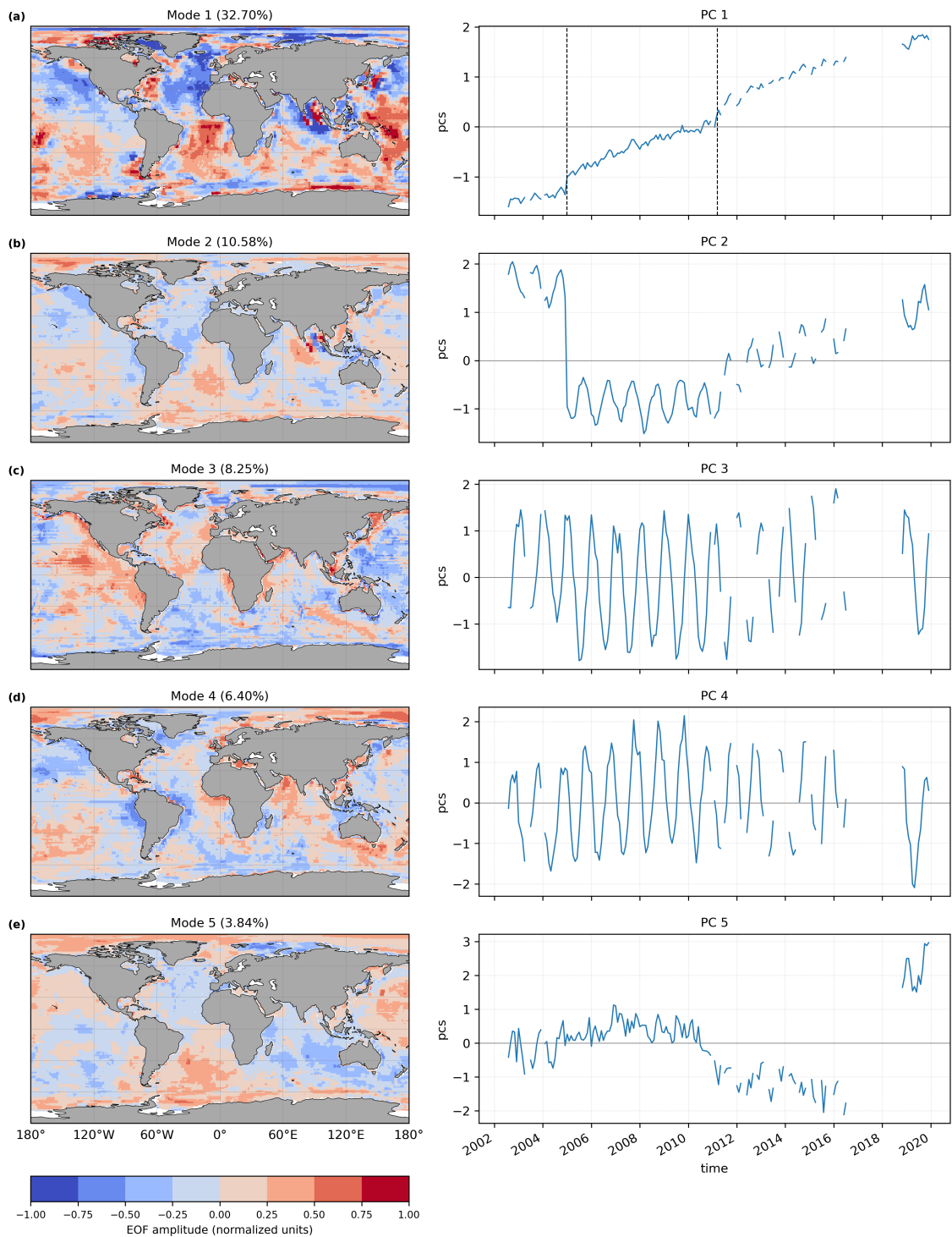
Figure 11. First five empirical orthogonal functions of the GRACE–ECCOV4r5 fields.
