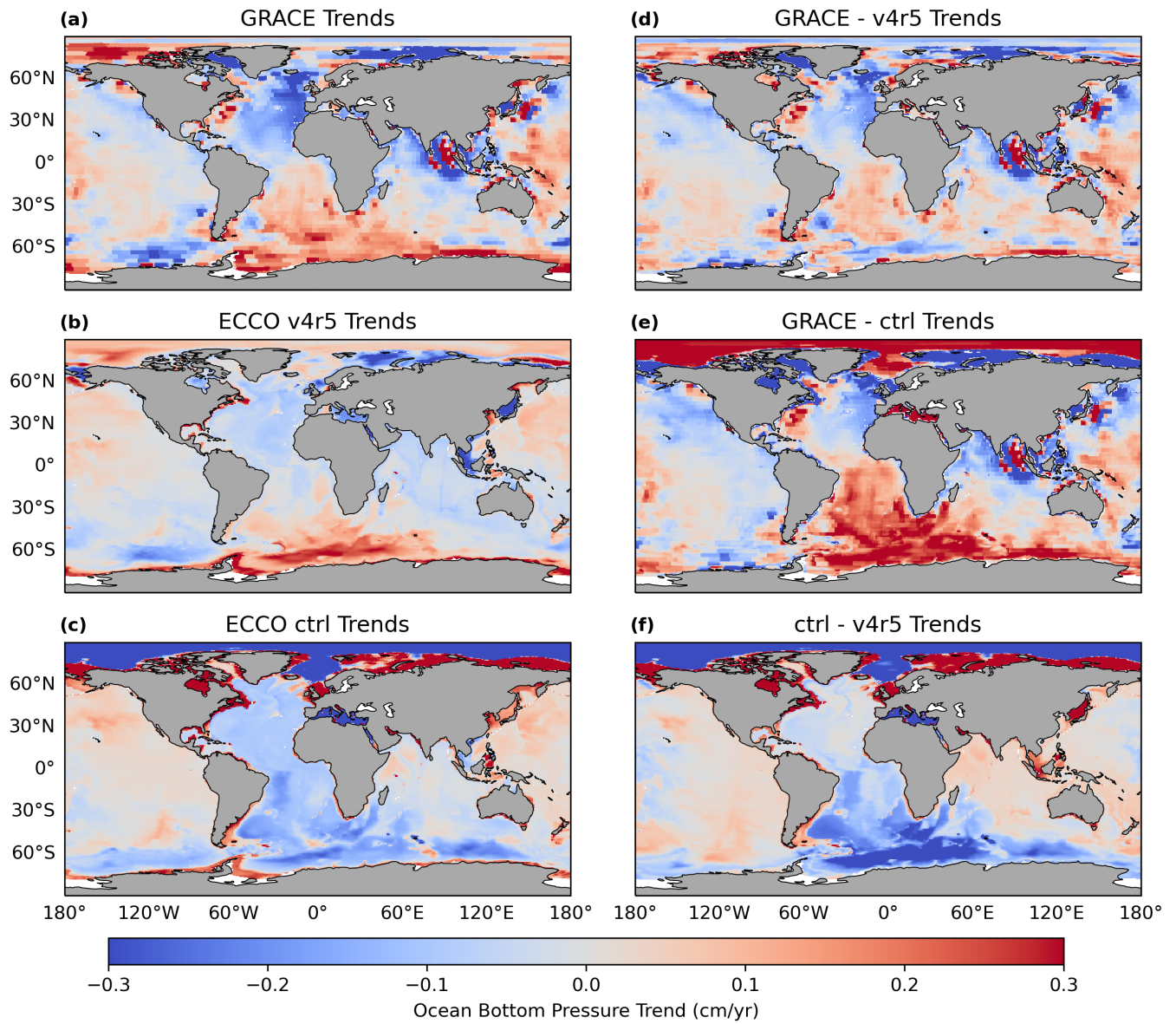
Figure 4. Trends of p_b fields for (a) GRACE, (b) ECCOv4r5, and (c) ECCOctrl, and respective differences (d) GRACE–ECCOv4r5, (e) GRACE–ECCOctrl, and (f) ECCOctrl–ECCOv4r5, all in units of cm/yr .
