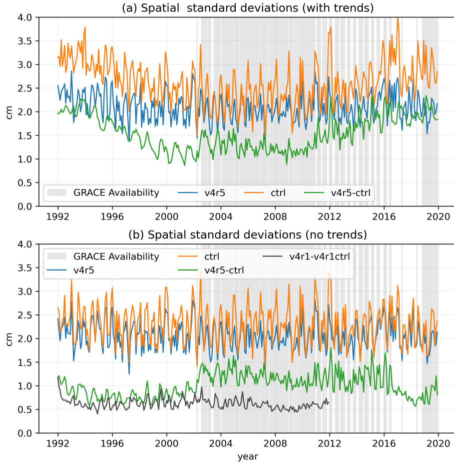
Figure 8. Time series of the spatial standard deviation ( cm ) of the ECCOctrl–ECCOv4r5 p_b fields (green), calculated based on (a) full values and (b) detrended values. Black curve in (b) denotes the standard deviation of differences between ECCOv4r1 and respective control run for comparison. Shaded areas denote periods with GRACE data availability. Standard deviations of the corresponding p_b fields for ECCOctrl ( orange ) and ECCOv4r5 ( blue ) are also shown for comparison context .
