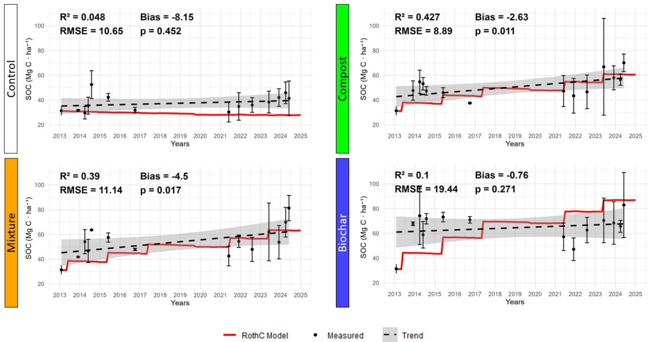
Figure 4. Comparative analysis of RothC model simulations (red line) against sampled-measured SOC data (black dots) for each treatment. Error bars represent the standard deviation. The black dashed line represents the regression line calculated from the measured values, with the shaded area showing 95% confidence interval. Model performance statistics ( R^2 , RMSE, Bias, and p-value ) are reported. The RMSE and Bias metrics are expressed in (\text{Mg C} \cdot \text{ha}^{-1}) .
