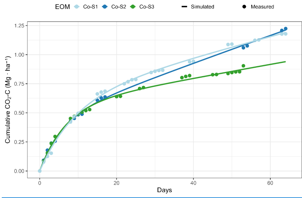
Figure 3. CO 2 emissions by compost amendment for different soils: measured (dots) and RothC-simulated (lines) cumulative CO 2 -C (Mg ha -1 )
