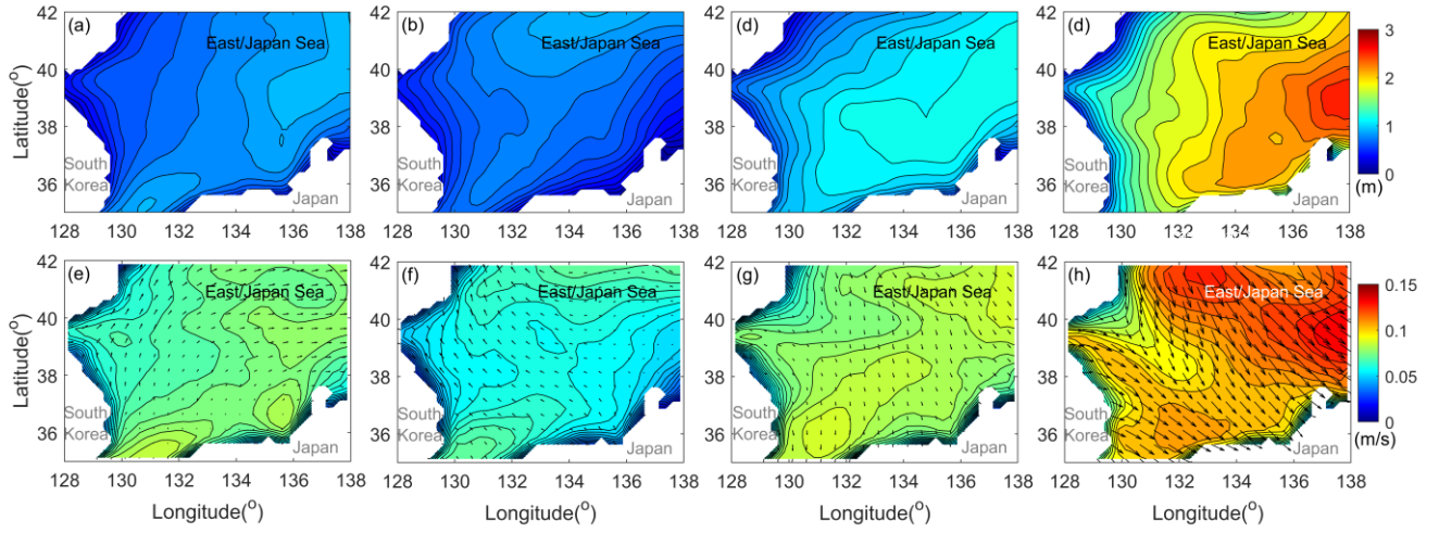
Figure 11. The mean of significant wave height (a-d), wind (e-f) in EJS for each season in 2021: (a,e) spring (March 01-May 30), (b,f) summer (June 01-August 30), (c,g) autumn (September 01-November 30), and (d,h) winter (December 01-February 28).
