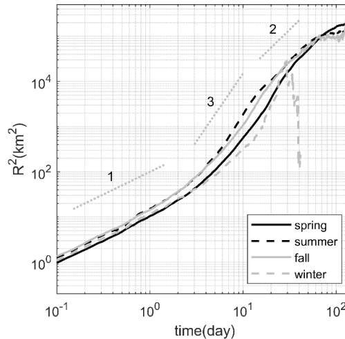
Figure 15. Seasonal variation of relative dispersion, R^2(t) , for particles (same as those used in Fig. 13, and 14) simulated using the optimal forcing combination (C7). Lines indicate relative dispersion for particles released in spring (black solid), summer (black dashed), autumn (gray solid), and winter (gray dashed).
