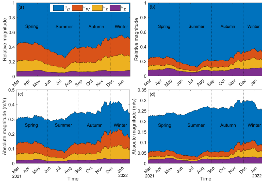
Figure 12. The relative and absolute value of the current components at the surface (a,c) and 1.5m-depth (b,d) of ( u_G -geostrophic current, u_W -wind-driver current, u_S -Stoke current and u_E -Ekman current) from March 2021 to February 2022.
