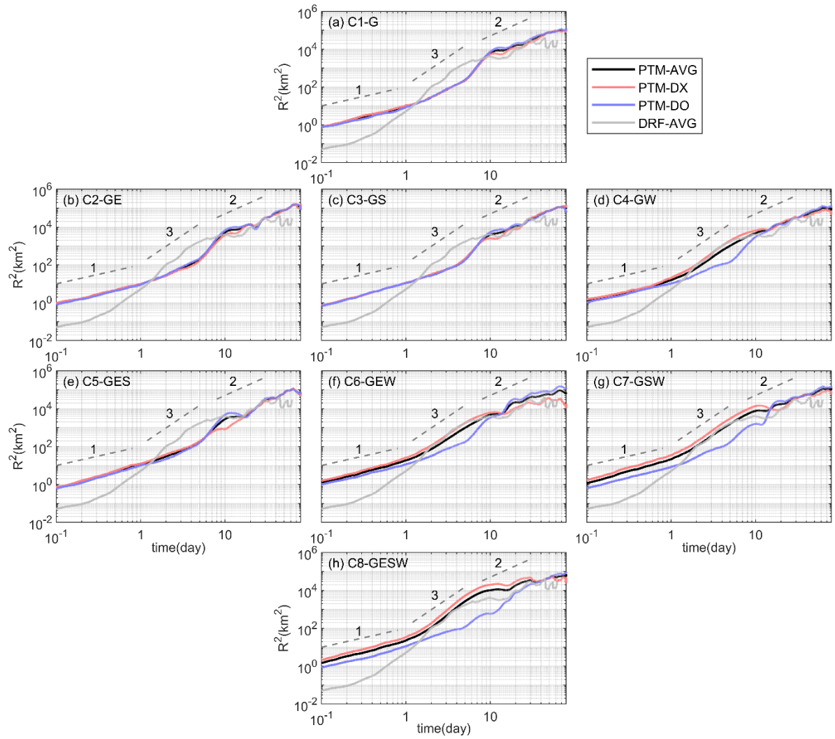
Figure 7. Relative dispersion ( R^2(t) ) of particles simulated with different forcing combinations (C1-C8) as described in Table 1, shown alongside observed drifter dispersion. Panels are arranged in the same order as in Fig. 5 and 6. Red and blue lines represent the relative dispersions for PTM-DX and PTM-DO simulations, respectively, and the gray line represents the average relative dispersion of the observed drifters for comparison. G, E, S, and W indicate geostrophic current, Ekman current, Stokes drift, and windage forcings, respectively.
