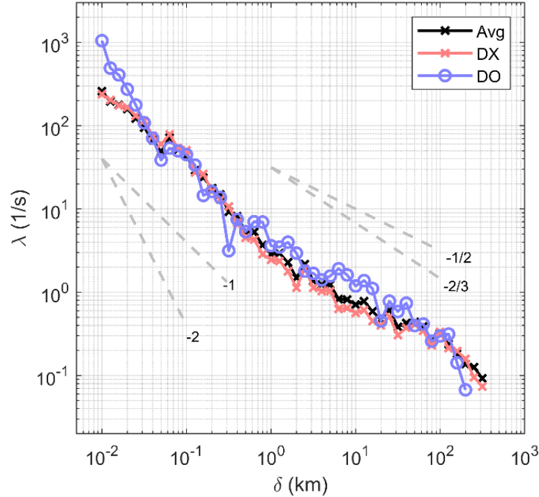
Figure 4. Finite-Size Lyapunov Exponent (FSLE), \lambda , as a function of separation distance, \delta , for the observed drifters. The black line represents the average of all drifters, the red line represents the undrogued (DX) drifters, and the blue line represents the drogued (DO) drifters. The dashed gray lines indicate reference slopes of -2, -1, -1/2, and -2/3.
