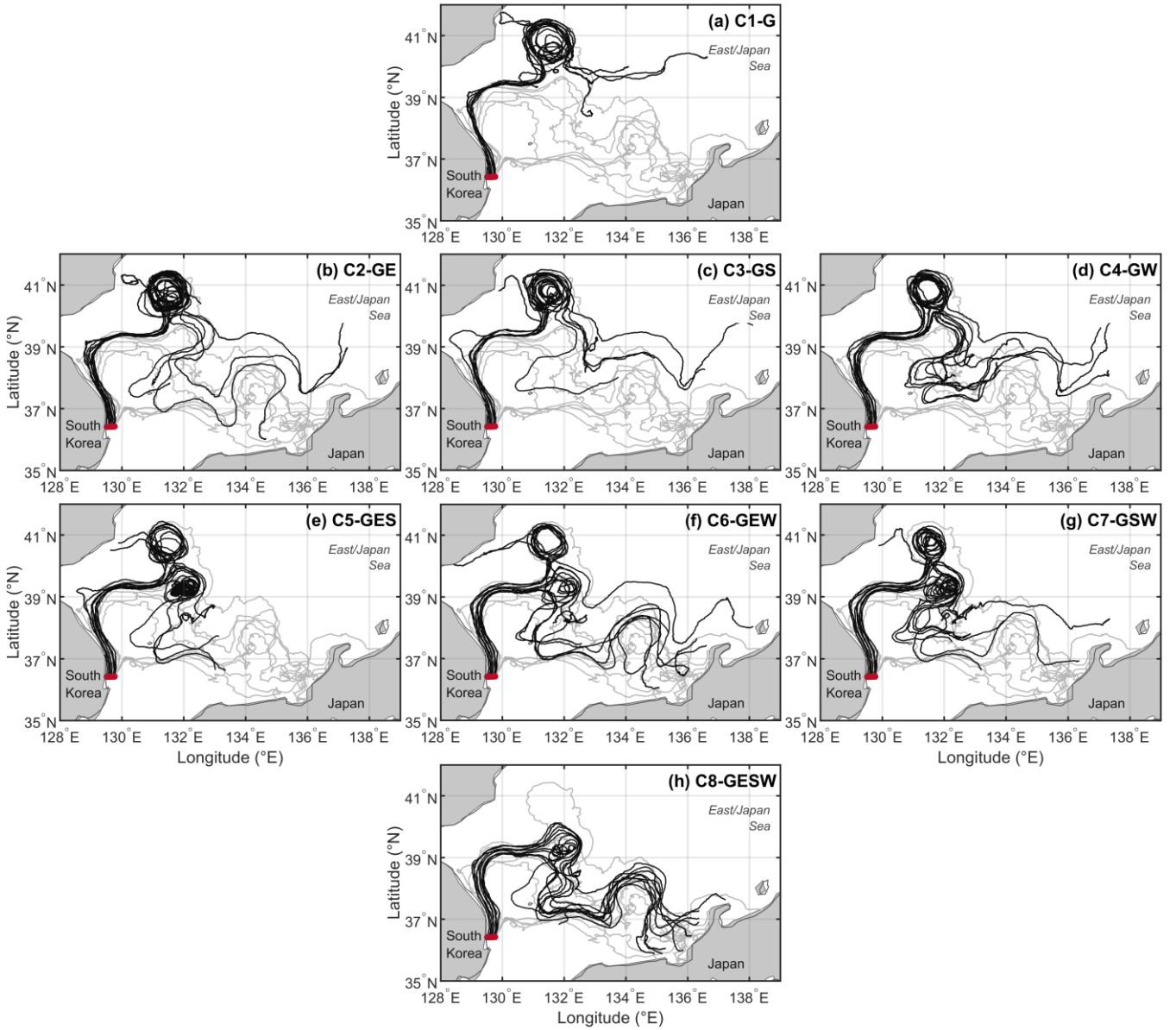
Figure 6. Observed trajectories of drogued DO drifters (gray) and simulated PTM-DO trajectories (black) over the 79-day simulation period for forcing combinations C1-C8 listed in Table 1. For PTM-DO, the Ekman current and Stokes drift were evaluated at the effective depth of 1.5 m. Red markers indicate the initial release locations. All panels use the same geographic domain, coordinate units, and labels for South Korea, Japan, and the East/Japan Sea. Panels (a-h) correspond to C1-C8 and are arranged by the number of forcing components: C1; C2-C4; C5-C7; and C8. G, E, S, and W denote geostrophic current, Ekman current, Stokes drift, and windage, respectively.
