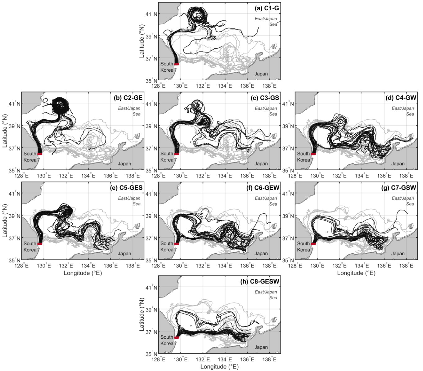
Figure 5. Observed trajectories of undrogued DX drifters (gray) and simulated PTM-DX trajectories (black) over the 79-day simulation period for forcing combinations C1-C8 listed in Table 1. Red markers indicate the initial release locations. All panels use the same geographic domain, coordinate units, and labels for South Korea, Japan, and the East/Japan Sea. Panels (a-h) correspond to C1-C8 and are arranged by the number of forcing components: C1; C2-C4; C5-C7; and C8. G, E, S, and W denote geostrophic current, Ekman current, Stokes drift, and windage, respectively.
