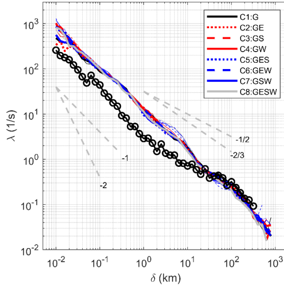
Figure 8. Finite-Size Lyapunov Exponent (FSLE), \lambda , as a function of separation distance, \delta , for the simulated particles and observed drifters. The black line with circles represents the FSLE averaged for all observed drifters. Other colored lines show FSLEs for simulated particles from different forcing combinations (C1-C8, as listed in Table 1). Thinner lines indicate PTM-DX simulations, and thicker lines indicate PTM-DO simulations. The variation in FSLE values between different forcing combinations and between PTM-DX and PTM-DO were small.
