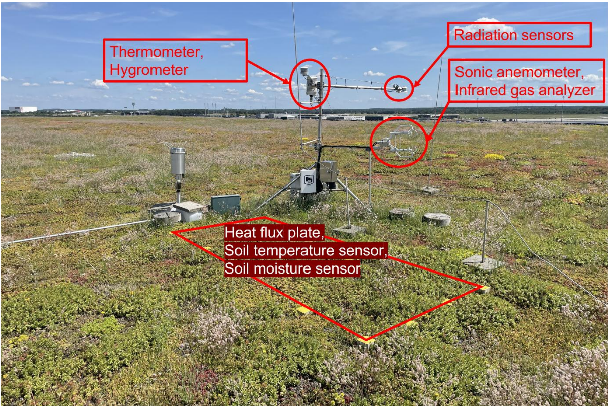
Figure A1. Photo of the green roof and measurement setup taken on 18.07.2024.
