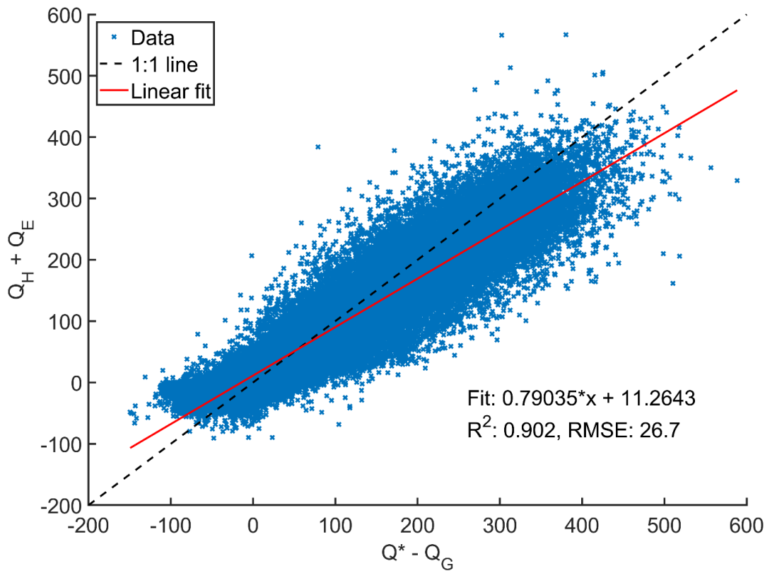
Figure A5. Half-hourly values of available energy ( Q^* - Q_G ) plotted against the sum of turbulent heat fluxes ( Q_H + Q_E ). A linear regression has been fit (red line) and the 1:1 line (dashed) plotted.
