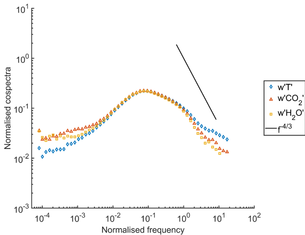
Figure A4. Cospectra (sensible heat, CO 2 , H 2 O) for unstable stratification ( -650 m < L < 0 m) for the time period of 01.04.2022–31.03.2023.
