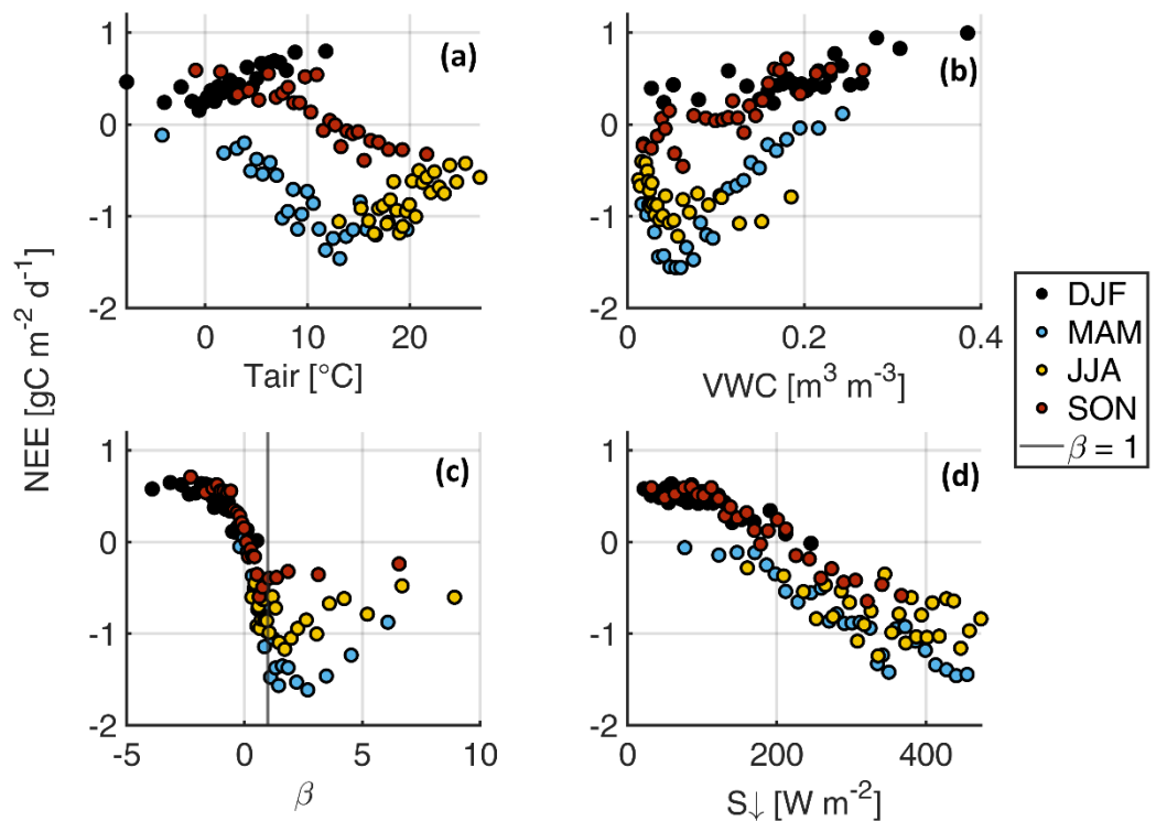
Figure 12: Net Ecosystem Exchange (NEE) in dependence on air temperature ( T_{\text{air}} , a), volumetric water content (VWC, b), Bowen-ratio ( \beta , c) and daytime shortwave-downward radiation ( S_{\downarrow} ,d). Daily means of the independent variables were used and sorted according to their value. A new bin was created every 30 values, and for each bin, the median value of the dependent variable was calculated and assigned to the mid-value of the bin. DJF = winter, MAM = spring, JJA = summer, SON = autumn.
