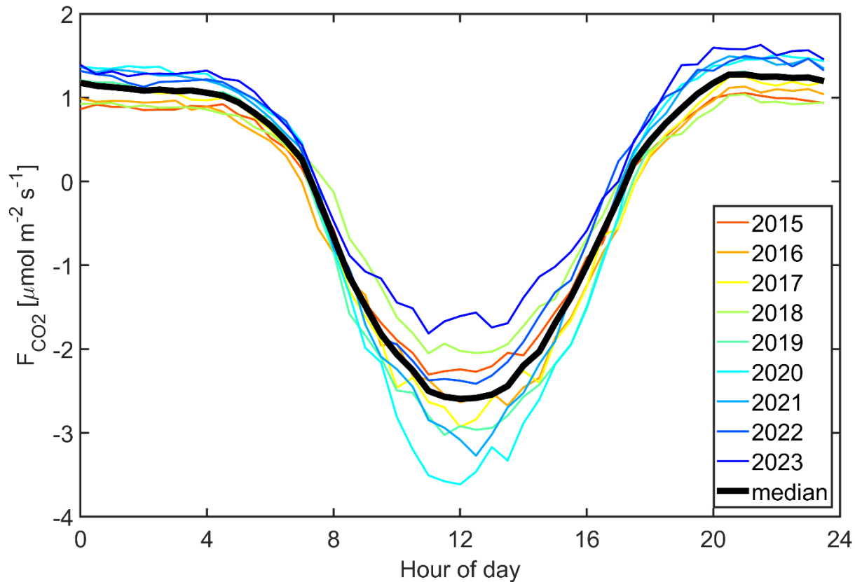
Figure 6: Median diurnal cycle of the carbon flux over the whole study period and for each year.
