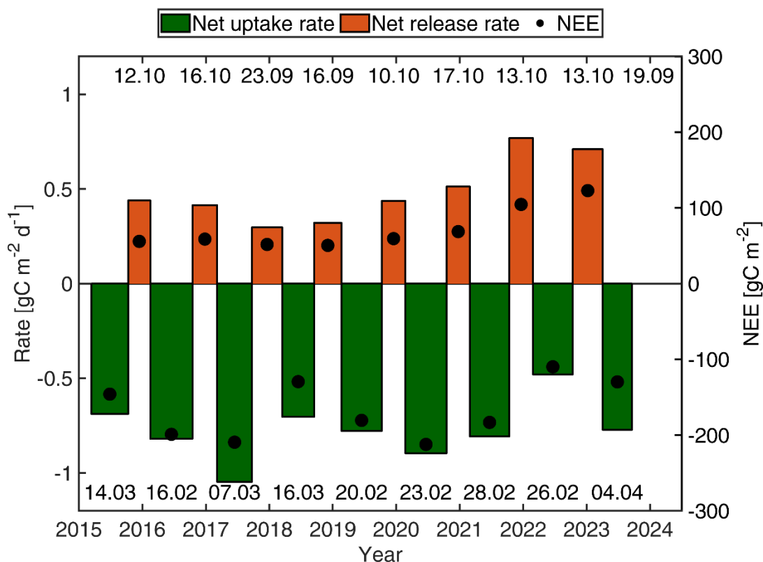
Figure 10: Net sink and net source seasons during the study period. The net uptake/release rate is indicated by the bars, the sum of carbon flux (NEE) by the black circles. The day and month of the beginning of each phase are shown.
