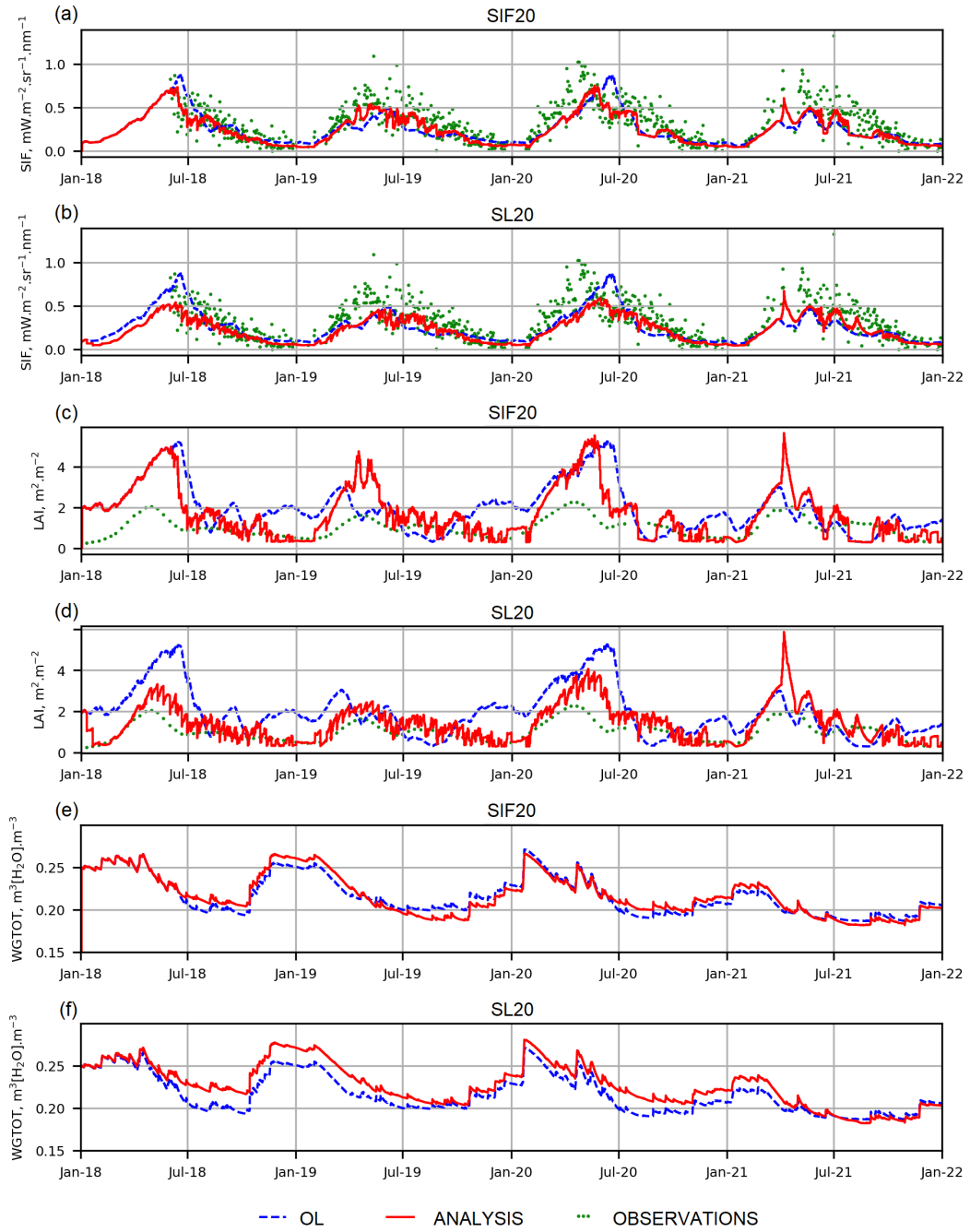
Figure 7. Timeseries extract on the cell locate in 1.05^{\circ}\text{E} , 41.65^{\circ}\text{N} for the SIF (a,b), the LAI (c,d) and the the total soil moisture (WGTOT) in the column (e,f). The open loop (OL in Table 1) indicated with dashed blue lines, SIF 20 (panels a,c,e) and SL 20 (panels b,d,f) analyses with the plain red line in their respective panels and observations with green dots. The observations for the SIF, and LAI are respectively extracted from TROPOMI SIF and LAI-300 described in section 2.2.3
