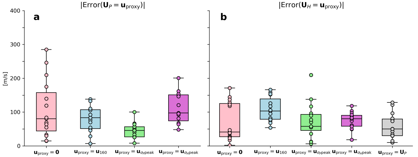
Figure 3. (a) For 15 neutral wind profiles, box-and-whisker plots of the magnitude of the Pedersen-weighted neutral wind ( \mathbf{U}_P , pink), the magnitude of the differences between \mathbf{U}_P and the neutral wind at 160-km altitude ( \mathbf{u}_{160} , blue), the magnitude of the difference between \mathbf{U}_P and the neutral wind at the height at which the Pedersen conductance maximizes ( \mathbf{u}_{\sigma_P \text{ peak}} , green), and the magnitude of the difference between \mathbf{U}_P and the neutral wind at the height at which the Hall conductance maximizes ( \mathbf{u}_{\sigma_H \text{ peak}} , violet). The first and second represent the error associated with assuming \mathbf{U}_P = 0 m/s and \mathbf{U}_P = \mathbf{u}_{160} ; the latter two represent the error associated with assuming \mathbf{U}_P is one of the two proxies. The horizontal lines above and below each box-and-whisker plot are the minimum and maximum except in panel b for \mathbf{u}_{\text{proxy}} = \mathbf{u}_{\sigma_P \text{ peak}} , shown in green, where one value is an outlier (see main text). (b) Same layout as panel a, but for the Hall-weighted neutral wind \mathbf{U}_H and with an additional box-and-whisker plot (gray at far right) to assess \mathbf{U}_H = \mathbf{U}_P . The point of this figure is to answer Question 2 posed at the beginning of Section 3 by assessing whether any proxy for the Hall- and Pedersen-weighted neutral winds statistically incurs less error than simply assuming that they are zero.
