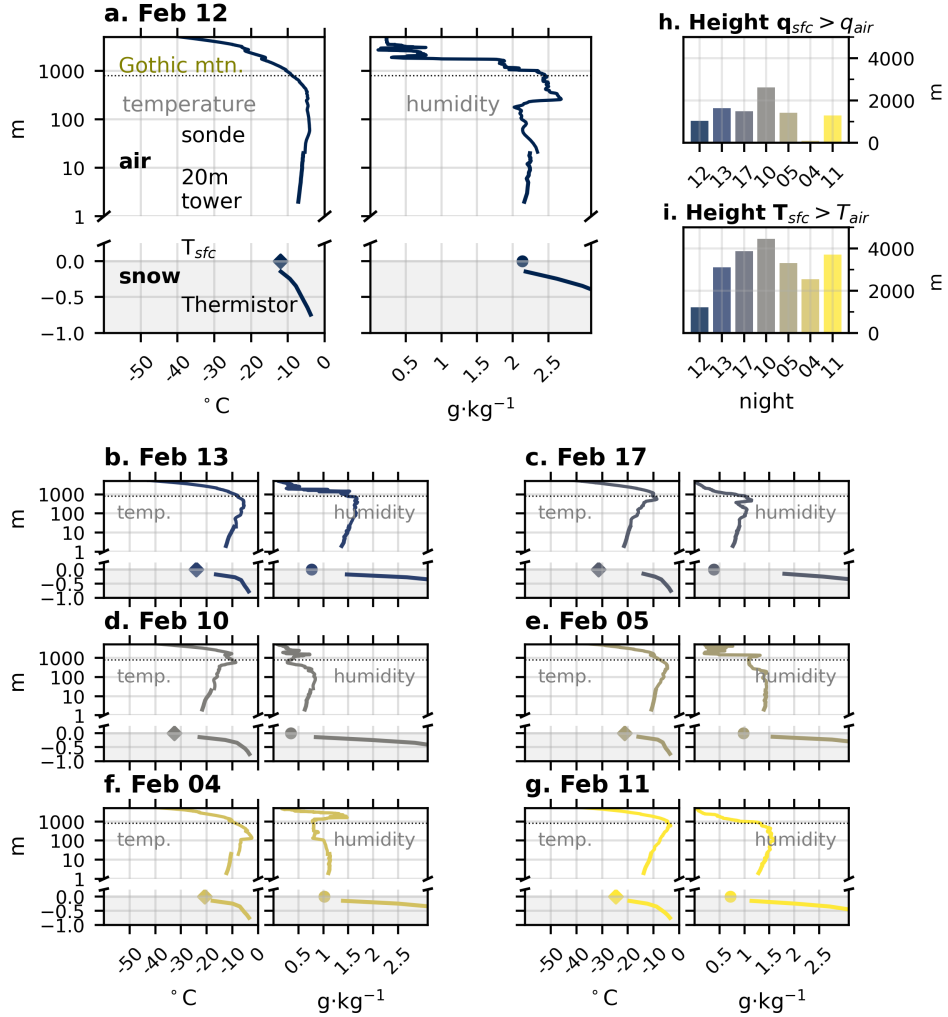
Figure 4. (a–g) 5:00 a.m. local time profiles of T_{air} and q_{air} throughout the snow-atmosphere continuum as measured by SOS towers, balloon sondes, down-looking radiometers ( T_{sfc} ), and buried snow thermistor arrays. Note the log scale y-axis. Units are heights in meters with respect to the snow surface height, defined as 0. (h, i) Barplots on the top-right depict the lowest atmospheric height level at which T_{sfc} and q_{sfc} exceeds the respective value in the atmosphere for each night. The panels are ordered by the size of the surface hoar event in the same order as (Fig. 8).
