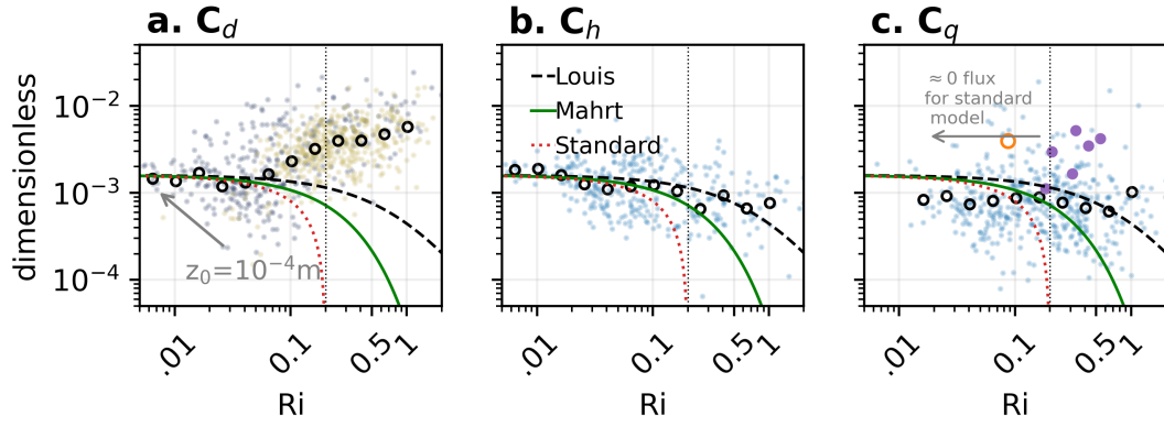
Figure 6. Relationship between Ri and the bulk transfer coefficients for (a) momentum (b) heat, and (c) moisture computed from EC fluxes and bulk gradients using Eq. 2—4. Blue circles in (a) — (c) are 30-minute values for all time periods considered and black open circles are bin-averages. Yellow circles in (a) denote clear-sky conditions. Purple and orange circles are estimated from Stössel box observations and digitized data from H97 respectively in (c). The solid, dashed, and dotted lines correspond to theoretical stability correction curves using the Mahrt, Louis, and standard parameterizations implemented in the SUMMA model and z_0 = 2 \times 10^{-4} .
