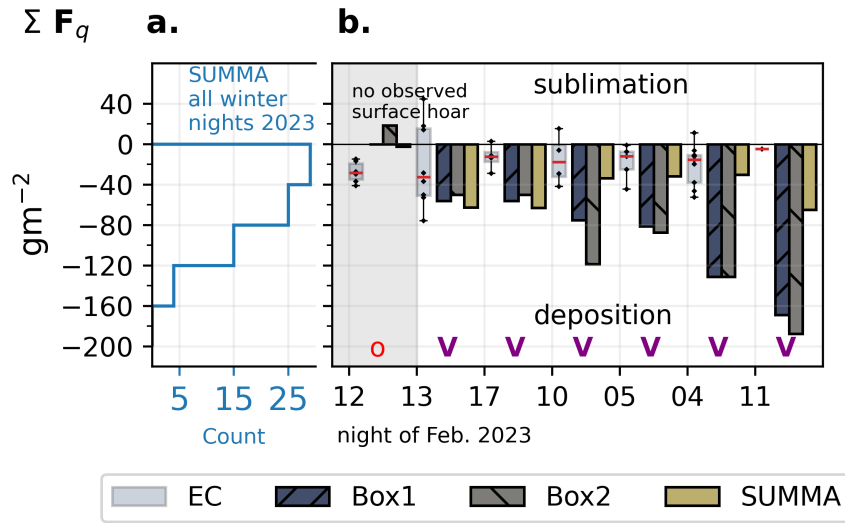
Figure 8. Validation of SUMMA against Stössel box observations: (a) histograms of total nightly cumulative deposition amount ( \Sigma F_q ) for the entire winter of 2023 from SUMMA and (b) barplots of \Sigma F_q for the 6 confirmed surface hoar events in Feb. 2023 compared against duplicate Stössel box observations (Box1, Box2). Boxplots of 30-minute EC fluxes observed at 3m are also depicted (multiplied by the length-of-night in seconds for purposes of comparison). The no surface hoar observation on the 12th is denoted by gray-shading in the background and the red open circle. Purple "V" markers denote nights with observed surface hoar.
