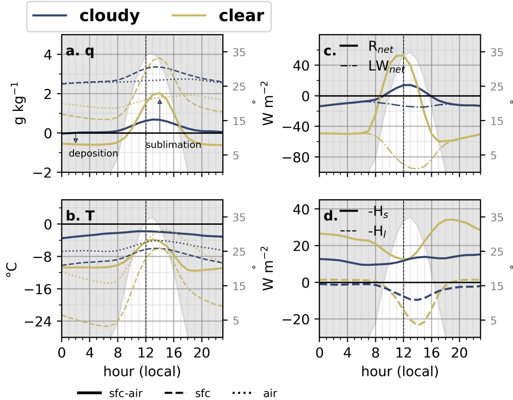
Figure 3. Composites of the diurnal evolution of observed (a) q , (b) T , (c) R_{\text{net}} and LW_{\text{net}} , and (d) turbulent fluxes ( H_s , H_l ) estimated from the bulk method under cloudy (dark blue) and clear (dark yellow) conditions from two winters at the M1 site. The additive inverse of H_l and H_s are depicted for convenience; positive values indicate the snowpack gains heat, and negative values the opposite. In panels (a) and (b), the dashed, dotted, and solid lines denote the snow surface, atmospheric, and snow-atmosphere difference ( \Delta ) for T and q respectively. The vertical dashed line marks local noon and the solar elevation angle is depicted by the unfilled white region.
