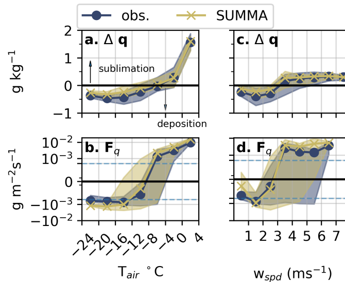
Figure 9. The sensitivity of overnight 30-minute \Delta q and F_q to T_{\text{air}} (a,b) and w_{\text{spd}} (c,d) from both observations and SUMMA output expressed as bin-averages. Shaded regions depict the 25th and 75th percentile ranges within each bin. Note that the y-axes for (b) and (d) use a symmetric logarithmic scale, with a linear region between the blue dashed lines.
