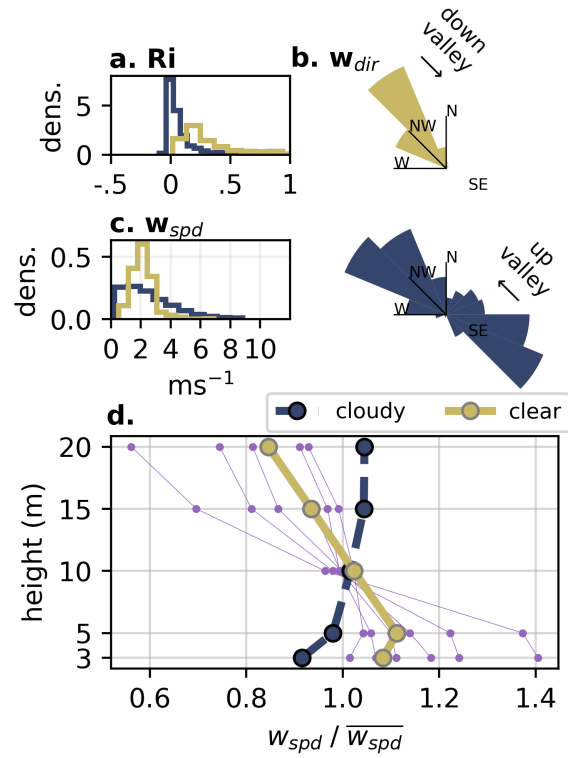
Figure 5. Wind conditions during clear and cloudy periods at the SOS KP site during winter of 2023: (a) histograms of Ri , (b) w_{dir} , (c) w_{spd} , and (d) vertical profiles of normalized wind speed ( w_{spd} / \overline{w_{spd}} ). The purple lines show wind profiles for observed February surface hoar cases. Up and down-valley wind directions with respect to the valley geometry are labeled in (b).
