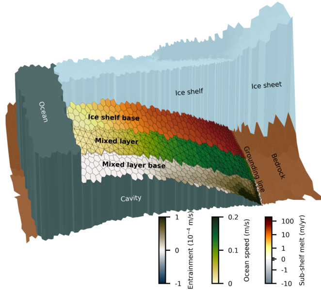
Figure 1. Schematic of main processes and their spatial discretisation: entrainment at the base of the mixed layer (voronoi cells), ocean currents within the mixed layer (triangular prisms with finite thickness), and sub-shelf melting (voronoi cells) at the ice/ocean interface. This illustration is based on an ISOMIP+ simulation (Sec. 3.2.1) with resolutions ranging from 1 km near the grounding line to 4 km over the rest of the ice shelf.
