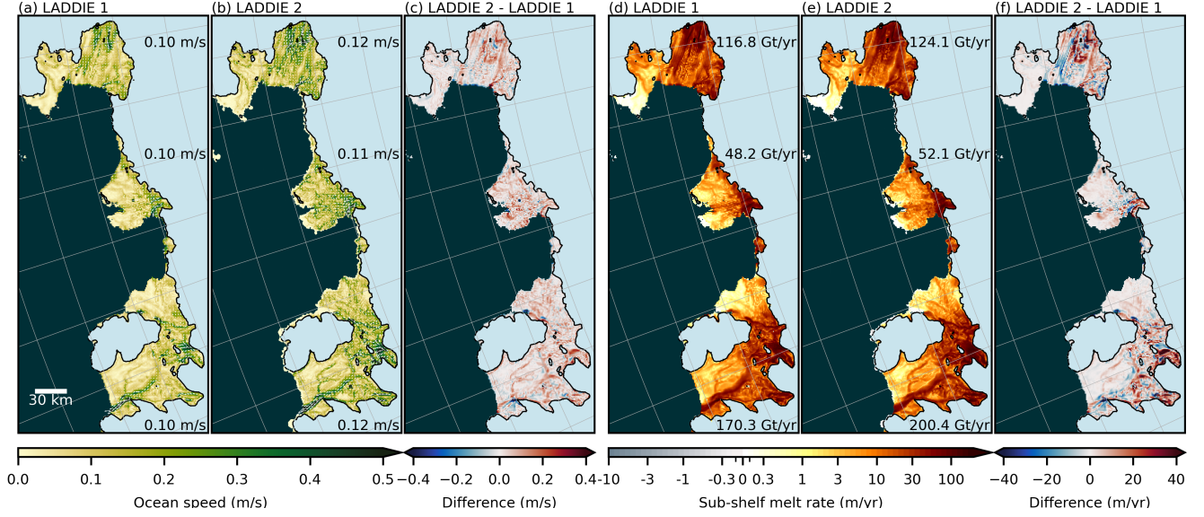
Figure 3. Amundsen Sea comparison between LADDIE 1.0 and LADDIE 2.0. Ocean speeds from (a) LADDIE 1.0, (b) LADDIE 2.0, and (c) the difference between the two model versions. White velocity vectors in (a,b) indicate the direction of the upper ocean flow. Average values for the Pine Island (top), Thwaites (middle), and Crosson–Dotson (bottom) ice shelves are noted. Sub-shelf melt rates for (d) LADDIE 1.0, (e) LADDIE 2.0, and (f) the difference. The numbers in (d,e) are integrated melt rates for the same three ice shelves. For visual reference, the grounding line (black line) as determined by LADDIE 2.0 is shown in each panel. Light blue colors denote grounded ice, dark green colors denote open ocean.
