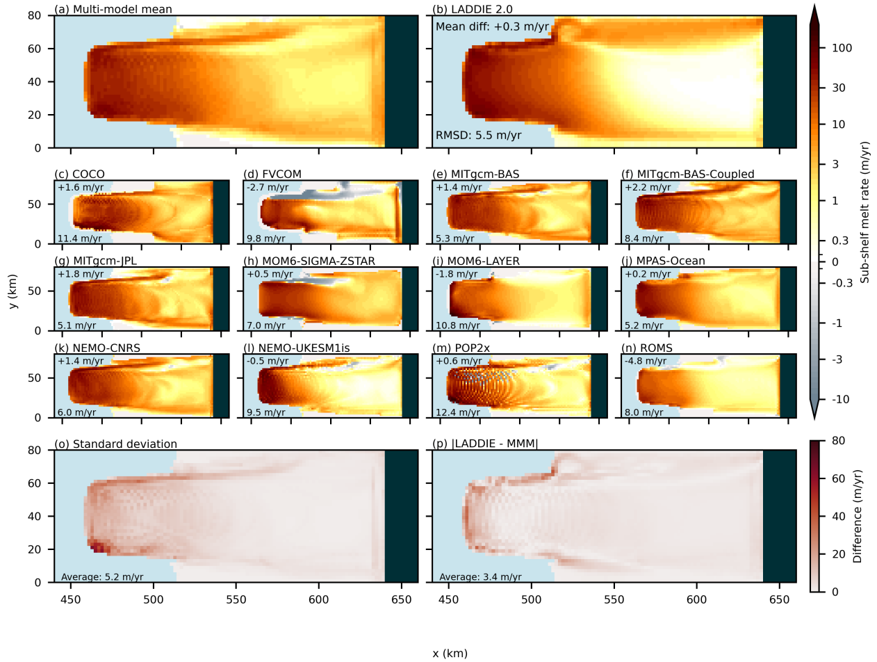
Figure 5. A comparison with 3D models based on the ISOMIP+ Ocean1 experiment. a) The multi-model mean sub-shelf melt rates of 12 ocean models. b) The results of LADDIE 2.0. c-n) The results of the individual models. o) The standard deviation of the 12 models. p) The absolute difference between LADDIE 2.0 and the multi-model mean. In panels b-n), two bulk quantities are included: the top number is the mean difference with respect to the multi-model mean; the bottom number is the root mean squared difference.
