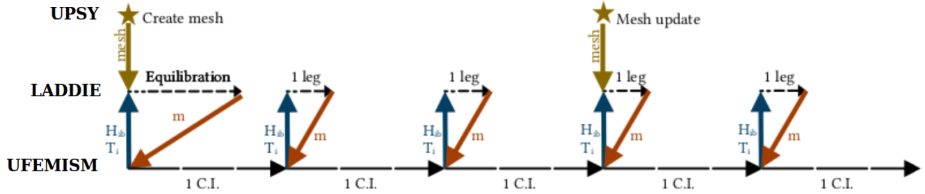
Figure 2. Illustration of the coupling strategy of UFEMISM and LADDIE. Dashed arrows indicate simulations of LADDIE and UFEMISM, the length of the dashes illustrates the time step, which ramps up during the first day of each LADDIE simulation. Coloured arrows indicate exchanged variables. C.I. stands for coupling interval.
