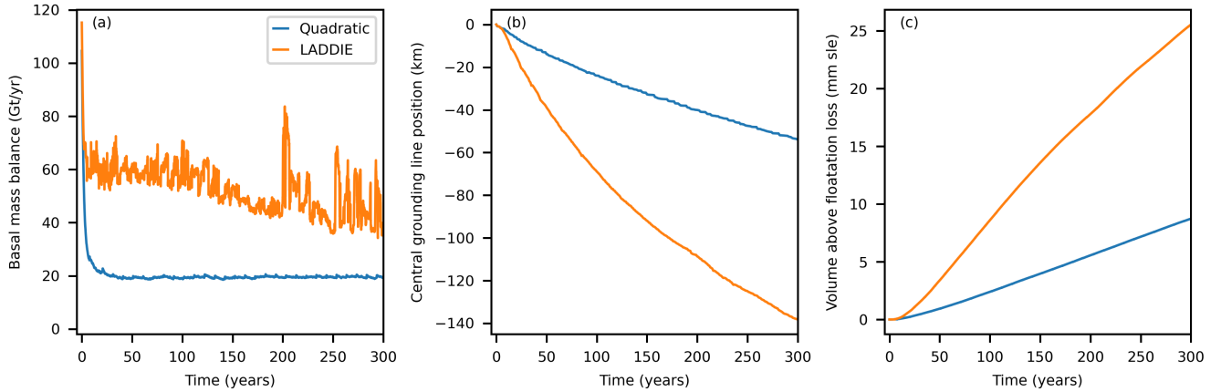
Figure 10. Time series of the two MISOMIP+ simulations. a) The integrated basal mass balance over the whole ice shelf. b) The grounding line position at y = 0 km, relative to the initial position at x = 450 km. c) The volume above floatation loss.
