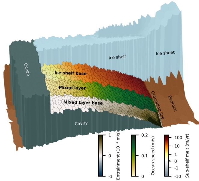
Figure 1. Schematic of main processes and their spatial discretisation: entrainment at the base of the mixed layer (voronoi cells), ocean currents within the mixed layer (triangles-triangular prisms with finite thickness), and sub-shelf melting (voronoi cells) at the ice/ocean interface. This illustration is based on an ISOMIP+ simulation (Sec. 3.2.1) with resolutions ranging from 1 km near the grounding line to 4 km over the rest of the ice shelf.
