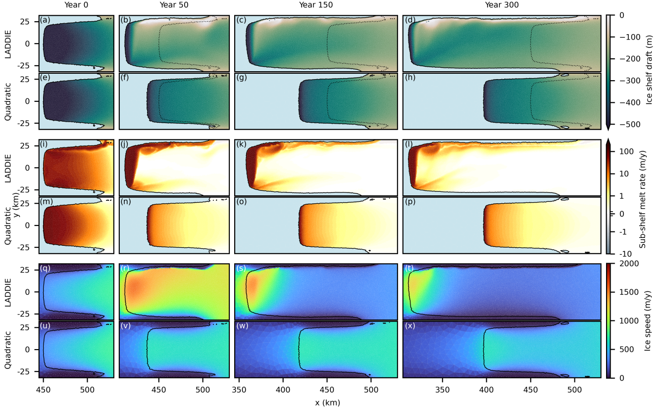
Figure 9. Ice–ocean interactions from UFEMISM comparing LADDIE to the quadratic parameterisation. The columns show four time slices of two idealised MISOMIP+ simulations. Three combined rows show the ice shelf draft (a-h), the sub-shelf melt rate (i-p), and the ice speed (q-x). For each combined row, the top row shows the LADDIE simulation, the bottom row the simulation with the quadratic melt parameterisation. Solid black lines represent the grounding line position, the dotted black lines (b-d and f-h) show the initial grounding line position (a and e).
