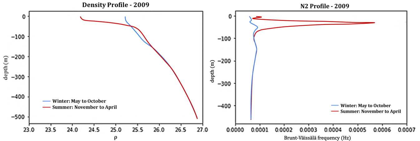
Figure 7. Left panel: Mean density profile around the VTR in the winter season (May to October) and in the summer season (November to April); Right panel: Mean Brunt-Väissälä frequency profile around the VTR in the winter season (May to October) and in the summer season (November to April)
