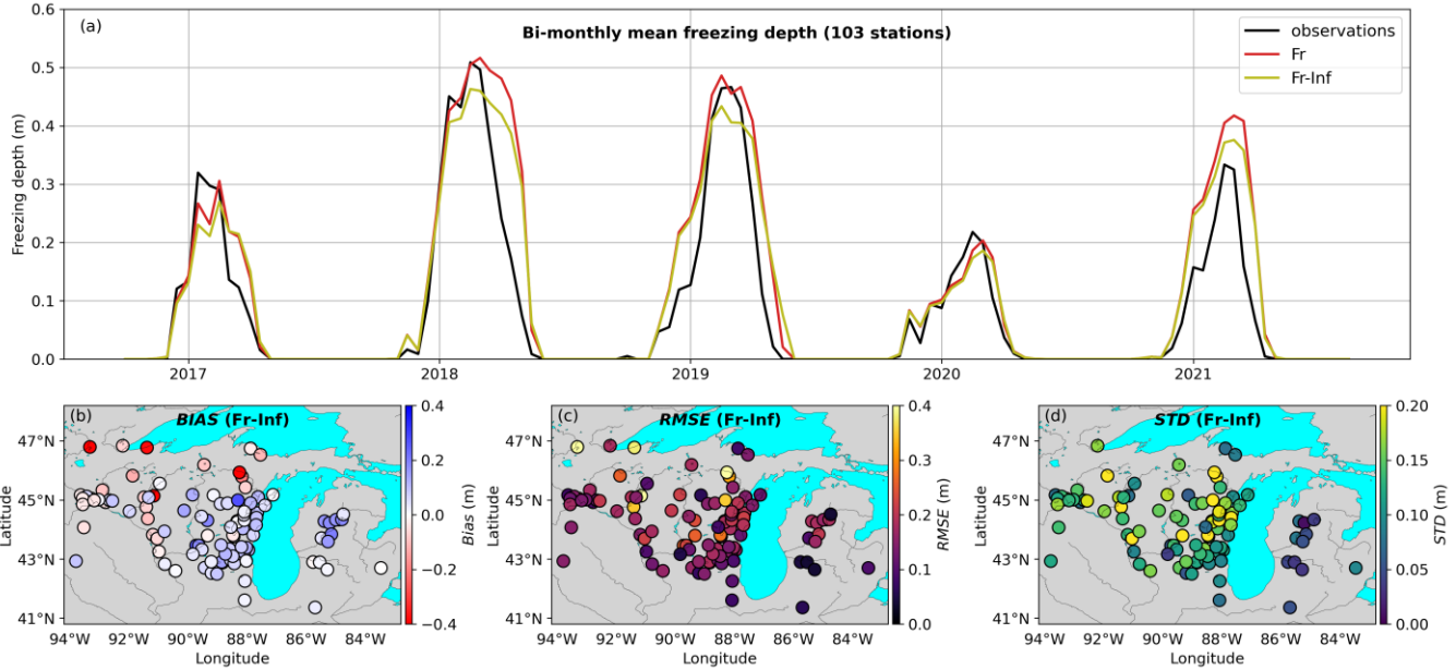
Figure 10: Bi-monthly mean of freezing depth for 103 stations located in the central US from 2016 to 2021 with observations shown in black and soil freezing (Fr) and enhanced frozen soil infiltration (Fr-Inf) simulations shown in red and yellow, respectively (a). The BIAS , RMSE and standard deviation ( STD ) at each station over the 2016-2021 period for the Fr-Inf experiment are respectively shown in (b), (c) and (d).
