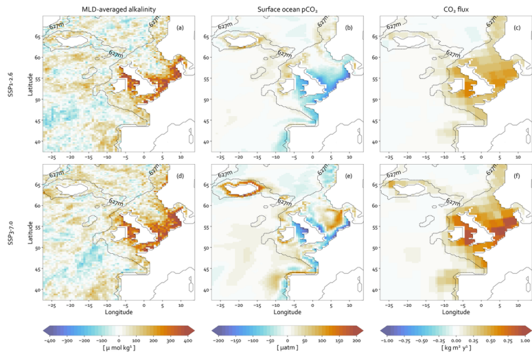
Figure 6: Seasonal amplitude change (OAE minus control run) averaged over 2090-2099 for MLD-averaged alkalinity (a, d), for surface ocean pCO 2 (b, e) and for the air-sea CO 2 flux (c, f). The top shows SSP1-2.6 and the bottom row shows SSP3-7.0. CO 2 flux calculations are performed on the atmospheric component of FOCI, which has a coarser resolution than the ocean component. The dashed line represents the shelf break set at the 627m isobath.
