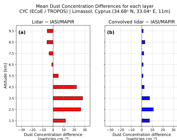
Figure 15. Dust concentration differences at each layer, regridded (a) and convolved (b) lidar vs IASI/MAPIR, for 12 dust cases over Limassol, Cyprus.
