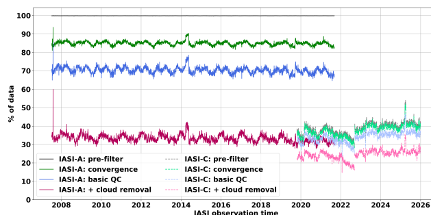
Figure 2. MAPIR v5.1 performance for IASI-A and IASI-C. In grey: the percentage of IASI observations for which the retrieval is run (passing all pre-filters), in green: the percentage of IASI observations for which the retrieval converges, in maximum 20 iterations; in blue: the percentage of retrievals passing the basic quality control criteria (i.e. RMS of spectral residuals below 0.75 K, 200\text{ K} < \text{surface temperature} < 350\text{ K} and dust AOD < 5 ; in pink: the percentage of retrievals passing all quality flags (i.e. also including those aiming to remove thin clouds, based on the difference between retrieved and a priori surface temperature))
