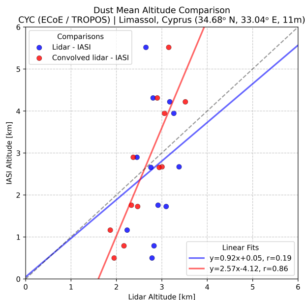
Figure 16. Dust mean altitude comparison, regridded (blue) and convolved (red) lidar vs IASI/MAPIR, for 12 dust cases over Limassol, Cyprus.
