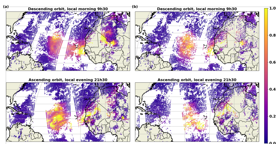
Figure 19. MAPIR IASI-A (a) and IASI-C (b) dust AOD 10 \mu\text{m} for 19 June 2020, morning and overpass separately.
