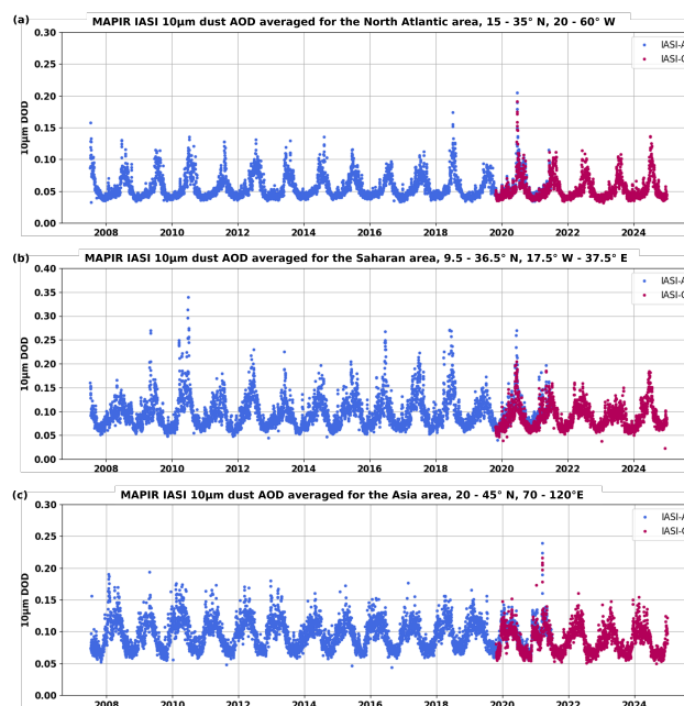
Figure 18. Time series of MAPIR IASI-A and IASI-C dust AOD at 10 \mu\text{m} , averaged daily (combined morning and evening overpasses) for (a) the North Atlantic area, latitude 15 to 35° N, longitude 20 to 60° W, (b) the Sahara area, latitude 9.5 to 36.5° N, longitude 17.5° W to 37.5° E, (c) for Asia, latitude 20 to 45° N, longitude 70 to 120° E.
