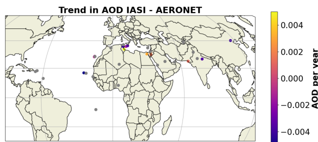
Figure 17. Linear trend in the bias of MAPIR IASI-A versus AERONET solar observations (AOD 550 nm per year). Stations plotted in grey are those included in the analysis but without significant trend at the 95% confidence (p value larger than 0.05).
