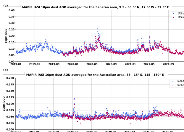
Figure 21. Same as Fig. 18, zoomed on the 2019–2021 years, for (a) the Sahara area, latitude 9.5 to 36.5^\circ N, longitude 17.5^\circ W to 37.5^\circ E, and (b) the Australian area, latitude 35 to 15^\circ S, longitude 115 to 150^\circ E.
