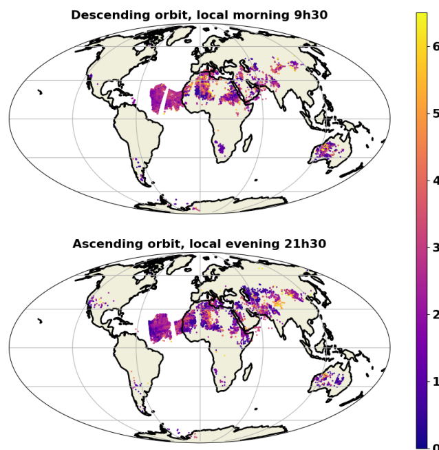
Figure 10. Mean altitude (km above sea level) for MAPIR IASI-A, 19 June 2020.
