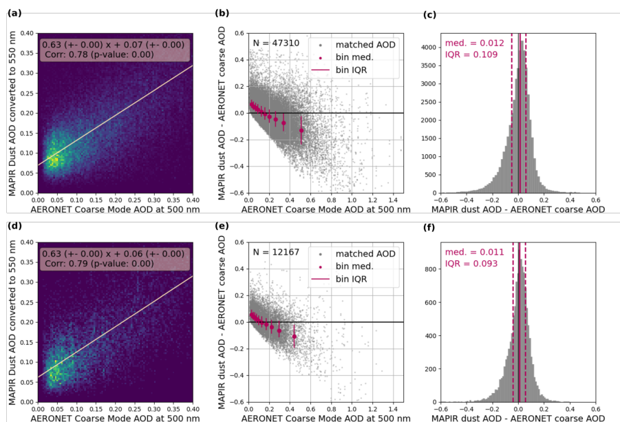
Figure 4. MAPIR v5.1 comparisons for IASI-A (a,b,c) and IASI-C (d,e,f) dust AOD converted to 550 nm against AERONET solar data SDA coarse mode AOD at 500 nm. (a,d) Density plot of AOD, IASI-A versus AERONET, with its linear regression and equation; (b,e) Scatter plot of the MAPIR AOD bias versus the AERONET AOD, with bins of equal number of points. (c,f) Histograms of the MAPIR AOD bias.
