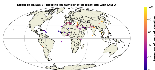
Figure 3. Reduction (in %) of AERONET - IASI-A collocation pairs due to AERONET quality filtering, including rejection of observations with fine mode fraction larger than 0.5.
