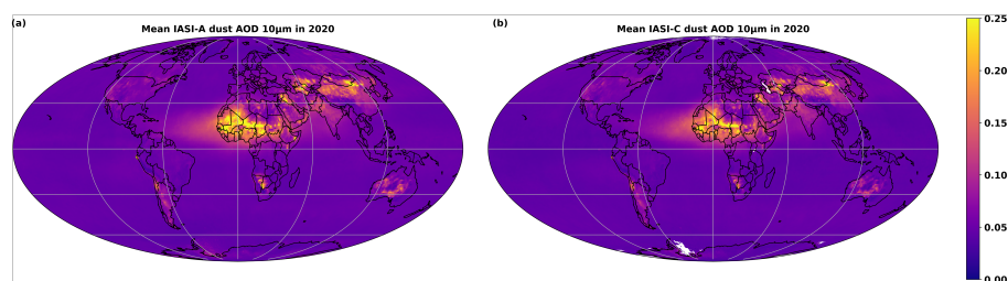
Figure 20. Yearly average of MAPIR IASI-A (a) and IASI-C (b) dust AOD 10\mu\text{m} for 2020.
