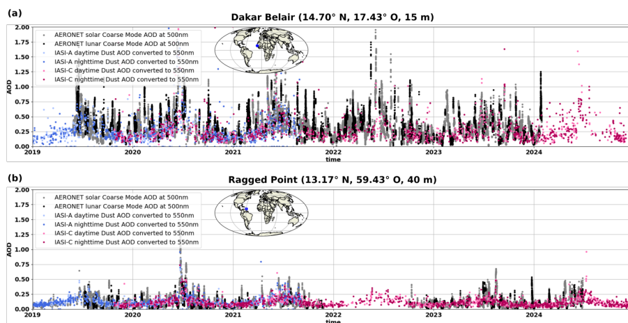
Figure 7. Time series of all AERONET (solar and lunar) SDA coarse mode AOD at 500 nm and of IASI-A and IASI-C dust AOD converted to 550 nm (separated day and night) for the time span with available AERONET data, at (a) the Dakar Belair AERONET station and (b) the Ragged Point station. Note that these are full data series, not only collocations.
