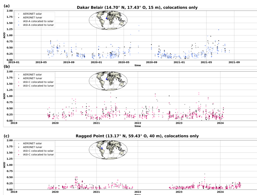
Figure 8. Time series of collocated AERONET (solar and lunar) SDA coarse mode AOD at 500 nm and of (a) IASI-A and (b) IASI-C dust AOD converted to 550 nm (separated day and night), at the Dakar Belair AERONET station, and (c) IASI-C at the Ragged Point station.
