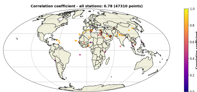
Figure 6. Correlation coefficient between MAPIR v5.1 comparisons for IASI-A dust AOD converted to 550 nm and AERONET solar data SDA coarse mode AOD at 500 nm, for all stations with at least 100 colocations
