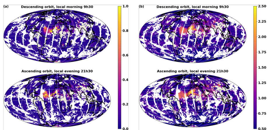
Figure 9. Dust 10\ \mu\text{m} AOD (a) and number of degrees of freedom (DOF, b) for MAPIR IASI-A, 19 June 2020. Morning and evening overpass data are plotted separately
