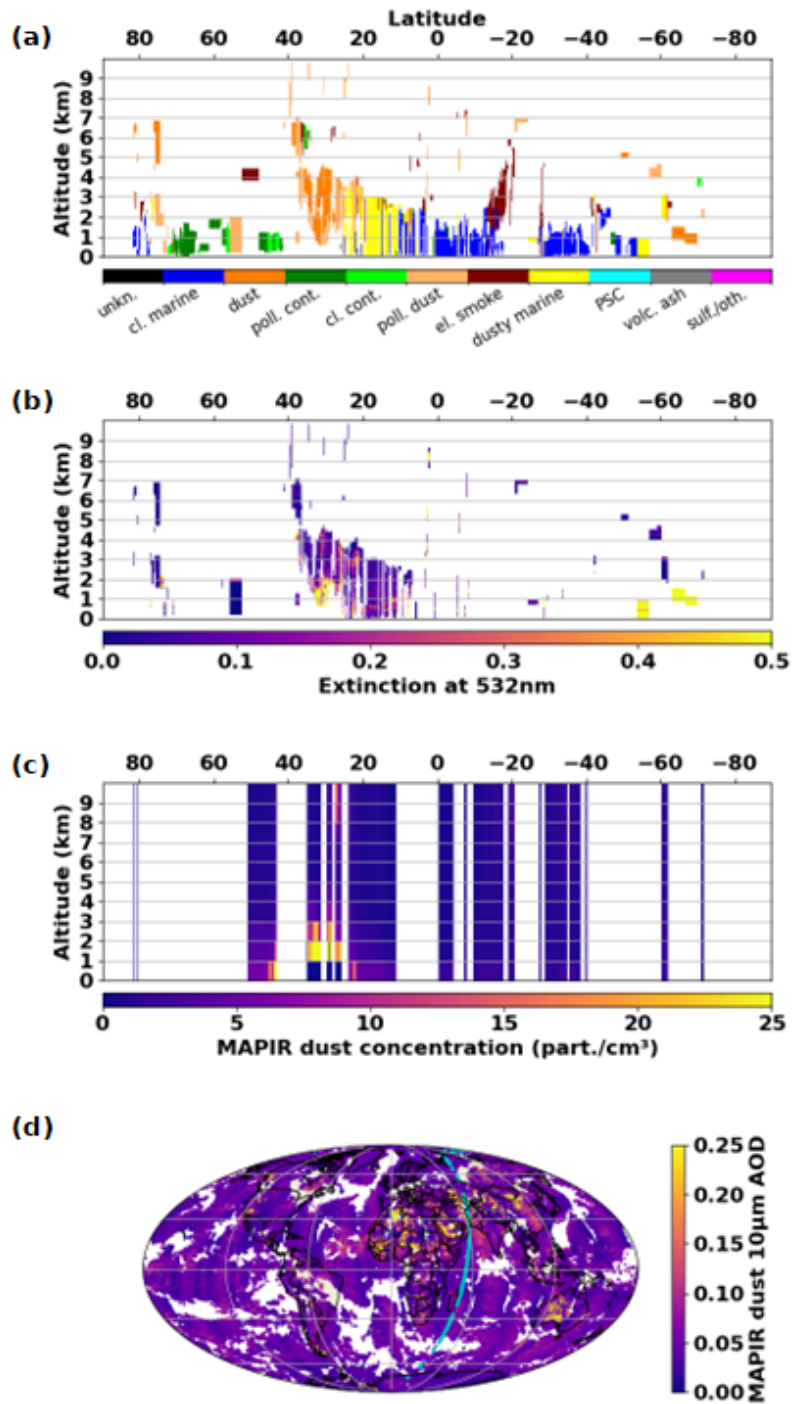
Figure 12. Comparison of CALIOP and IASI-A MAPIR for 28 October 2018, night-time. (a) CALIOP aerosol type; (b) CALIOP 532 nm extinction for the aerosol types "dust", "polluted dust" and "dusty marine"; (c) IASI-A MAPIR dust concentration profile along the selected CALIOP orbit part; (d) IASI-A MAPIR dust AOD (daily average), with the track of CALIOP for the selected orbit part.
