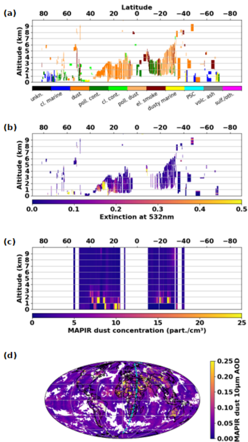
Figure 13. Same as Fig. 12, for a different CALIOP orbit of the same day.
