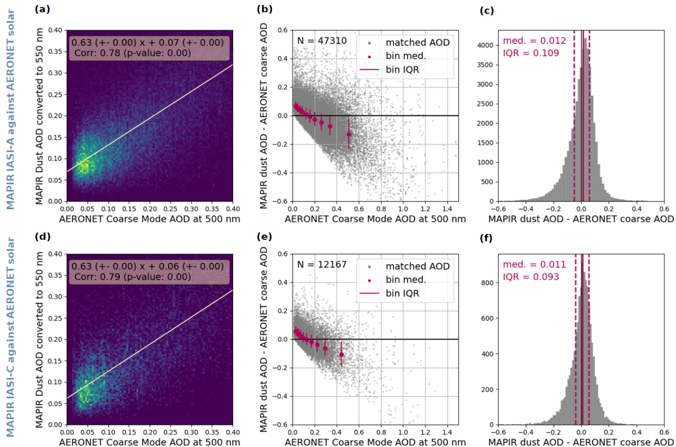
Figure 4. MAPIR v5.1 comparisons for IASI-A (a,b,c) and IASI-C (d,e,f) dust AOD converted to 550 nm against AERONET solar SDA CAOD at 500 nm. (a,d) Density plot of AOD, MAPIR versus AERONET, with its linear regression and equation; (b,e) Scatter plot of the MAPIR AOD bias versus the AERONET AOD, with bins of equal number of points. (c,f) Histograms of the MAPIR AOD bias.
