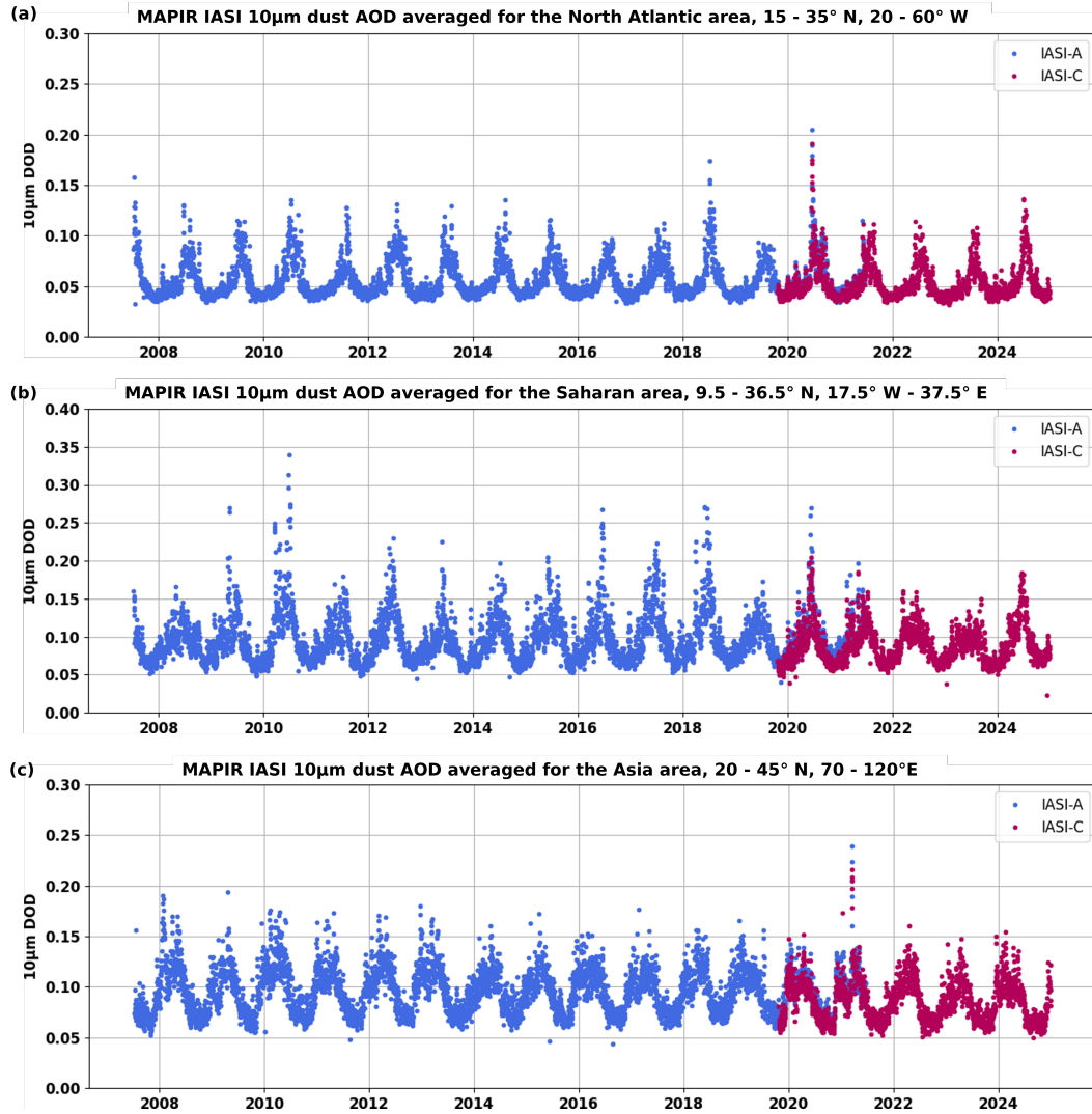
Figure 17. Time series of MAPIR IASI-A and IASI-C dust AOD at 10 \mu\text{m} , averaged daily (combined morning and evening overpasses) for (a) the North Atlantic area, latitude 15 to 35° N, longitude 20 to 60° W, (b) the Sahara area, latitude 9.5 to 36.5° N, longitude 17.5° W to 37.5° E, (c) for Asia, latitude 20 to 45° N, longitude 70 to 120° E.
