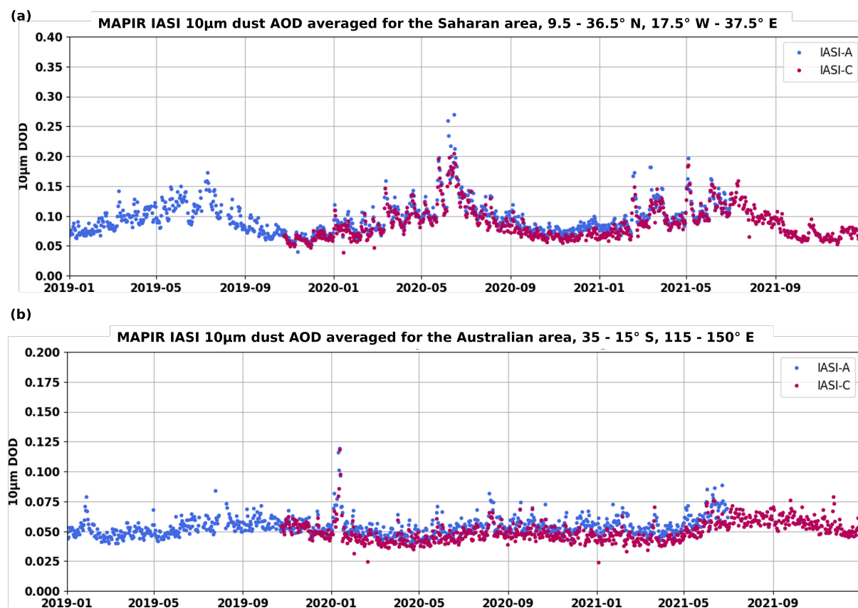
Figure 20. Same as Fig. 17, zoomed on the 2019-2021 years, for (a) the Sahara area, latitude 9.5 to 36.5° N, longitude 17.5° W to 37.5° E, and (b) the Australian area, latitude 35 to 15° S, longitude 115 to 150° E.
