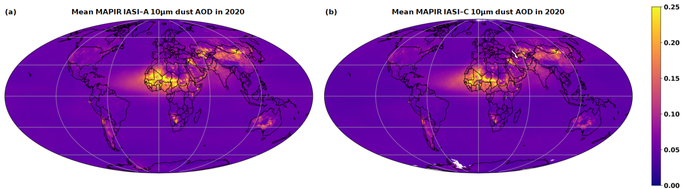
Figure 19. Yearly average of MAPIR IASI-A (a) and IASI-C (b) dust AOD 10 \mu m for 2020.
