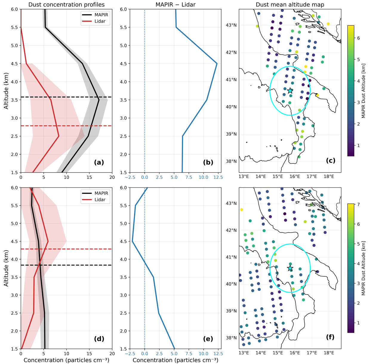
Figure 15. Case study comparison of dust retrievals for Potenza, Italy, on 19 June 2024 (top row; a–c) and 20 June 2023 (bottom row; d–f). Panels (a,d) show vertical dust concentration profiles and mean dust altitude derived from lidar and MAPIR, panels (b,e) show the absolute difference between MAPIR and lidar retrievals, while panels (c,f) show the spatial distribution of MAPIR-derived mean dust altitude.
