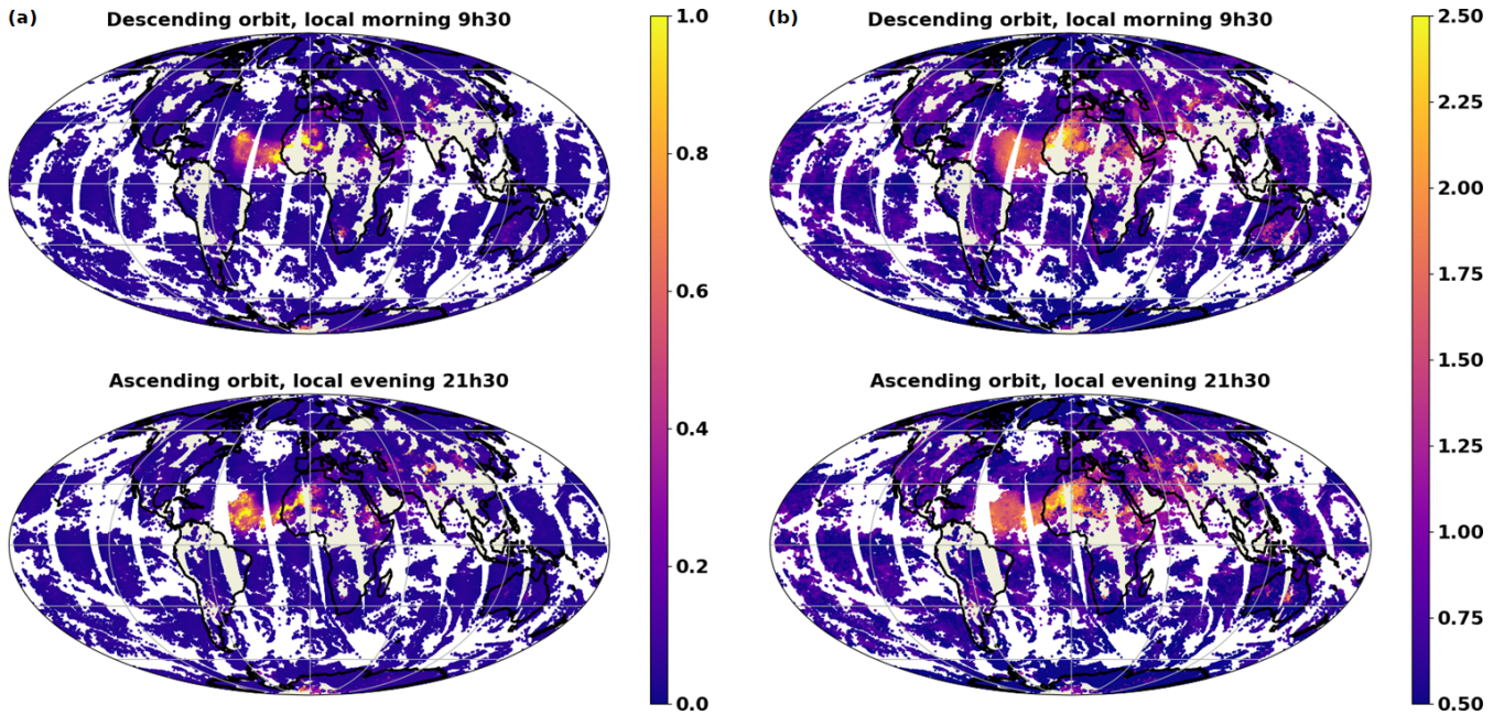
Figure 9. Dust 10\ \mu\text{m} AOD (a) and number of DOF (b) for MAPIR IASI-A, 19 June 2020. Morning and evening overpass data are plotted separately
