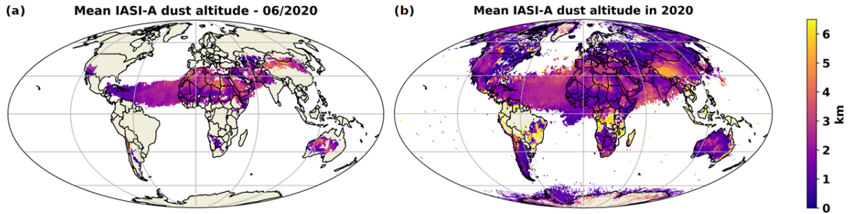
Figure 11. Mean altitude for MAPIR IASI-A averaged over the month of June 2020 (a) and the whole year 2020 (b). Morning and evening overpasses are included.
