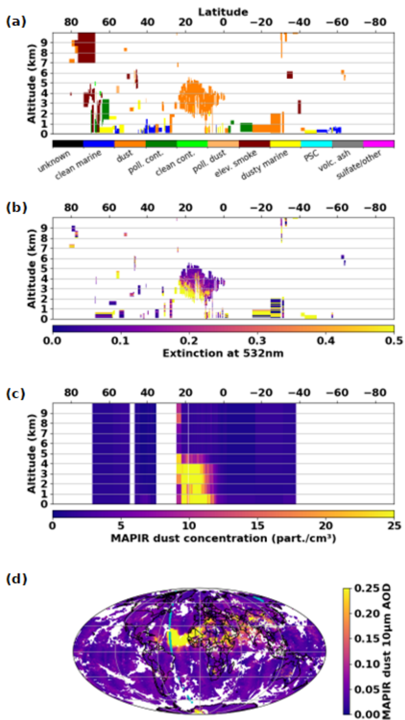
Figure 14. Same as Fig. 12, for an orbit of 19 June 2020 day-time and using IASI-C MAPIR data.
