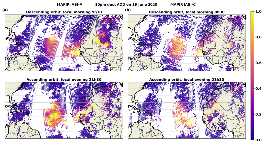
Figure 18. MAPIR IASI-A (a) and IASI-C (b) dust AOD 10 \mu m for 19 June 2020, morning and overpass separately.
