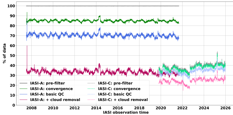
Figure 2. MAPIR v5.1 performance for IASI-A and IASI-C.
