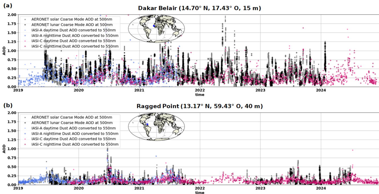
Figure 7. Time series of all AERONET (solar and lunar) SDA coarse-mode-AOD-CAOD at 500 nm and of MAPIR IASI-A and IASI-C dust AOD converted to 550 nm (separated day and night) for the time span with available AERONET data, at (a) the Dakar Belair AERONET station and (b) the Ragged Point station. Note that these are full data series, not only colocations.
