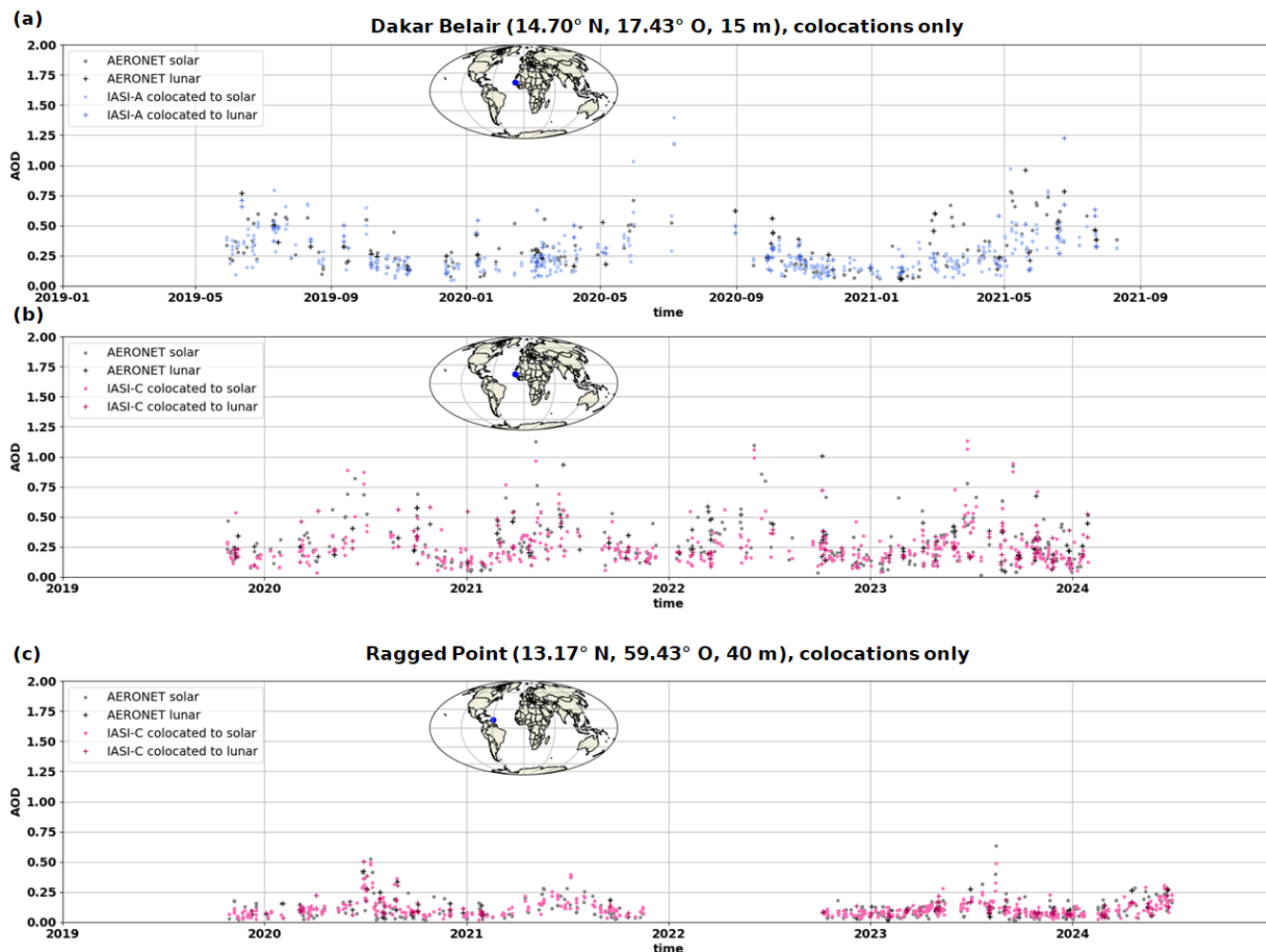
Figure 8. Time series of collocated AERONET (solar and lunar) SDA coarse-mode-AOD CAOD at 500 nm and of MAPIR (a) IASI-A and (b) IASI-C dust AOD converted to 550 nm (separated day and night), at the Dakar Belair AERONET station, and (c) IASI-C at the Ragged Point station.
