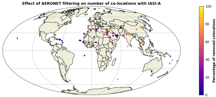
Figure 3. Reduction (in %) of AERONET - MAPIR IASI-A collocation pairs due to AERONET quality-filtering, including rejection of observations with fine mode fraction larger than 0.5.
