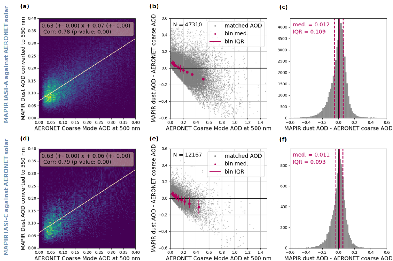
Figure 4. MAPIR v5.1 comparisons for IASI-A (a,b,c) and IASI-C (d,e,f) dust AOD converted to 550 nm against AERONET solar data-SDA coarse-mode-AOD-CAOD at 500 nm. (a,d) Density plot of AOD, IASI-A-MAPIR versus AERONET, with its linear regression and equation; (b,e) Scatter plot of the MAPIR AOD bias versus the AERONET AOD, with bins of equal number of points. (c,f) Histograms of the MAPIR AOD bias.
