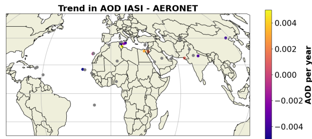
Figure 16. Linear trend in the bias of MAPIR IASI-A versus AERONET solar observations (AOD 550 nm per year). Stations plotted in grey are those included in the analysis but without significant trend at the 95% confidence (p value larger than 0.05).
