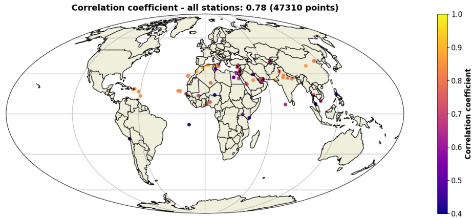
Figure 6. Correlation coefficient between MAPIR v5.1 comparisons for IASI-A dust AOD converted to 550 nm and AERONET solar data SDA coarse-mode AOD CAOD at 500 nm, for all stations with at least 100 colocations
