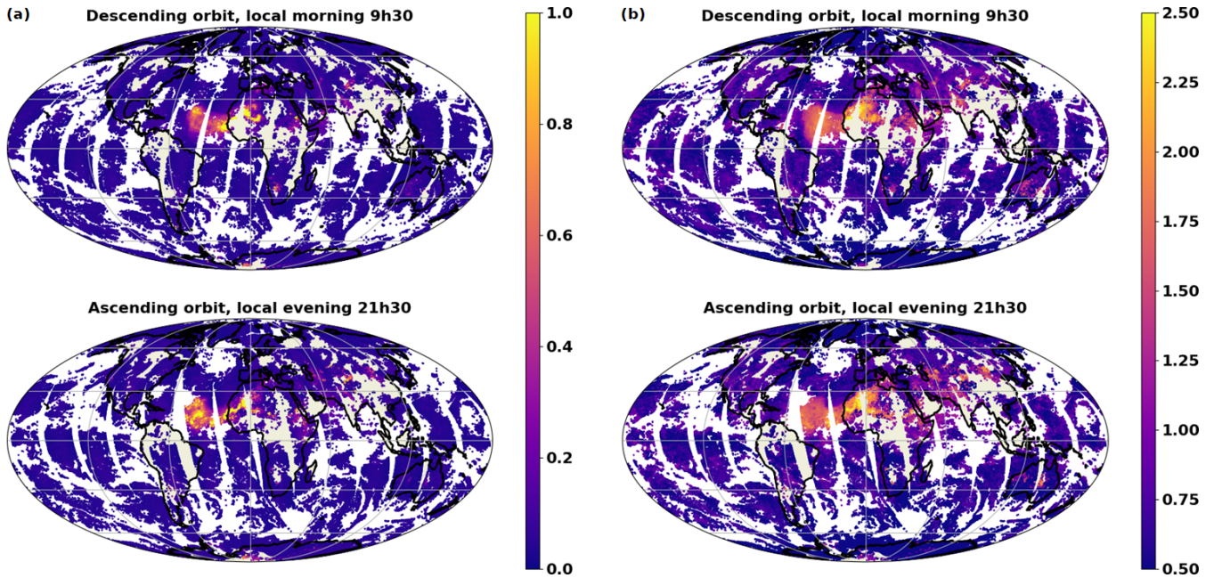
Figure 9. Dust 10\ \mu\text{m} AOD (a) and number of degrees-of-freedom (DOF) (b) for MAPIR IASI-A, 19 June 2020. Morning and evening overpass data are plotted separately
