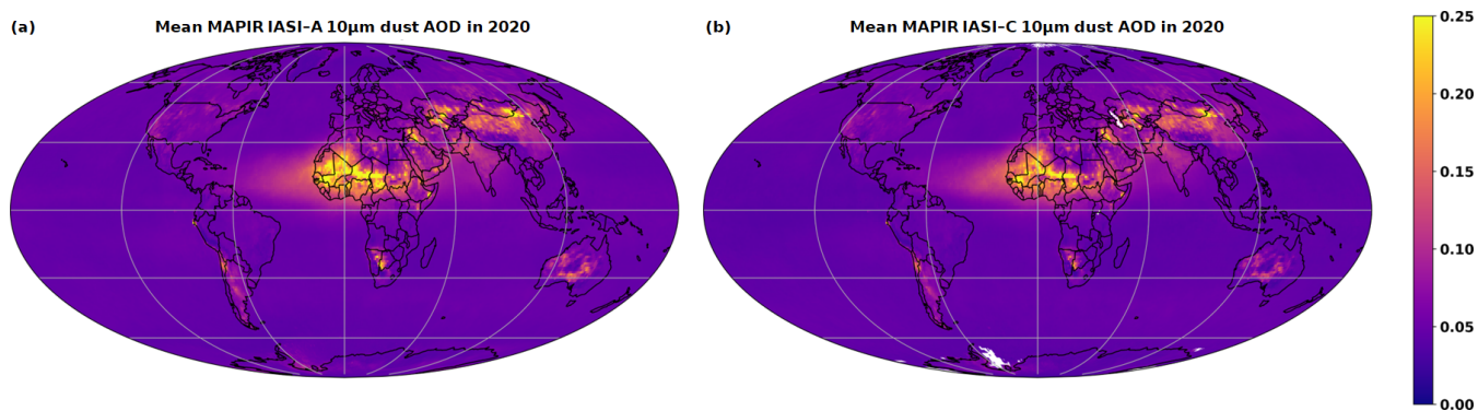
Figure 19. Yearly average of MAPIR IASI-A (a) and IASI-C (b) dust AOD 10 \mu m 10 \mu m for 2020.
