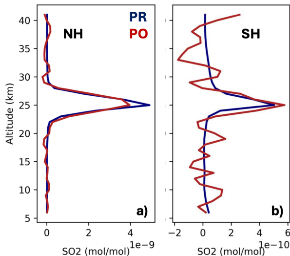
Figure 5: Average vertical SO 2 profiles, PR (blue lines) and CAIRT PO (red lines), for the two SO 2 injection points visible in Fig. 4b-c (panel a: injection point in the NH, at 15°N; panel b: injection point in the SH, at 15°S). The total SO 2 mass intercepted by the CAIRT POs, for the two injection points, is: panel a: 3.1 tonnes (PR: 3.4 tonnes), and panel b: 0.4 tonnes (PR: 0.5 tonnes).
