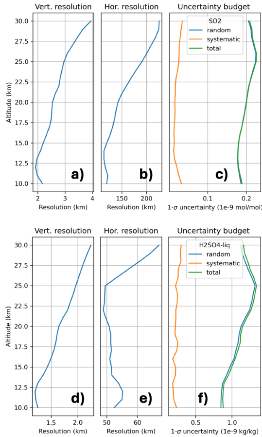
250 Figure 3: Vertical profile of the vertical (panels a and d) and horizontal resolutions (panels b and e) and of the uncertainty budget (panels c and f) for SO 2 (panels a-c) and SA CAIRT PO retrievals (panels d-f). In panels c and f, the blue, orange and green curves represent the random, systematic and total uncertainties, respectively. The vertical and horizontal resolution and the uncertainty budget, for both SO 2 and SA, are representative of individual retrievals with 100-km across-track binning.
