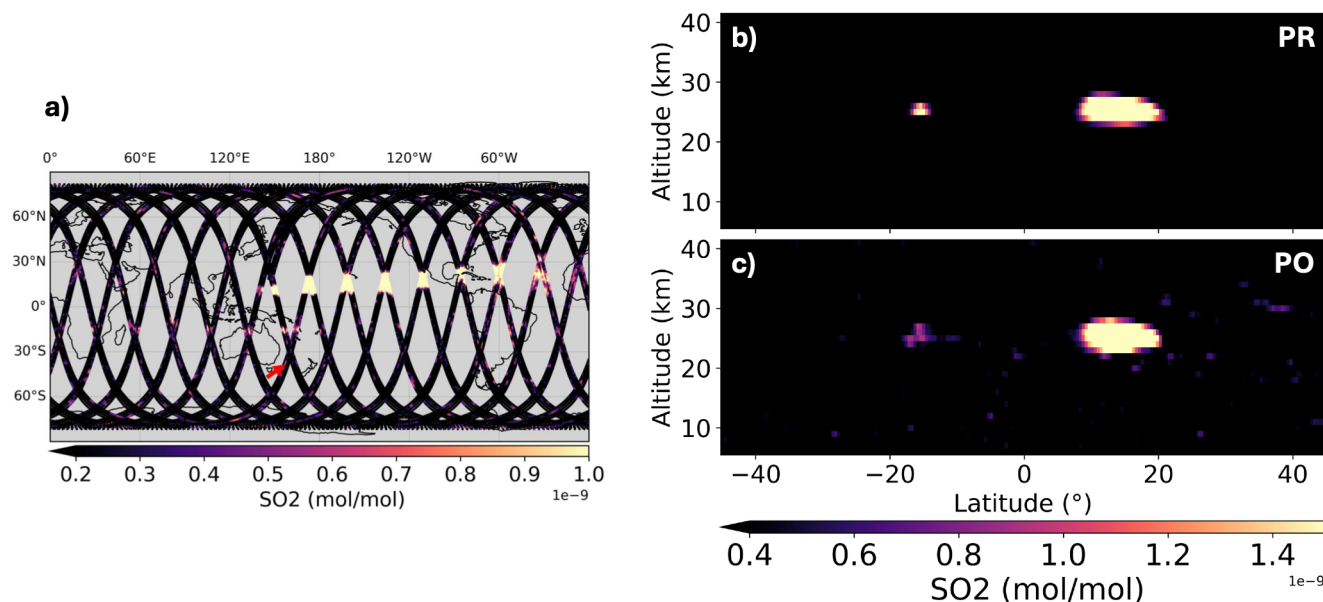
270 Figure 4: (a) CAIRT POs of the SO 2 mixing ratio for February 2034, at 25 km altitude. (b-c) Across-track average PR (panel b) and 275 CAIRT PO (panel c) of the SO 2 vertical profiles, for the orbit segment individuated with a red arrow in panel a.
