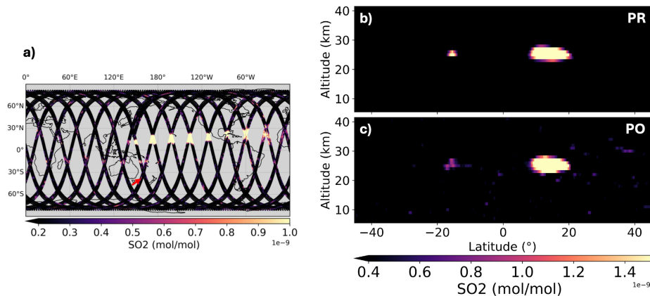
Figure 4: (a) CAIRT POs of the SO 2 mixing ratio for February 2034, at 25 km altitude. (b-c) Across-track average PR (panel b) and CAIRT PO (panel c) of the SO 2 vertical profiles, for the orbit segment individuated with a red arrow in panel a.
