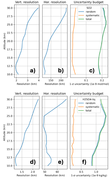
255 Figure 3: Vertical profile of the vertical (panels a and d) and horizontal resolutions (panels b and e) and of the uncertainty budget (panels c and f) for SO 2 (panels a-c) and SA CAIRT PO retrievals (panels d-f). In panels c and f, the blue, orange and green curves represent the random, systematic and total uncertainties, respectively. The vertical and horizontal resolution and the uncertainty budget, for both SO 2 and SA, are representative of individual retrievals with 100-km across-track binning.
