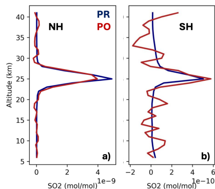
Figure 5: Average vertical \text{SO}_2 profiles, PR (blue lines) and CAIRT PO (red lines), for the two \text{SO}_2 injection points visible in Fig. 4b-c (panel a: injection point in the NH, at 15^\circ\text{N} ; panel b: injection point in the SH, at 15^\circ\text{S} ). The total \text{SO}_2 mass intercepted by the CAIRT POs, for the two injection points, is: panel a: 3.1 tonnes (PR: 3.4 tonnes), and panel b: 0.4 tonnes (PR: 0.5 tonnes).
