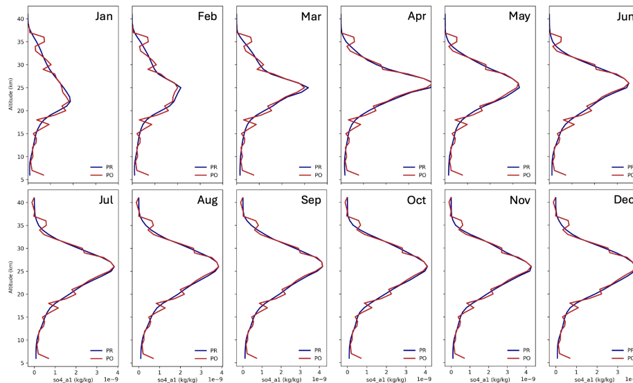
345 Figure 8: Global average vertical profiles of nucleation mode SA concentration, for CAIRT POs based on the Geo SSP5-34-OS 2.0 PR scenario, as monthly means from January to December 2034 (PR in blue lines and CAIRT POs in red lines).
