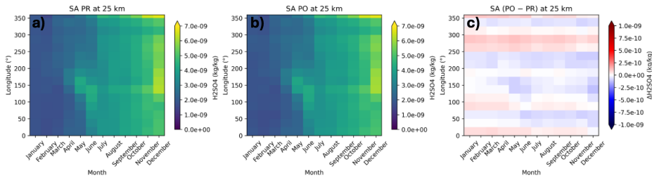
Figure 6: Time series of monthly average meridional mean total SA mass concentration at 25 km altitude, for the Geo SSP5-34-OS 2.0 PR scenario (panel a) and corresponding CAIRT PO (panel b), for year 2034. The absolute difference of PO and PR monthly average meridional means are shown in panel c.
