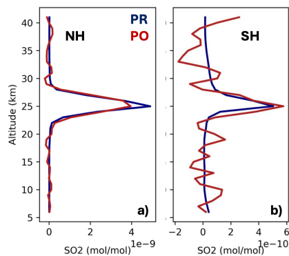
Figure 5: Average vertical \text{SO}_2 profiles, PR (blue lines) and CAIRT PO (red lines), for the two \text{SO}_2 injection points visible in Fig. 4b-c (panel a: injection point in the NH, at 15^\circ\text{N} ; panel b: injection point in the SH, at 15^\circ\text{S} ). The total \text{SO}_2 mass intercepted by the CAIRT POs, for the two injection points, is: panel a: 3.1 tonnes (PR: 3.4 tonnes), and panel b: 0.4 tonnes (PR: 0.5 tonnes).
