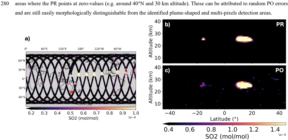
Figure 4: (a) CAIRT POs of the SO 2 mixing ratio for February 2034, at 25 km altitude. (b-c) Across-track average PR (panel b) and CAIRT PO (panel c) of the SO 2 vertical profiles, for the orbit segment individuated with a red arrow in panel a. 285 Figure 5 shows the average vertical PR and CAIRT PO SO 2 profiles, around the injection points at 15°S (Fig. 5a) and 15°N (Fig. 4b), individuated in Figs. 4b-c. It is important to stress that what is shown in Figs. 1a-c and Figs. 4-5 are very weak initial SAI interventions, in the simulated SAI protocol of Geo SSP5-34-OS 2.0 PR scenario. The total SO 2 mass values intercepted by this specific CAIRT orbit segment, in the area impacted by the two injection points, is 0.5 tonnes (injection at 15°S, Fig. 5a) and 3.4 tonnes (injection at 15°N, Fig. 5b), respectively. More in general, the total SO 2 injected mass in the PR scenario, cumulated until end February 2034 (SO 2 PR of Fig. 1c) does not exceed a few hundreds tonnes. As mentioned in the Introduction, these injections can be seen as analogues of “near-term” to “mid-term” experiments, i.e. scenarios considered
