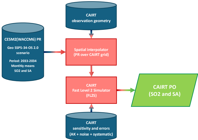
275 Figure 2: Scheme of the method used in this work to generate CAIRT PO.
