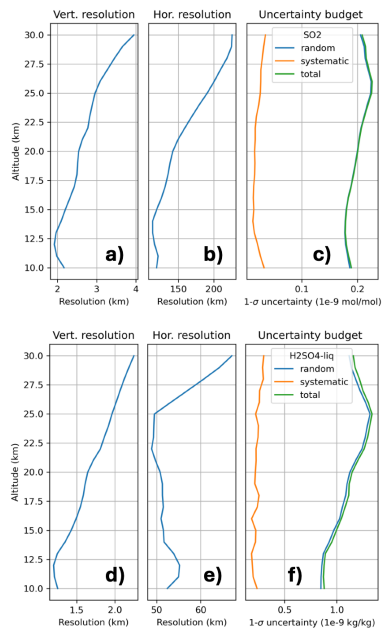
Figure 3: Vertical profile of the vertical (panels a and d) and horizontal resolutions (panels b and e) and of the uncertainty budget (panels c and f) for \text{SO}_2 (panels a-c) and SA CAIRT PO retrievals (panels d-f). In panels c and f, the blue, orange and green curves
