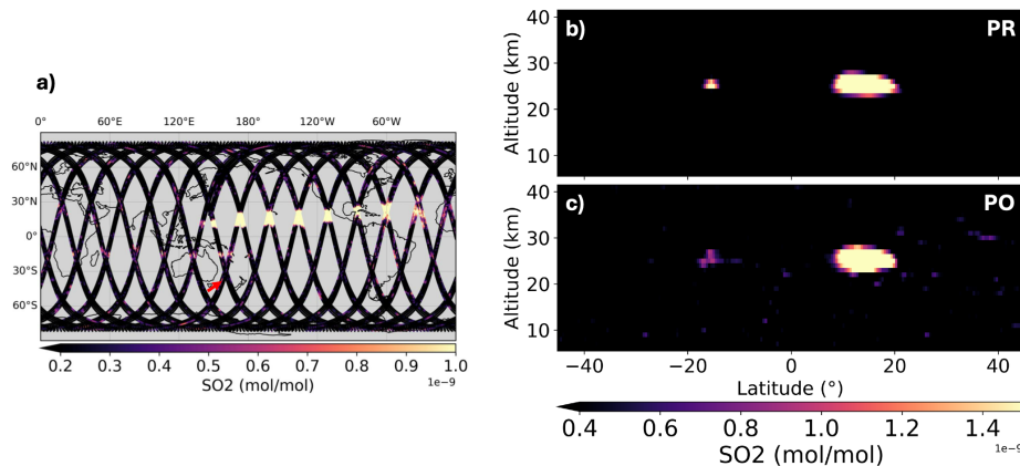
Figure 4: (a) CAIRT POs of the SO 2 mixing ratio, for February 2034, at 25 km altitude. (b-c) Across-track average PR (panel b) and CAIRT PO (panel c) of the SO 2 vertical profiles, for the orbit segment individuated with a red arrow in panel a.
