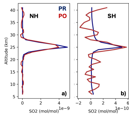
Figure 5: Average vertical SO 2 profiles, PR (blue lines) and CAIRT PO (red lines), for the two SO 2 injection points visible in Fig. 4b-c (panel a: injection point in the NH, at 15°N; panel b: injection point in the SH, at 15°S). The total SO 2 mass intercepted by the CAIRT POs, for the two injection points, is: panel a: 3.1 tonnes (PR: 3.4 tonnes), and panel b: 0.4 tonnes (PR: 0.5 tonnes).
