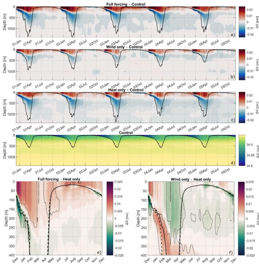
390 Figure 5. Response of salinity to tip jet forcing in the convective region. (a–d) Temporal evolution of area-averaged salinity anomalies (psu): (a) full-forcing – control, (b) wind-only – control, (c) heat-only – control, (d) control reference. Black curves show the MLD. Annual mean salinity differences: (e) full forcing – heat-only, (f) wind-only – heat-only. The black solid line shows annual mean MLD in the full forcing (e) or wind-only (f) and the dashed one shows the MLD for heat-only run. Thin dotted lines mark depths where salinity differences between the runs are significant at the 95 % confidence level.
