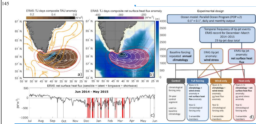
Figure 1. Study domain, composite tip jet (TJ) forcing fields, and definition of analysis region. (a) ERA5 composite of wind stress (TAU) anomalies on tip jet days (relative to the 1969–2022 climatology; Fedorov et al., 2025). The red outline marks the region where
