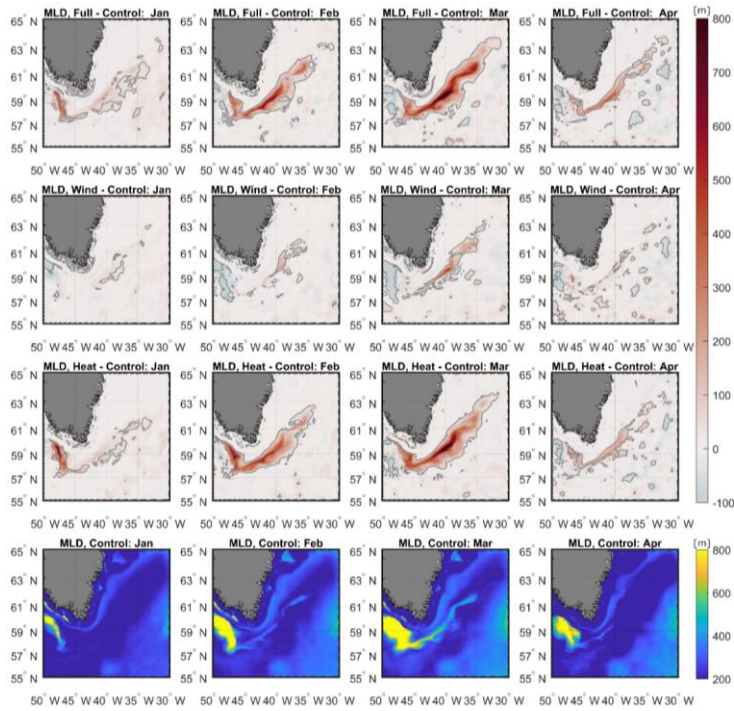
275 Figure 2. Monthly mixed layer depth (MLD) differences relative to the control run in the Irminger Sea. Columns represent January–April (left to right). Rows show: (top) full-forcing minus control, (second) wind-only minus control, (third) heat-only minus control, and (bottom) the corresponding monthly mean MLD from the control run. Grey contours indicate regions where MLD differences are significant at the 95 % confidence level.
