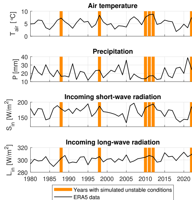
Figure 4. Climatic conditions during summer (July-August, 1980-2022) based on ERA5 data and years with simulated slope instability. Note: incoming short-wave and long-wave radiation are for horizontal surfaces.
