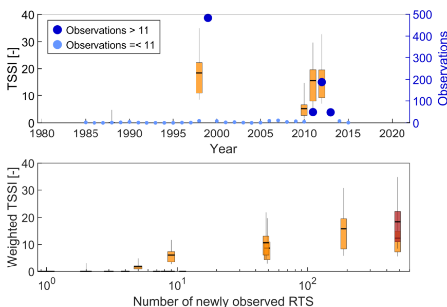
Figure 5. (a) Simulated TSSI (1980-2022) and the number of newly observed RTS in the study area (1985-2015). Many new RTS are detected in the satellite imagery in the year following their initiation (Lewkowicz and Way, 2019), explaining the time lag with the TSSI. (b) Log-linear relationship between weighted TSSI (taking into account the time lag - see text) and the number of newly observed RTS in the study area. The TSSI relating to the highest number of RTS in 1999 is shown as weighted between the years of 1998 and 1999 (orange) and entirely based on 1998 (red).
