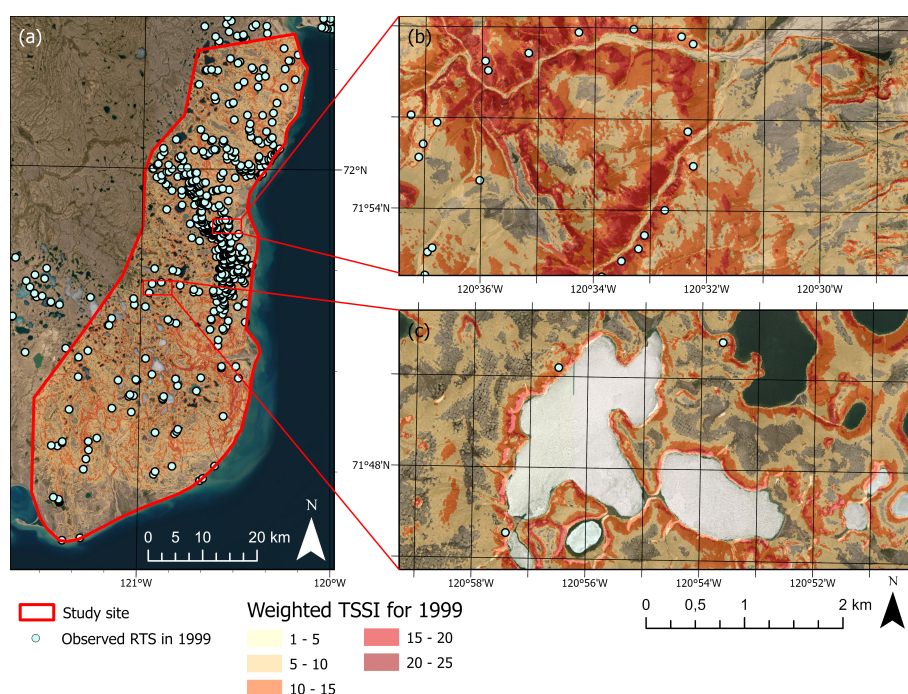
Figure 7. The simulated weighted Thawing Slope Stability Index (TSSI) and newly observed initiated retrogressive thaw slumps (RTS) in 1999 for the entire study area. Sources: Esri, TomTom, Garmin, FAO, NOAA, USGS, © OpenStreetMap contributors, and the GIS User Community | Powered by Esri.
