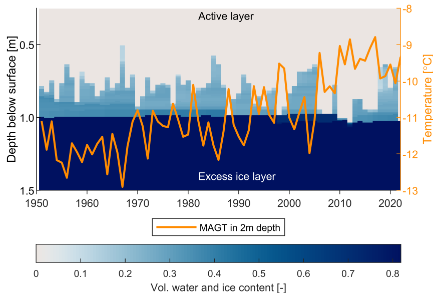
Figure 3. Simulated mean annual ground temperature (MAGT) at 2 m depth and minimum annual volumetric water and ice content (1950-2022). The latter is only shown for grid cells with continuously frozen conditions for the respective year to visualize the depth of the active layer. Both parameters are the average values for the 20 clusters weighted by cluster area.
