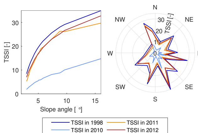
Figure 6. Relationship between the simulated TSSI for years with median positive values and (a) slope angle and (b) aspect. Soil properties were assumed to be the same in all clusters. Note: Years with a mean TSSI of zero are not shown.
