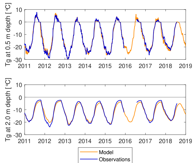
Figure A1. Observed and simulated ground temperatures T_g at 0.5 m and 2.0 m depth in Aulavik Nationalpark, Banks Island.
