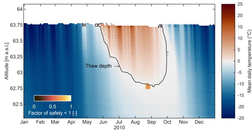
Figure 4. Simulated mean daily ground temperature in 2010 for a cluster with a north-facing slope and a slope angle of 3.4^{\circ}\text{C} . The figure illustrates that unstable conditions occur at the top of the permafrost, where ground temperatures are just below 0^{\circ}\text{C} .
