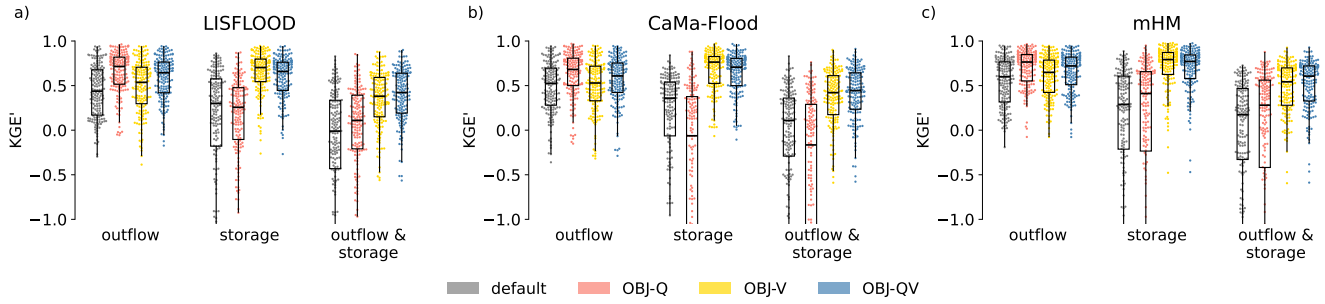
Figure 5. Comparison of the model performance depending on the variable(s) targeted in the calibration. The panels correspond to the three reservoir routines that were calibrated: a) LISFLOOD, b) CaMa-Flood and c) mHM. Within each panel, three groups of box plots show the performance in terms of outflow, storage, and both variables together. Four parameter sets are compared —default parameters, calibration of outflow (OBJ-Q), storage (OBJ-V) and both variables (OBJ-QV)— indicated by colors. The dots represent individual reservoirs, indicating the distribution of the overall performance.
