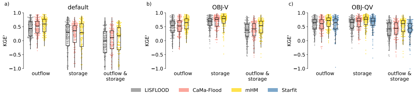
Figure 6. Comparison of the model performance depending on the reservoir routine. The panels corresponds correspond to three of the experiments: a) default values parameters , b) calibration of storage (OBJ-V), c) bivariate calibration of outflow and storage (OBJ-QV). Within each panel, three groups of box plots show the performance in terms of outflow, storage, and both variables together. Four reservoir routines are compared— LISFLOOD, CaMa-Flood, mHM and STARFIT— indicated by colors. The dots represent individual reservoirs, indicating the distribution of overall performance.
