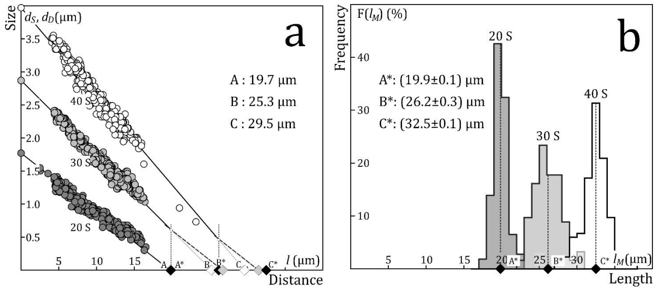
Figure 3. Results of the Kr-track length and size measurements. (a) Diamond sizes ( d_D ) plotted against distance along the track ( l = l_D / \cos(\frac{1}{4}\pi) ) for 20 s (dark), 30 s (light), and 40 s (white) immersion. The intercepts ( d_s ) at l = 0 are the average D_{par} . The solid lines are geometric mean regression lines anchored at d_s . The white diamonds at A (20 s; hidden), B (30 s), and C (40 s) are the intersections ( l_I ) of the regression lines with the l -axis. The black diamonds at A* (20 s), B* (30 s), and C* (40 s) are the corresponding measured lengths ( l_M ; Figure 3b). The dashed lines and grey diamonds ( l_E ) are extrapolations of the 30 s, and 40 s values at A* and B*, assuming that the unetched sections beyond A* and B* etch at the rate calculated from the 20-s data (b) Histograms of the measured track lengths ( l_M = l_T / \cos(\frac{1}{4}\pi) ) for 20 s, (20 + 10) s, and (30 + 10) s etching in 5.5 M \text{HNO}_3 at 21 °C. A*, B*, and C* are the mean lengths plotted in (a) (black symbols).
