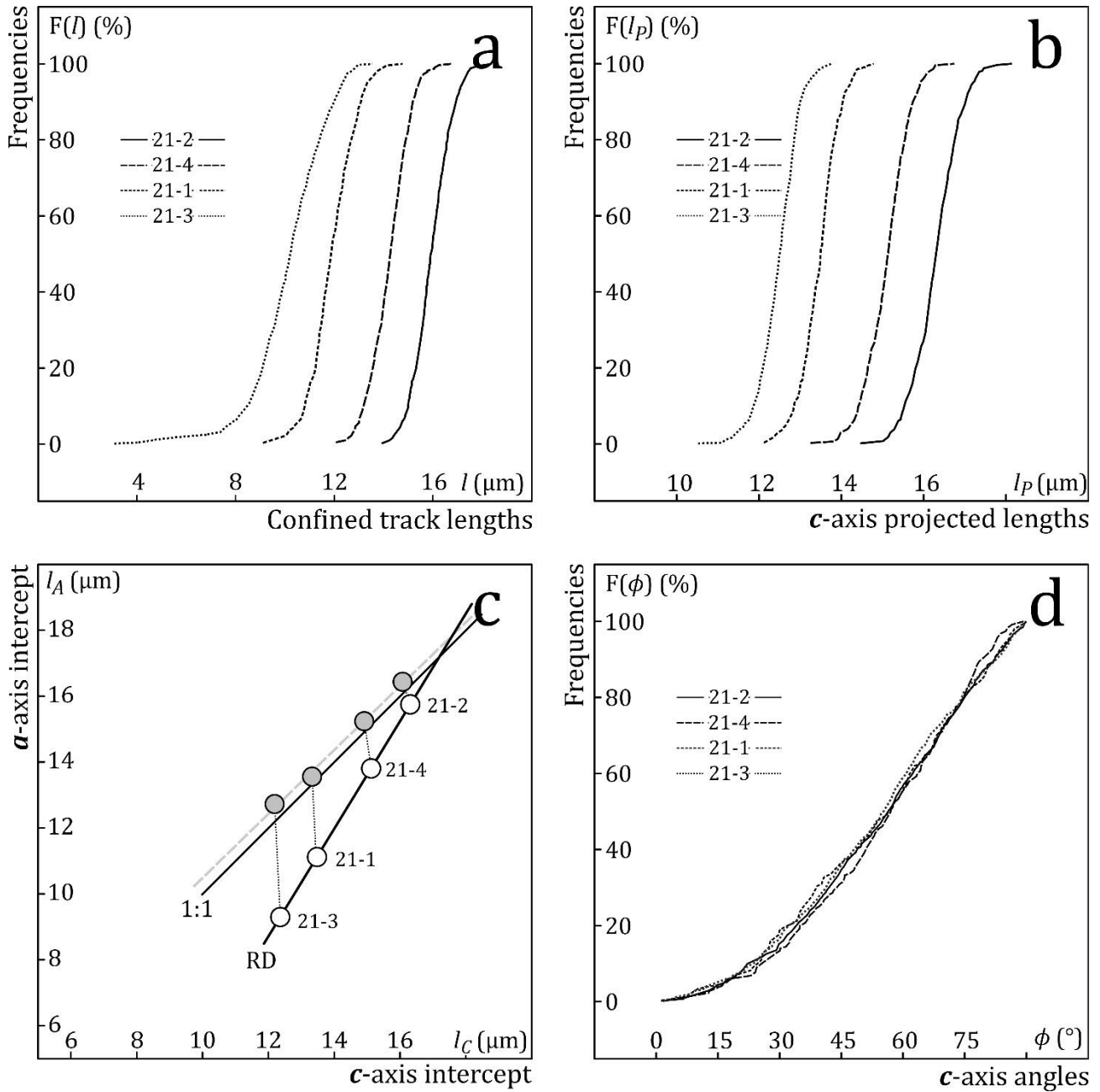
178 Figure 5. (a) Cumulative frequencies of the lengths ( l ) of horizontal induced confined tracks in prism faces 179 of four Durango apatites with increasing degrees of annealing, distributed as part of an inter-lab experi- 180 ment (Ketcham et al., 2015; 21-2: unannealed; 21-4: annealed 10 h at 240 ^\circ\text{C} ; 21-1: annealed 10 h at 288 181 ^\circ\text{C} ; 21-3: annealed 10 h at 310 ^\circ\text{C} ). (b) Cumulative frequencies of the c -axis projected lengths ( l_p ). (c) The 182 a -axis ( l_A ) vs. c -axis intercepts ( l_C ) of ellipses fitted to the length ( l ) vs. c -axis angle ( \phi ) data (white; RD: l_A 183 = 1.632 l_C - 10.879; empirical relationship of Donelick et al., 1999), and of regression lines fitted to the c - 184 axis projected length ( l_p ) vs. c -axis angle ( \phi ) (grey; 1:1: isotropic line: l_A = l_C ); (d) cumulative frequencies 185 of the c -axis angles.
