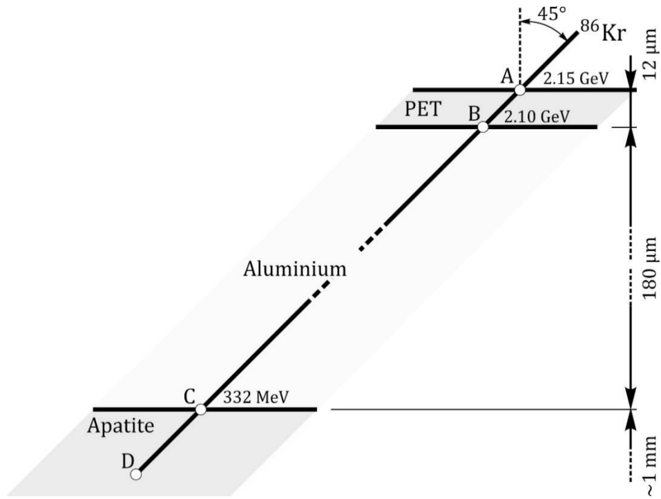
64 Figure 1. Kr irradiation: a prism section of an unannealed single Durango apatite is covered with a 180 65 \mu\text{m} Al degrader and a 12 \mu\text{m} PET film, and irradiated perpendicular to the apatite c -axis and at \frac{1}{4}\pi dip 66 angle with 25.0 \text{ MeV}\cdot\text{amu}^{-1} \text{ }^{86}\text{Kr} . The samples were etched in 5.5 M \text{HNO}_3 at 21 ^\circ\text{C} for 20 s + 10 s + 10 s 67 to reveal the tracks.
