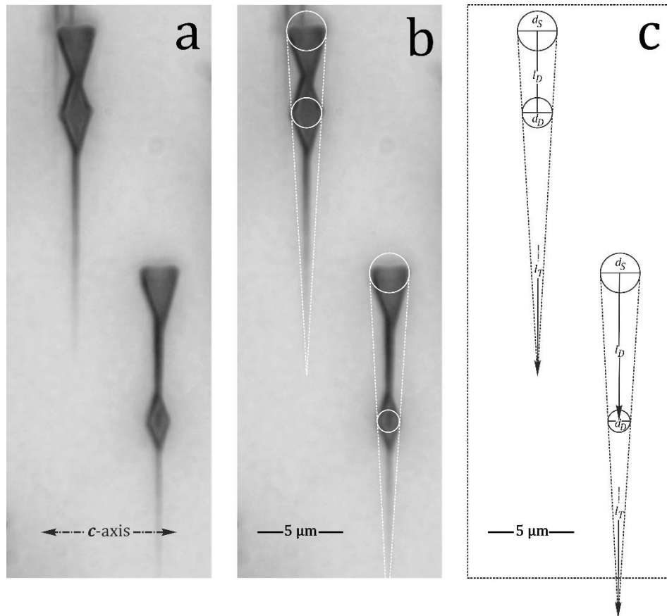
68 Figure 2. Compressed image stack of Kr-tracks perpendicular to the c -axis, intersecting an apatite prism 69 face (a, b); their measurements are shown in (c): d_s and d_b are the diameters of circles tangent to the out- 70 side edges of the triangle- and diamond-shaped etch figures at their intersections with the surface and 71 with a crack; l_D is the distance between their centres, and l_T the measured distance to the end of the etched 72 section.
