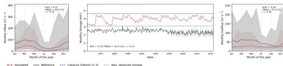
Figure B-3: Monthly inflow climatology (left), storage (center), and outflow climatology (right) for two reservoirs where storage performance was significantly degraded by an initial storage condition set above actual operational levels. Reference observations also show high variability across datasets. Shaded areas in climatology plots represent \pm 1.5 standard deviations; shaded areas in storage panels indicate the range between maximum and minimum reported values across datasets.
