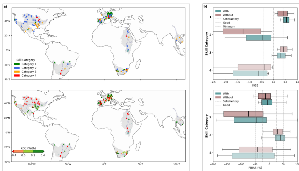
Figure 8: Monthly streamflow performance assessment. Box a) shows the spatial distribution of stations with their corresponding skill category (top) and the KGE value of the model with new implementations (bottom). Box b) shows the distribution of performance per skill categories for KGE (top) and PBIAS (bottom) with and without new implementations, as well as the performance classification thresholds.
