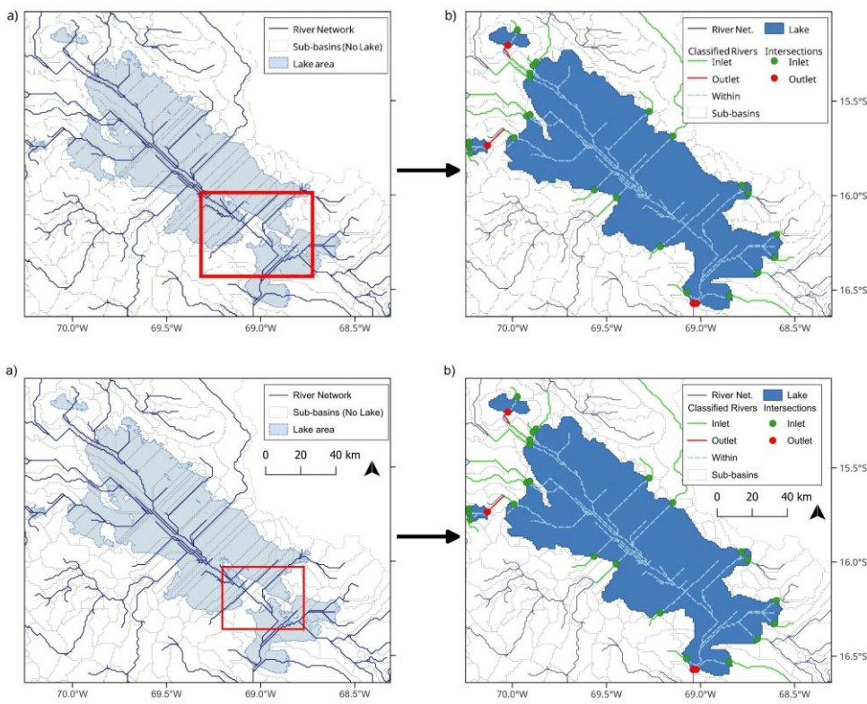
Figure 4: Example of Lake Titicaca in the model structure, a) before network resolution integration process, and b) after resolution integration, showing classified river network elements and points of intersection at the water body limits to define inlets and outlets. Rivers classified as “Within” are eventually excluded from the model structure. The area marked in red on box a) represents the Lago Menor division, an example where complex topography leads to a network in which the lake cannot be integrated without the new resolution integration approach.
