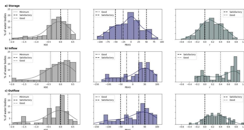
Figure 5: Distribution of KGE, PBIAS, and R related to model performance for monthly mean a) storage, b) inflow, and c) outflow, using normalized histograms expressed as a percentage of evaluated water bodies for the corresponding variable. A kernel density estimate (KDE) curve is overlaid on each histogram to provide a continuous representation of the underlying probability distribution. Vertical reference lines indicate the established adequacy classifications for performance thresholds.
