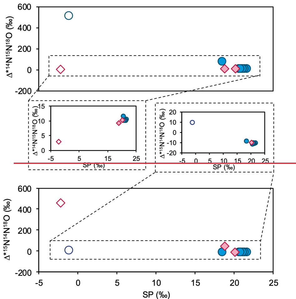
Figure 4: Convergence of isotopic parameters on a common composition. Starting materials (hollow symbols) that bracket the expected equilibrium composition in \Delta^{*14}\text{N}^{15}\text{N}^{18}\text{O} , \Delta^{*15}\text{N}^{14}\text{N}^{18}\text{O} , and SP were heated over activated \gamma\text{-Al}_2\text{O}_3 and are observed to converge on a narrow range in all parameters (filled symbols). Zoomed plots (dashed insets) show that this convergence is observed even over finer scales in \Delta^{*14}\text{N}^{15}\text{N}^{18}\text{O} and \Delta^{*15}\text{N}^{14}\text{N}^{18}\text{O} for the complementary isotopologues to the ones specifically spiked into the starting materials used.
