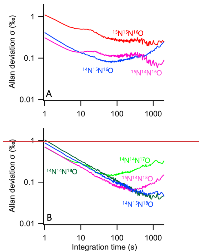
Figure 2: Allan-Werle deviation plots for isotopologues measured by QCL1 (Panel A) and QCL2 (Panel B).
