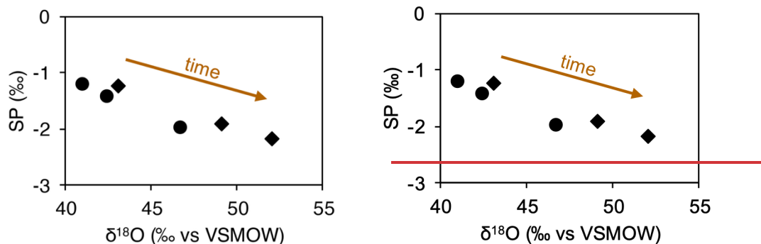
Figure 8: Coevolution of SP and \delta^{18}\text{O} over the course of thermal decomposition. Diamonds represent \Delta^{*14}\text{N}^{15}\text{N}^{18}\text{O} -spiked starting material, while circles represent natural abundance \text{N}_2\text{O} .
