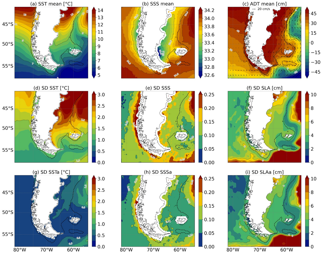
Figure 2: Mean fields of SST (a), SSS (b), and ADT (c) and their standard deviations. Panels d, e and f show the standard deviation of the low-pass filtered time series with respect to the mean fields, thus including seasonal variability. Panels g, h, and i display the standard deviation of the anomalies after removing the annual signal. Contour intervals for the mean and standard deviations are 0.5 and 0.25°C (SST), 0.1 and 0.05 (SSS), and 5 and 1 cm (ADT). The black arrows in panel c represent the mean geostrophic velocity vectors calculated from the ADT (scale shown in panel c). The black dashed line in all maps indicates the 200 m isobath.
