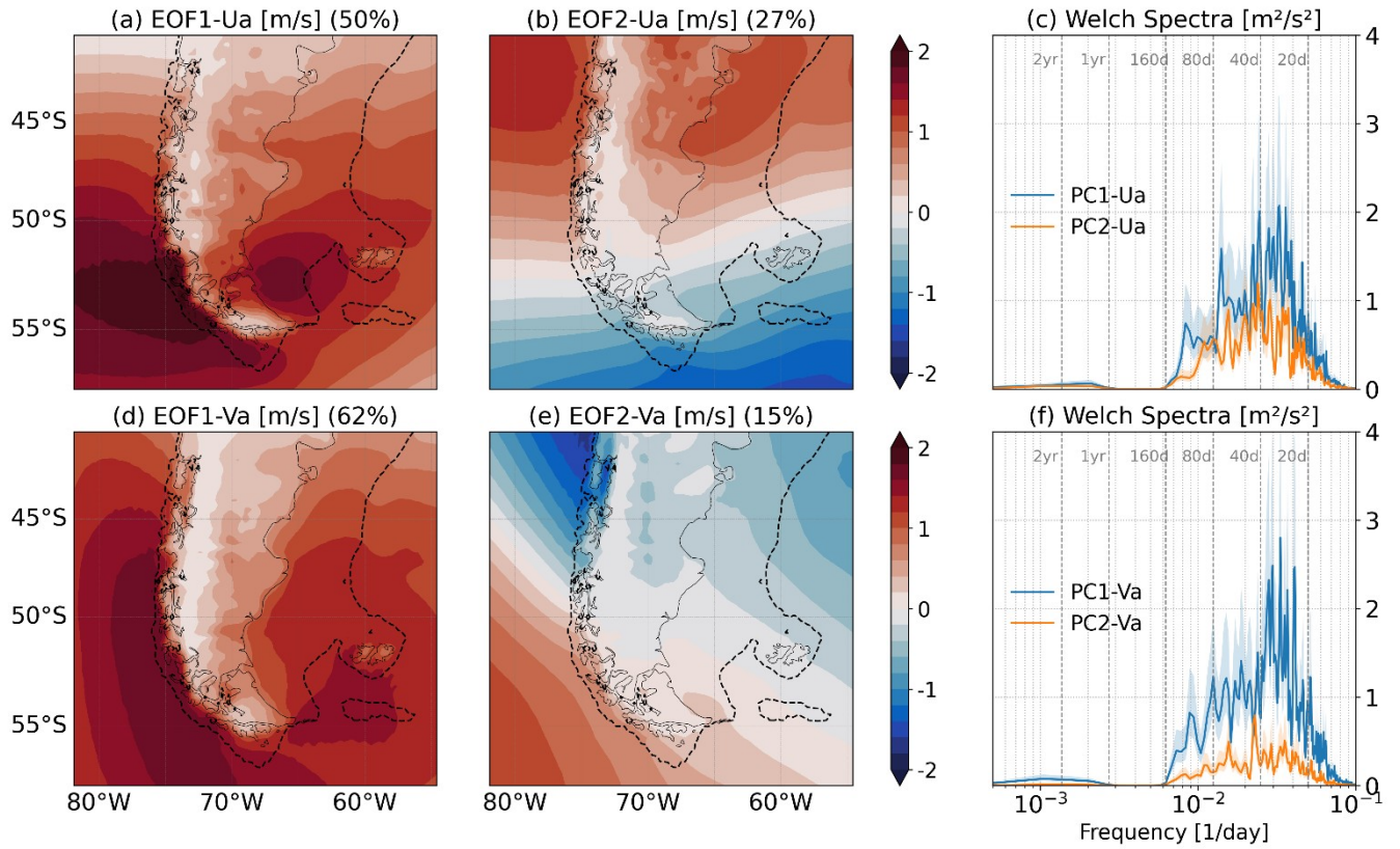
Figure 5: EOF patterns of zonal (Ua) and meridional (Va) wind anomalies. Panels a and b show EOF1 and EOF2 of zonal wind anomalies, while panels d and e show EOF1 and EOF2 of meridional wind anomalies. Contour intervals are 0.2 \text{ m s}^{-1} . The black dashed line on the EOF maps indicates the 200 m isobath. Panels c and f display the power spectra of the corresponding principal component time series for zonal and meridional wind anomalies, respectively, estimated using Welch's method. In the spectral plots, blue and orange curves represent the spectra of the first and second principal components. Spectra are displayed in a variance-preserving form to highlight the distribution of variance across frequency bands.
