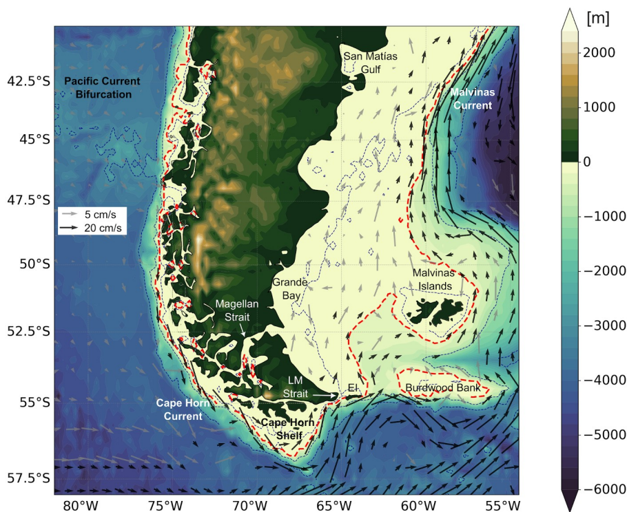
Figure 1: Mean circulation around South America inferred from the Mean Dynamic Topography for the period 1993–2022. Gray arrows indicate velocities lower than 8 cm/s, and black arrows indicate velocities greater than 10 cm/s. Note the different scales. Colours show bathymetry (blue) and land topography (green and brown), in meters. Bathymetry data are from GEBCO Bathymetric Compilation Group (2023). The red dashed line marks the 200 m isobath, close to the continental shelf break. Blue dashed lines indicate the 100, 1000, and 3000 m isobaths. LM: Le Maire Strait. EI: Estados Islands.
