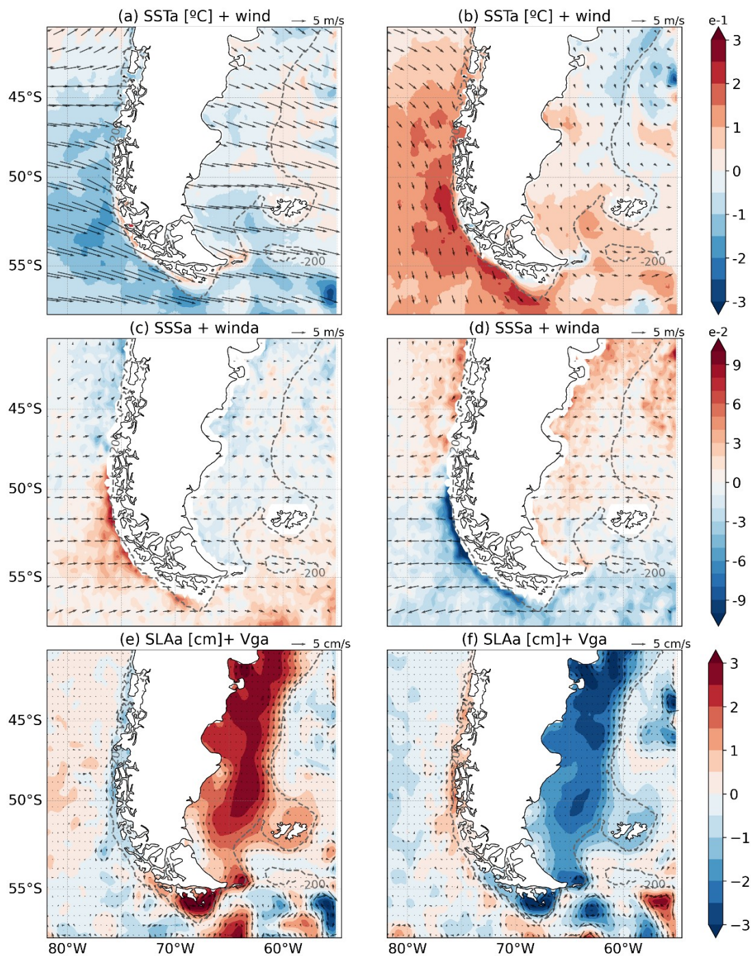
Figure 7: Composites for the positive (increased westerlies) and negative (decreased westerlies) phases of the leading mode of the zonal wind. Panels a, c, and e show SSTa, SSSa, and SLA anomalies for the positive phase, while panels b, d, and f show these anomalies for the negative phase. Black arrows represent wind composites in panels a and b, wind anomalies in panels c and d, and ocean geostrophic velocity anomalies in panels e and f. Gray dashed lines indicate the 200 m isobath.
