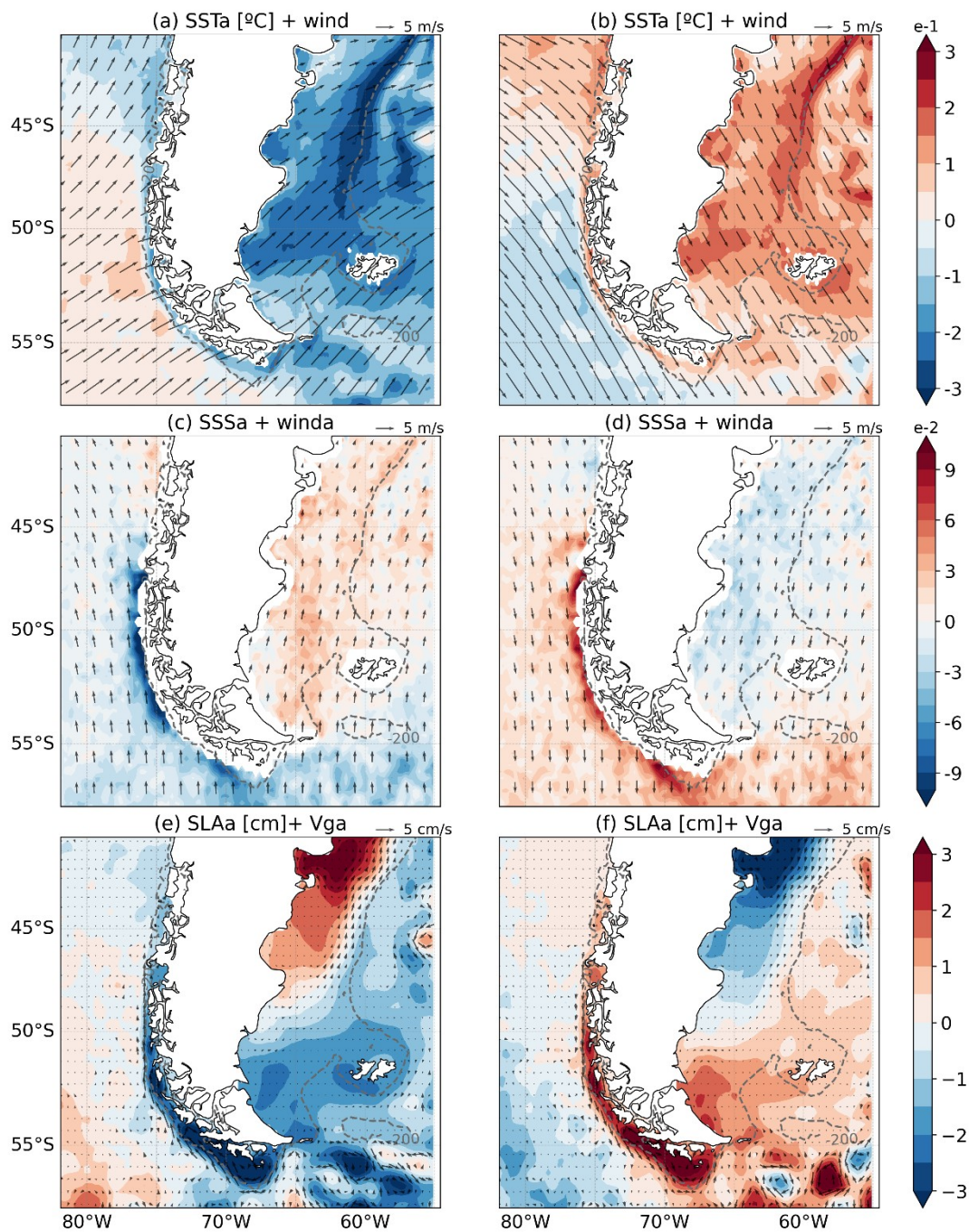
Figure 6: Composites for the positive (southerly winds) and negative (northerly winds) phases of the leading mode of the meridional wind. Panels a, c, and e show SST, SSS, and SLA anomalies for the positive phase, while panels b, d, and f show these anomalies for the negative phase. Black arrows represent wind composites in panels a and b, wind anomalies in panels c and d, and ocean geostrophic velocity anomalies in panels e and f. Gray dashed lines indicate the 200 m isobath.
