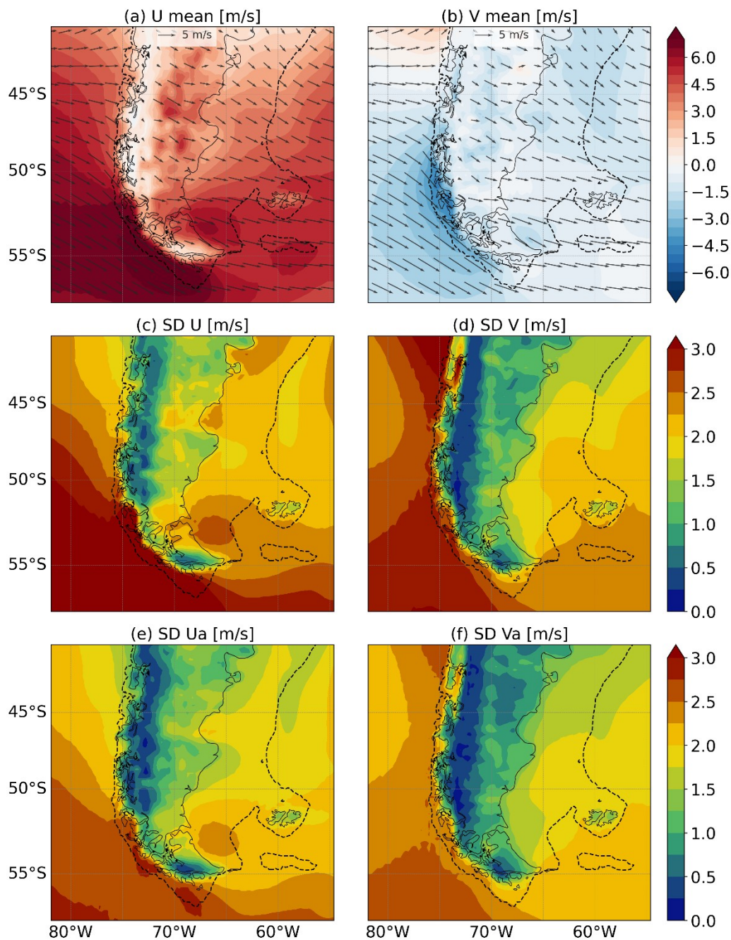
Figure 3: Mean fields of zonal (a, m/s) and meridional wind (b, m/s) components and their standard deviation. Panels c and d show the standard deviation of the low-pass filtered time series with respect to the mean fields, thus including seasonal variability. Panels e and f display the standard deviation of the wind anomalies, after removing the annual signal. The contours are drawn every 0.5 m/s in the mean fields and 0.25 m/s in the standard deviation maps. The black arrows in panels a and b represent the mean wind vectors (scale shown at the top of panels). The black dashed line in all maps indicates the 200 m isobath.
